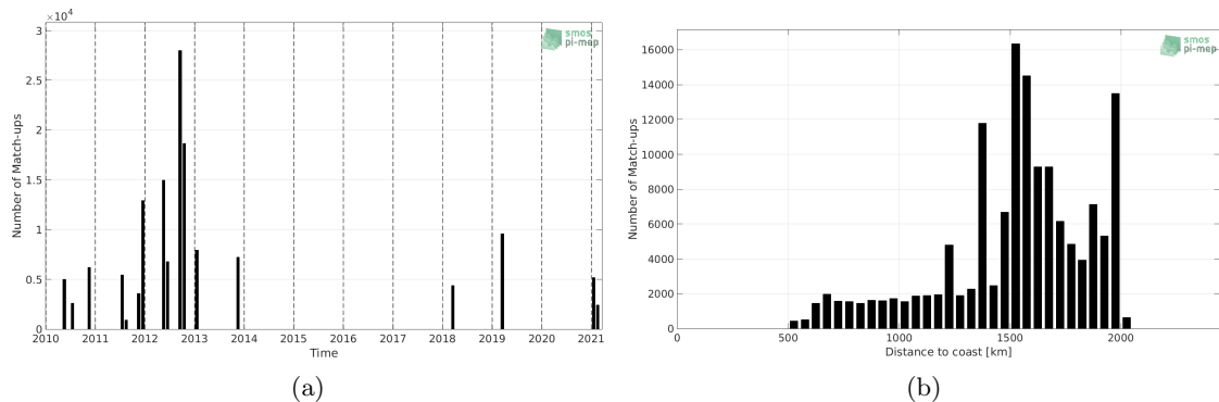
Figure 1: Number of match-ups between TSG (SAMOS) and SMOS SSS L3 v7 - 18 Days (CATDS-CECOS-LOCEAN) SSS as a function of time (a) and as function of the distance to coast (b) over the SPURS 1 Pi-MEP region and for the full satellite product period.
