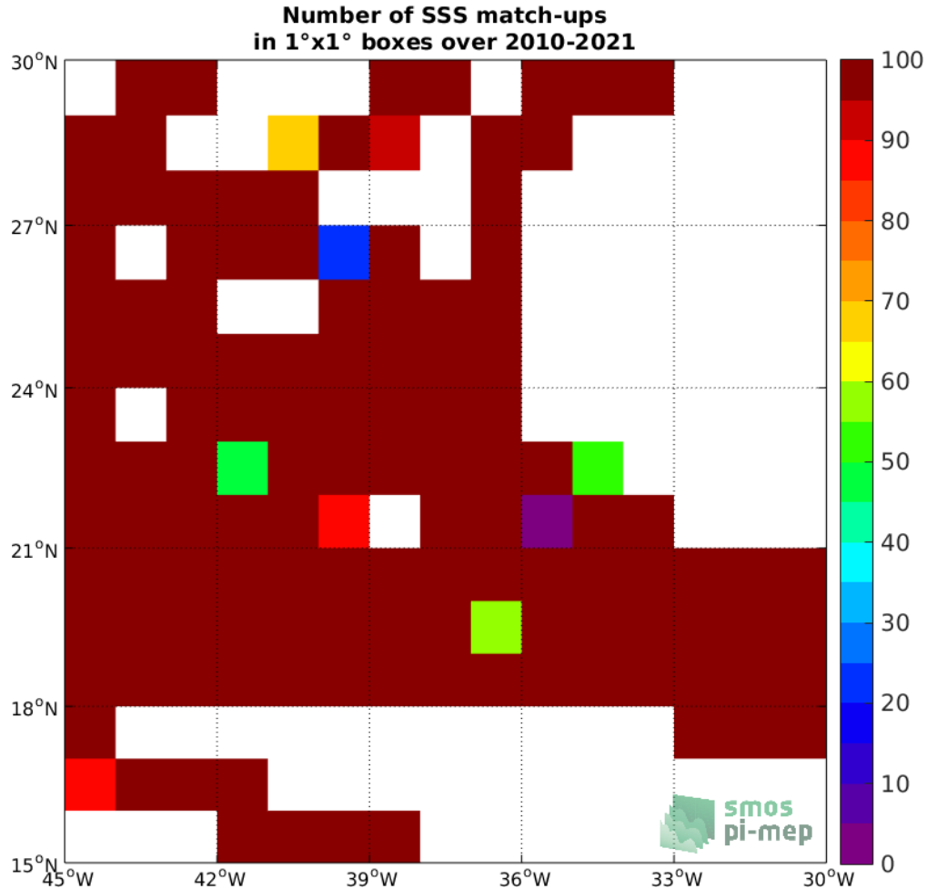
Figure 4: Number of SSS match-ups between TSG (SAMOS) SSS and the SMOS SSS L3 v7 - 18 Days (CATDS-CECOS-LOCEAN) SSS product for the SPURS 1 Pi-MEP region over 1^\circ \times 1^\circ boxes and for the full satellite product period.
