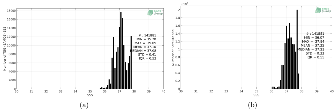
Figure 2: Histograms of SSS from TSG (SAMOS) (a) and SMOS SSS L3 v7 - 18 Days (CATDS-CECOS-LOCEAN) (b) considering all match-up pairs per bins of 0.1 over the SPURS 1 Pi-MEP region and for the full satellite product period.
