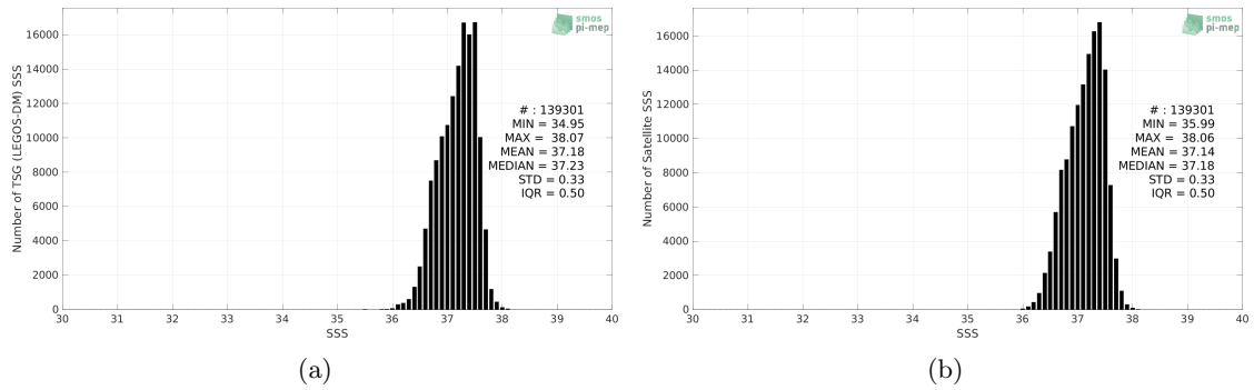
Figure 2: Histograms of SSS from TSG (LEGOS-DM) (a) and SMOS SSS L3 v7 - 18 Days (CATDS-CECOS-LOCEAN) (b) considering all match-up pairs per bins of 0.1 over the SPURS 1 Pi-MEP region and for the full satellite product period.
