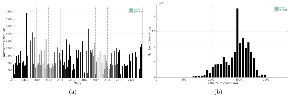
Figure 1: Number of match-ups between TSG (LEGOS-DM) and SMOS SSS L3 v7 - 18 Days (CATDS-CECOS-LOCEAN) SSS as a function of time (a) and as function of the distance to coast (b) over the SPURS 1 Pi-MEP region and for the full satellite product period.
