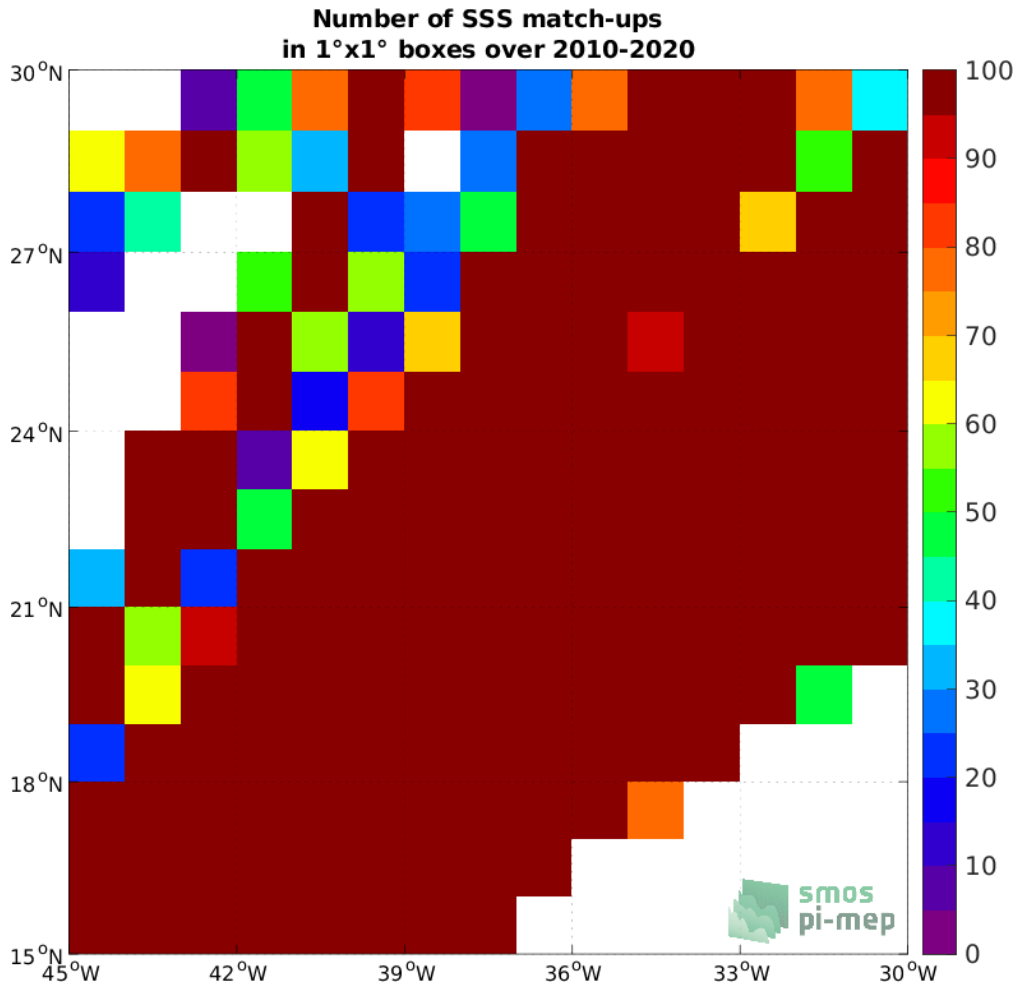
Figure 4: Number of SSS match-ups between TSG (LEGOS-DM) SSS and the SMOS SSS L3 v7 - 18 Days (CATDS-CECOS-LOCEAN) SSS product for the SPURS 1 Pi-MEP region over 1^\circ \times 1^\circ boxes and for the full satellite product period.
