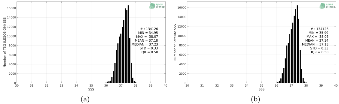
Figure 2: Histograms of SSS from TSG (LEGOS-DM) (a) and SMOS SSS L3 v7 - 18 Days (CATDS-CECOS-LOCEAN) (b) considering all match-up pairs per bins of 0.1 over the SPURS 1 Pi-MEP region and for the full satellite product period.
