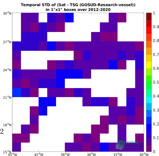
(f) Std( \Delta SSS) (Satellite - TSG (GOSUD-Research-vessel))
