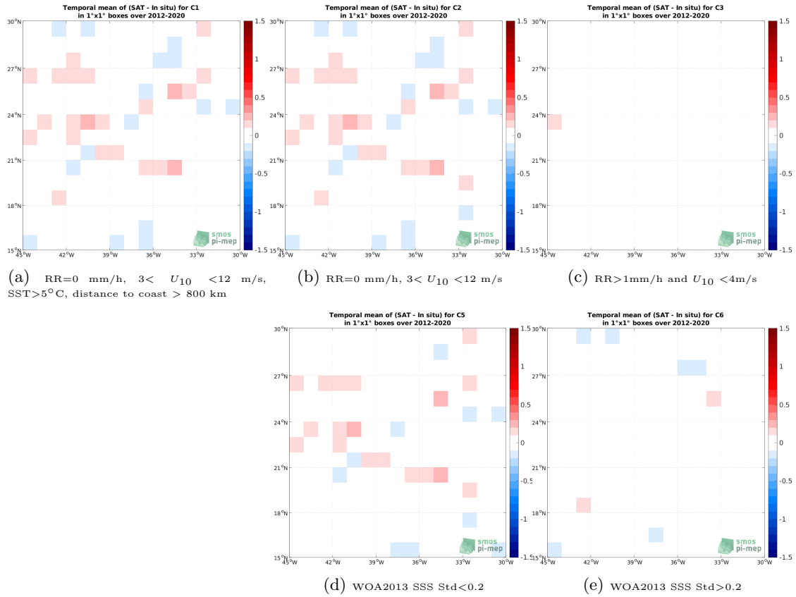
Figure 12: Temporal mean gridded over spatial boxes of size 1^\circ \times 1^\circ of \Delta SSS (SMOS SSS L3 v7 - 18 Days (CATDS-CECOS-LOCEAN) - TSG (GOSUD-Research-vessel)) for 5 different sub-datasets corresponding to: RR=0 mm/h, 3 < U_{10} < 12 m/s, SST>5°C, distance to coast > 800 km (a), RR=0 mm/h, 3 < U_{10} < 12 m/s (b), RR>1mm/h and U_{10} < 4 m/s (c), WOA2013 SSS Std<0.2 (d), WOA2013 SSS Std>0.2 (e).
