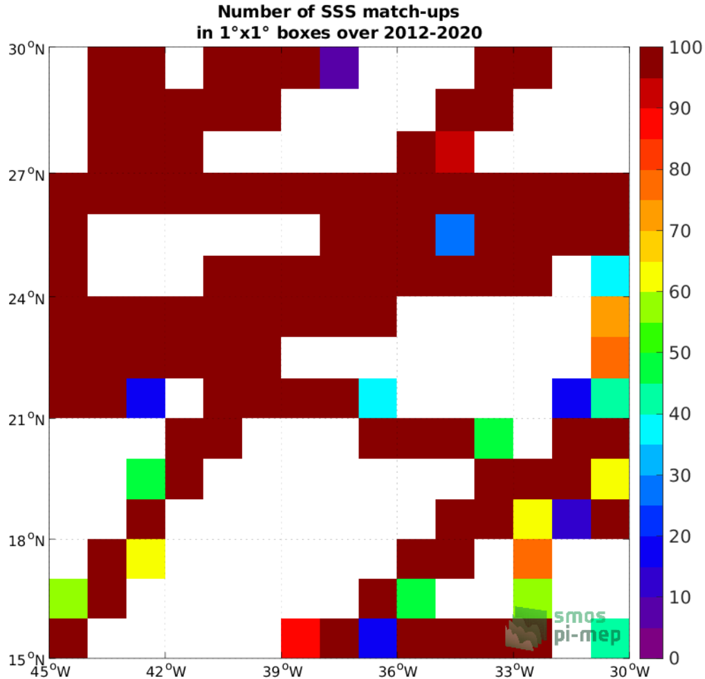
Figure 4: Number of SSS match-ups between TSG (GOSUD-Research-vessel) SSS and the SMOS SSS L3 v7 - 18 Days (CATDS-CECOS-LOCEAN) SSS product for the SPURS 1 Pi-MEP region over 1^\circ \times 1^\circ boxes and for the full satellite product period.
