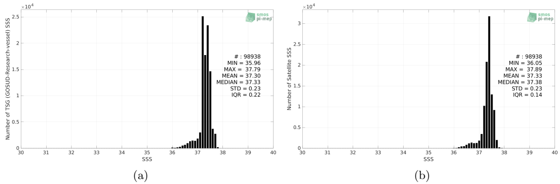
Figure 2: Histograms of SSS from TSG (GOSUD-Research-vessel) (a) and SMOS SSS L3 v7 - 18 Days (CATDS-CECOS-LOCEAN) (b) considering all match-up pairs per bins of 0.1 over the SPURS 1 Pi-MEP region and for the full satellite product period.
