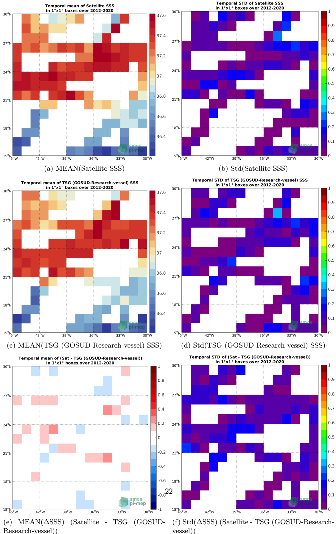
Figure 6: Temporal mean (left) and Std (right) of SSS from SMOS SSS L3 v7 - 18 Days (CATDS-CECOS-LOCEAN) (top), TSG (GOSUD-Research-vessel) (middle), and of \Delta SSS (Satellite - TSG (GOSUD-Research-vessel)). Only match-up pairs are used to generate these maps.
