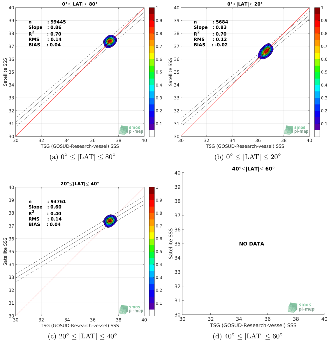
Figure 9: Contour maps of the concentration of SMOS SSS L3 v7 - 18 Days (CATDS-CECOS-LOCEAN) SSS ( y -axis) versus TSG (GOSUD-Research-vessel) SSS ( x -axis) at match-up pairs for different latitude bands. For each plot, the red line shows x=y . The black thin and dashed lines indicate a linear fit through the data cloud and the \pm 95\% confidence levels, respectively. The number match-up pairs n , the slope and R^2 coefficient of the linear fit, the root mean square (RMS) and the mean bias between satellite and in situ data are indicated for each latitude band in each plots.
