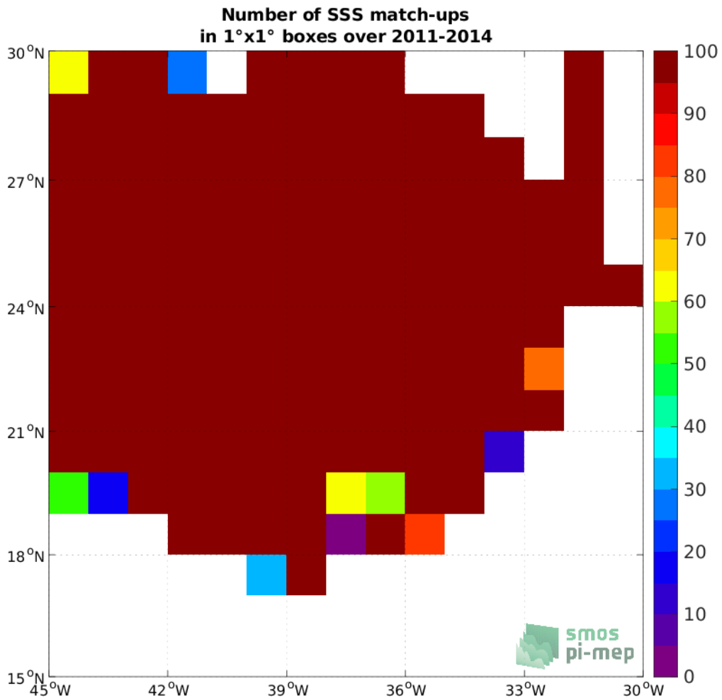
Figure 3: Number of SSS match-ups between Surface drifters SSS and the SMOS SSS L3 v7 - 18 Days (CATDS-CECOS-LOCEAN) SSS product for the SPURS 1 Pi-MEP region over 1°x1° boxes and for the full satellite product period.
