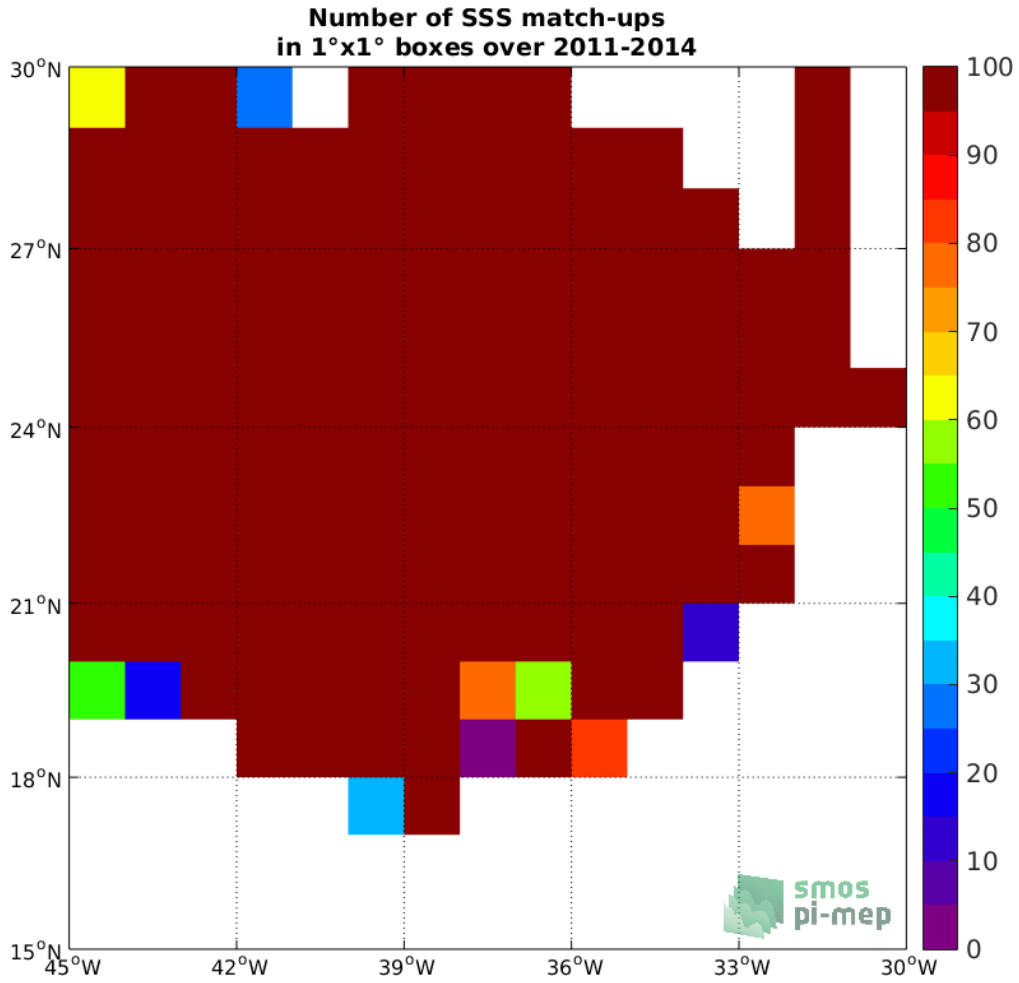
Figure 3: Number of SSS match-ups between Surface drifters SSS and the SMOS SSS L3 v7 - 18 Days (CATDS-CECOS-LOCEAN) SSS product for the SPURS 1 Pi-MEP region over 1^\circ \times 1^\circ boxes and for the full satellite product period.
