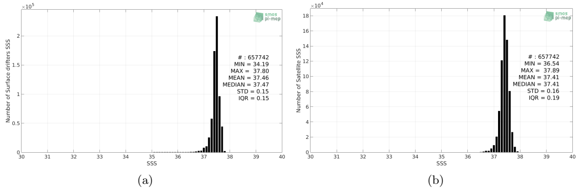
Figure 2: Histograms of SSS from Surface drifters (a) and SMOS SSS L3 v7 - 18 Days (CATDS-CECOS-LOCEAN) (b) considering all match-up pairs per bins of 0.1 over the SPURS 1 Pi-MEP region and for the full satellite product period.
