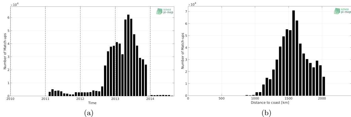
Figure 1: Number of match-ups between Surface drifters and SMOS SSS L3 v7 - 18 Days (CATDS-CECOS-LOCEAN) SSS as a function of time (a) and as function of the distance to coast (b) over the SPURS 1 Pi-MEP region and for the full satellite product period.
