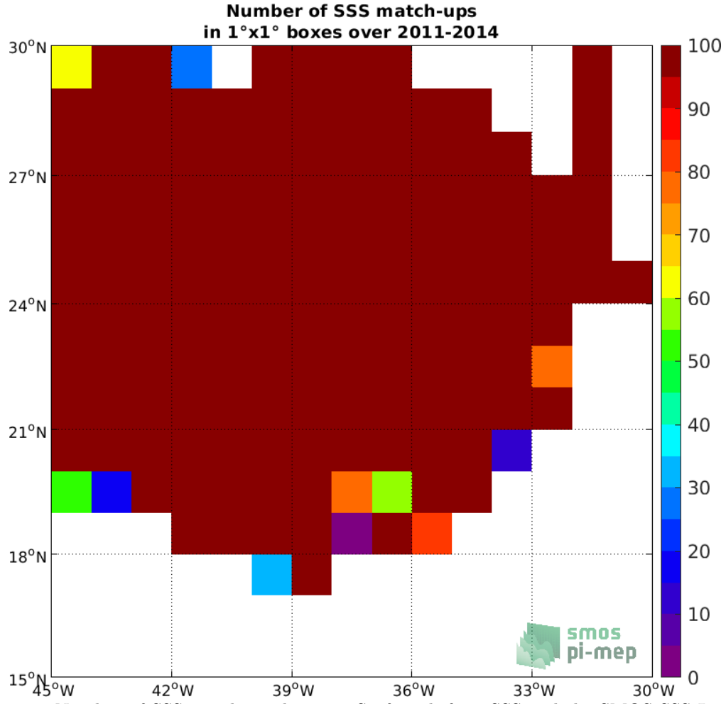
Figure 3: Number of SSS match-ups between Surface drifters SSS and the SMOS SSS L3 v5 - 9 Days (CATDS-CECOS-LOCEAN) SSS product for the SPURS 1 Pi-MEP region over 1°x1° boxes and for the full satellite product period.
