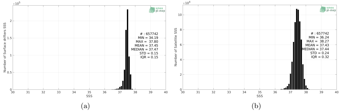
Figure 2: Histograms of SSS from Surface drifters (a) and SMOS SSS L3 v5 - 9 Days (CATDS-CECOS-LOCEAN) (b) considering all match-up pairs per bins of 0.1 over the SPURS 1 Pi-MEP region and for the full satellite product period.
