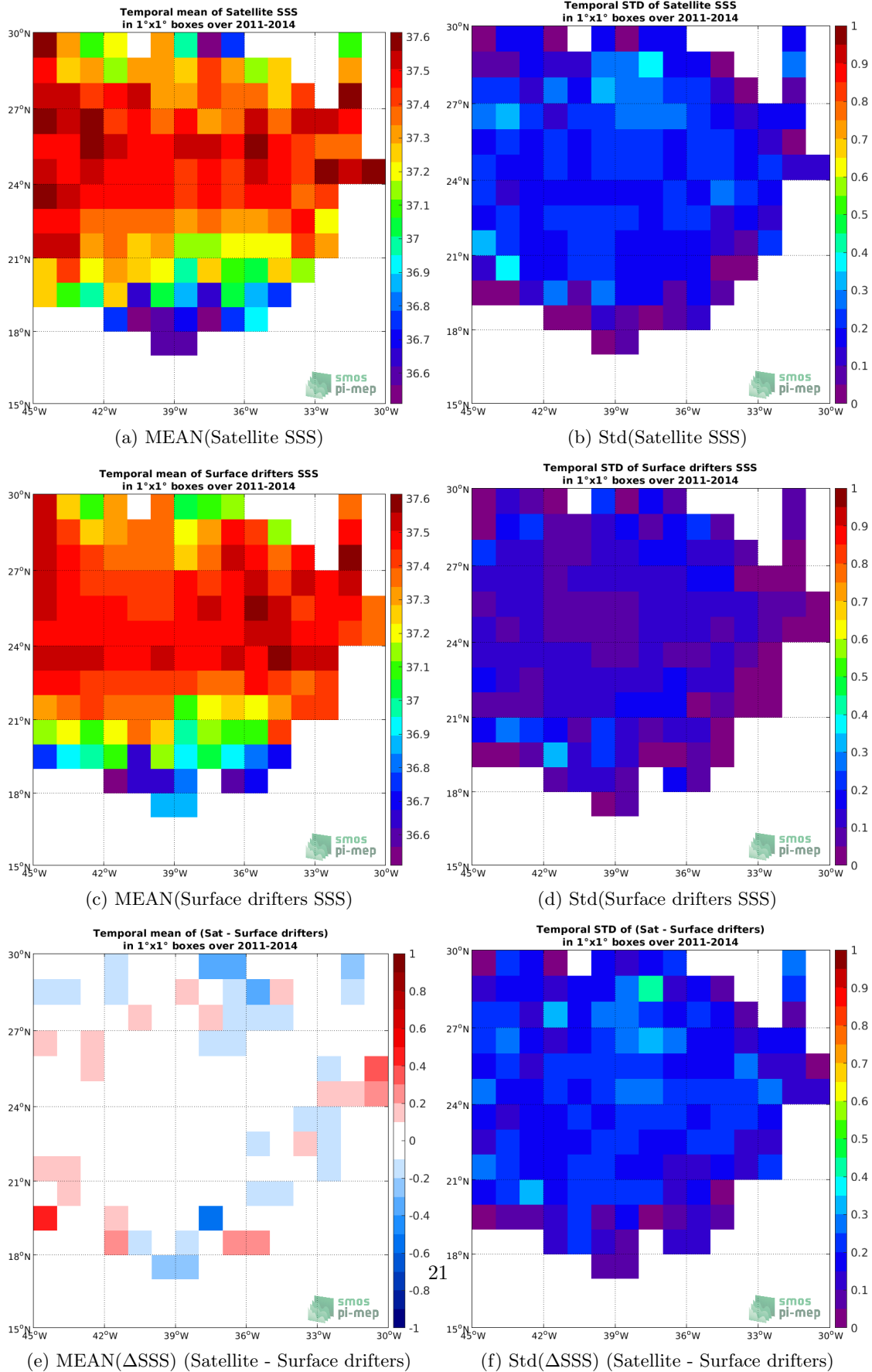
Figure 5: Temporal mean (left) and Std (right) of SSS from SMOS SSS L3 v5 - 9 Days (CATDS-CECOS-LOCEAN) (top), Surface drifters (middle), and of \Delta SSS (Satellite - Surface drifters). Only match-up pairs are used to generate these maps.
