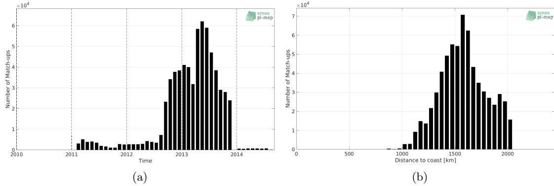
Figure 1: Number of match-ups between Surface drifters and SMOS SSS L3 v5 - 9 Days (CATDS-CECOS-LOCEAN) SSS as a function of time (a) and as function of the distance to coast (b) over the SPURS 1 Pi-MEP region and for the full satellite product period.
