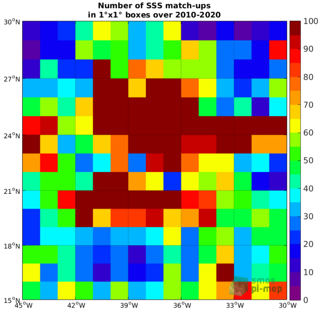
Figure 4: Number of SSS match-ups between Argo SSS and the SMOS SSS L3 v5 - 9 Days (CATDS-CECOS-LOCEAN) SSS product for the SPURS 1 Pi-MEP region over 1°x1° boxes and for the full satellite product period.
