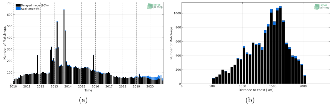
Figure 1: Number of match-ups between Argo and SMOS SSS L3 v5 - 9 Days (CATDS-CECOS-LOCEAN) SSS as a function of time (a) and as function of the distance to coast (b) over the SPURS 1 Pi-MEP region and for the full satellite product period.
