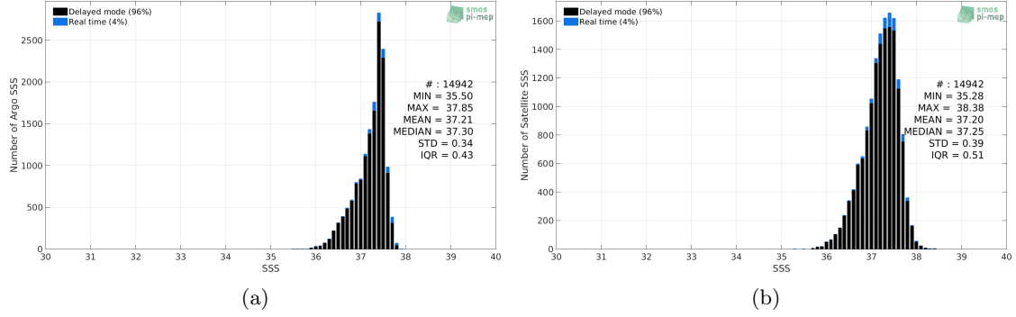
Figure 2: Histograms of SSS from Argo (a) and SMOS SSS L3 v5 - 9 Days (CATDS-CECOS-LOCEAN) (b) considering all match-up pairs per bins of 0.1 over the SPURS 1 Pi-MEP region and for the full satellite product period.
