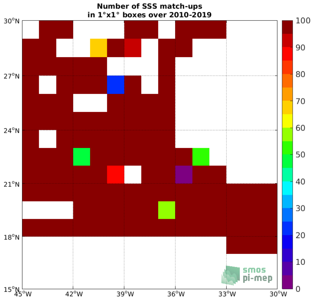
Figure 4: Number of SSS match-ups between TSG (SAMOS) SSS and the SMOS SSS L3 v5 - 18 Days (CATDS-CECOS-LOCEAN) SSS product for the SPURS 1 Pi-MEP region over 1°x1° boxes and for the full satellite product period.
