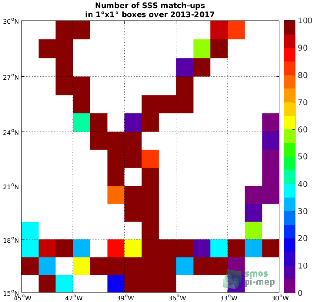
Figure 4: Number of SSS match-ups between TSG (GOSUD-Sailing-ship) SSS and the SMOS SSS L3 v5 - 18 Days (CATDS-CECOS-LOCEAN) SSS product for the SPURS 1 Pi-MEP region over 1°x1° boxes and for the full satellite product period.
