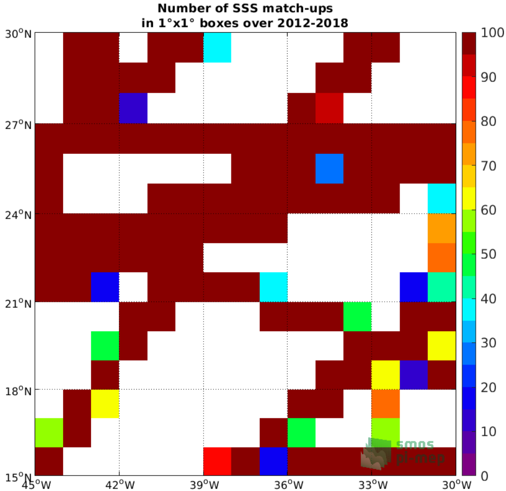
Figure 4: Number of SSS match-ups between TSG (GOSUD-Research-vessel) SSS and the SMOS SSS L3 v5 - 18 Days (CATDS-CECOS-LOCEAN) SSS product for the SPURS 1 Pi-MEP region over 1^\circ \times 1^\circ boxes and for the full satellite product period.
