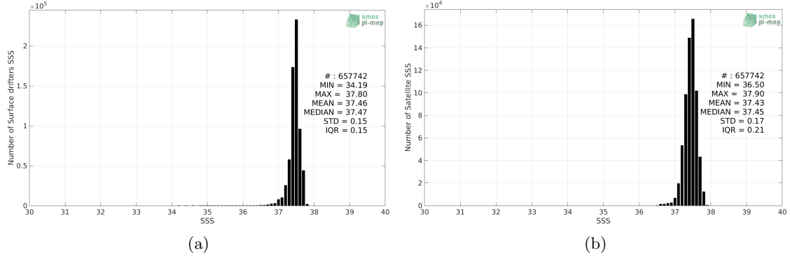
Figure 2: Histograms of SSS from Surface drifters (a) and SMOS SSS L3 v5 - 18 Days (CATDS-CECOS-LOCEAN) (b) considering all match-up pairs per bins of 0.1 over the SPURS 1 Pi-MEP region and for the full satellite product period.
