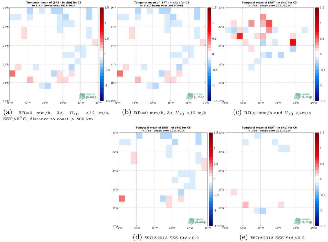
Figure 11: Temporal mean gridded over spatial boxes of size 1^{\circ}\times 1^{\circ} of \Delta\text{SSS} (SMOS SSS L3 v5 - 18 Days (CATDS-CECOS-LOCEAN) - Surface drifters) for 5 different subdatasets corresponding to: RR=0 mm/h, 3 < U_{10} < 12 m/s, SST >5^{\circ}\text{C} , distance to coast > 800 km (a), RR=0 mm/h, 3 < U_{10} < 12 m/s (b), RR >1 mm/h and U_{10} < 4 m/s (c), WOA2013 SSS Std <0.2 (d), WOA2013 SSS Std >0.2 (e).
