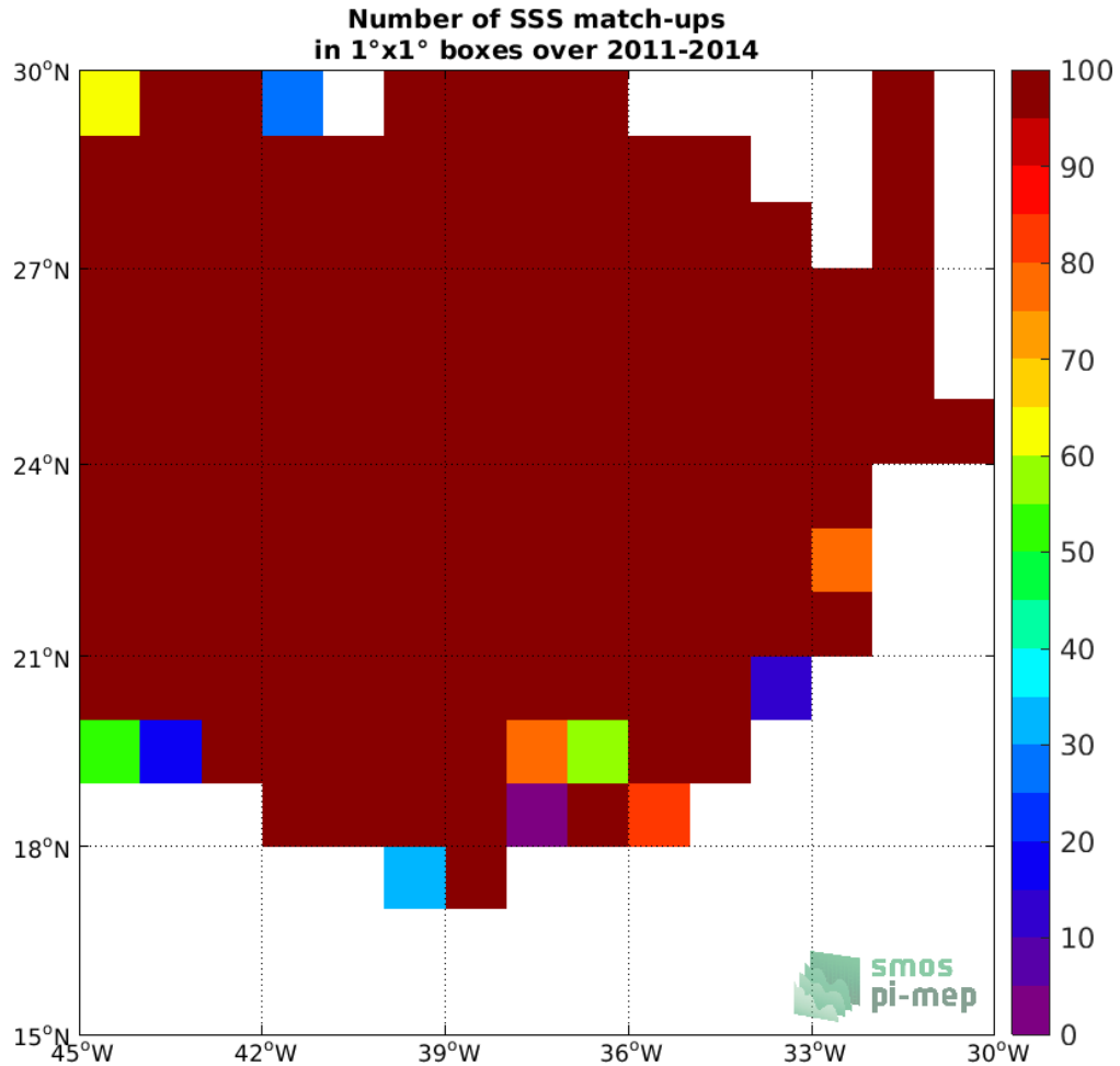
Figure 3: Number of SSS match-ups between Surface drifters SSS and the SMOS SSS L3 v5 - 18 Days (CATDS-CECOS-LOCEAN) SSS product for the SPURS 1 Pi-MEP region over 1°x1° boxes and for the full satellite product period.
