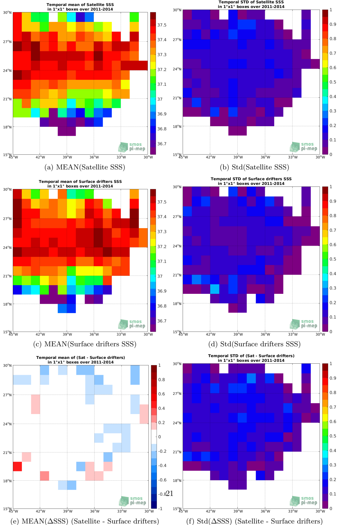
Figure 5: Temporal mean (left) and Std (right) of SSS from SMOS SSS L3 v5 - 18 Days (CATDS-CECOS-LOCEAN) (top), Surface drifters (middle), and of \Delta SSS (Satellite - Surface drifters). Only match-up pairs are used to generate these maps.
