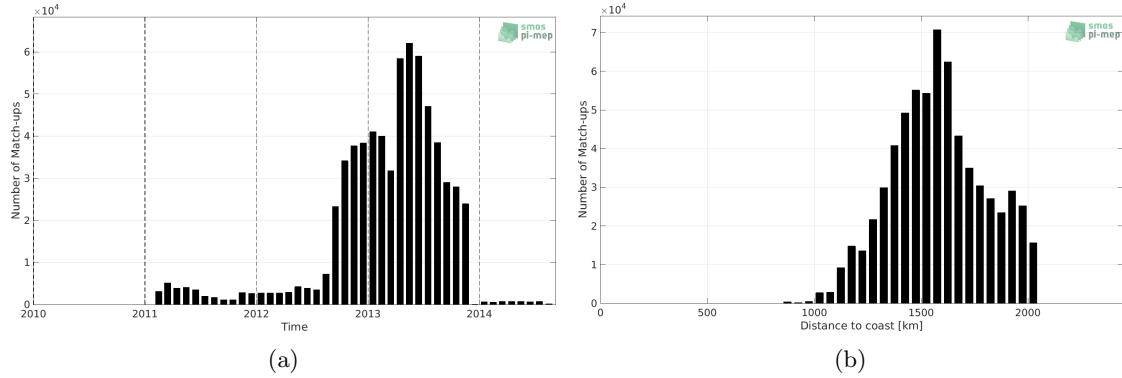
Figure 1: Number of match-ups between Surface drifters and SMOS SSS L3 v5 - 18 Days (CATDS-CECOS-LOCEAN) SSS as a function of time (a) and as function of the distance to coast (b) over the SPURS 1 Pi-MEP region and for the full satellite product period.
