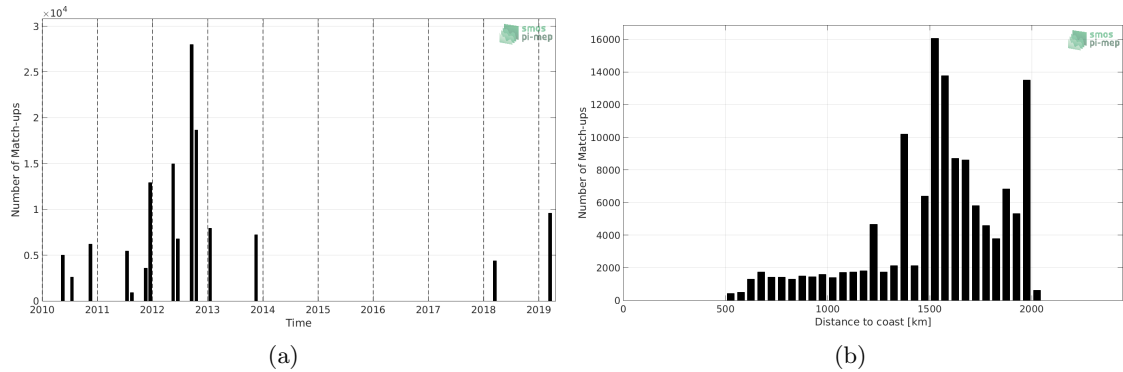
Figure 1: Number of match-ups between TSG (SAMOS) and SMOS SSS L3 v4 - 9 Days (CATDS-CECOS-LOCEAN) SSS as a function of time (a) and as function of the distance to coast (b) over the SPURS 1 Pi-MEP region and for the full satellite product period.
