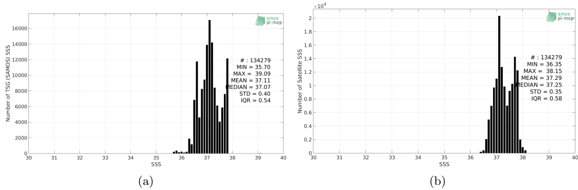
Figure 2: Histograms of SSS from TSG (SAMOS) (a) and SMOS SSS L3 v4 - 9 Days (CATDS-CECOS-LOCEAN) (b) considering all match-up pairs per bins of 0.1 over the SPURS 1 Pi-MEP region and for the full satellite product period.
