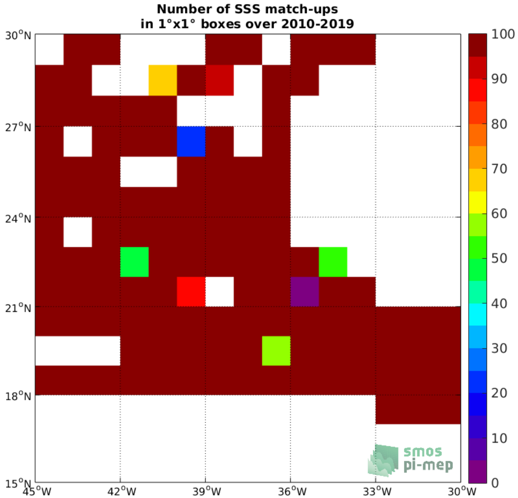
Figure 4: Number of SSS match-ups between TSG (SAMOS) SSS and the SMOS SSS L3 v4 - 9 Days (CATDS-CECOS-LOCEAN) SSS product for the SPURS 1 Pi-MEP region over 1°x1° boxes and for the full satellite product period.
