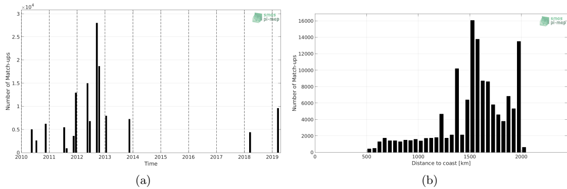
Figure 1: Number of match-ups between TSG-SAMOS and SMOS-L3-CATDS-CECOS-LOCEAN-V4-9DAYS-25KM SSS as a function of time (a) and as function of the distance to coast (b) over the SPURS 1 Pi-MEP region and for the full satellite product period.
