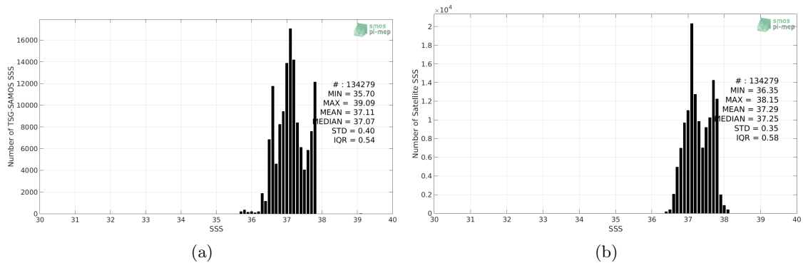
Figure 2: Histograms of SSS from TSG-SAMOS (a) and SMOS-L3-CATDS-CECOS-LOCEAN-V4-9DAYS-25KM (b) considering all match-up pairs per bins of 0.1 over the SPURS 1 Pi-MEP region and for the full satellite product period.
