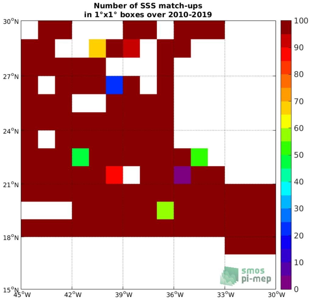
Figure 4: Number of SSS match-ups between TSG-SAMOS SSS and the SMOS-L3-CATDS-CECOS-LOCEAN-V4-9DAYS-25KM SSS product for the SPURS 1 Pi-MEP region over 1°x1° boxes and for the full satellite product period.
