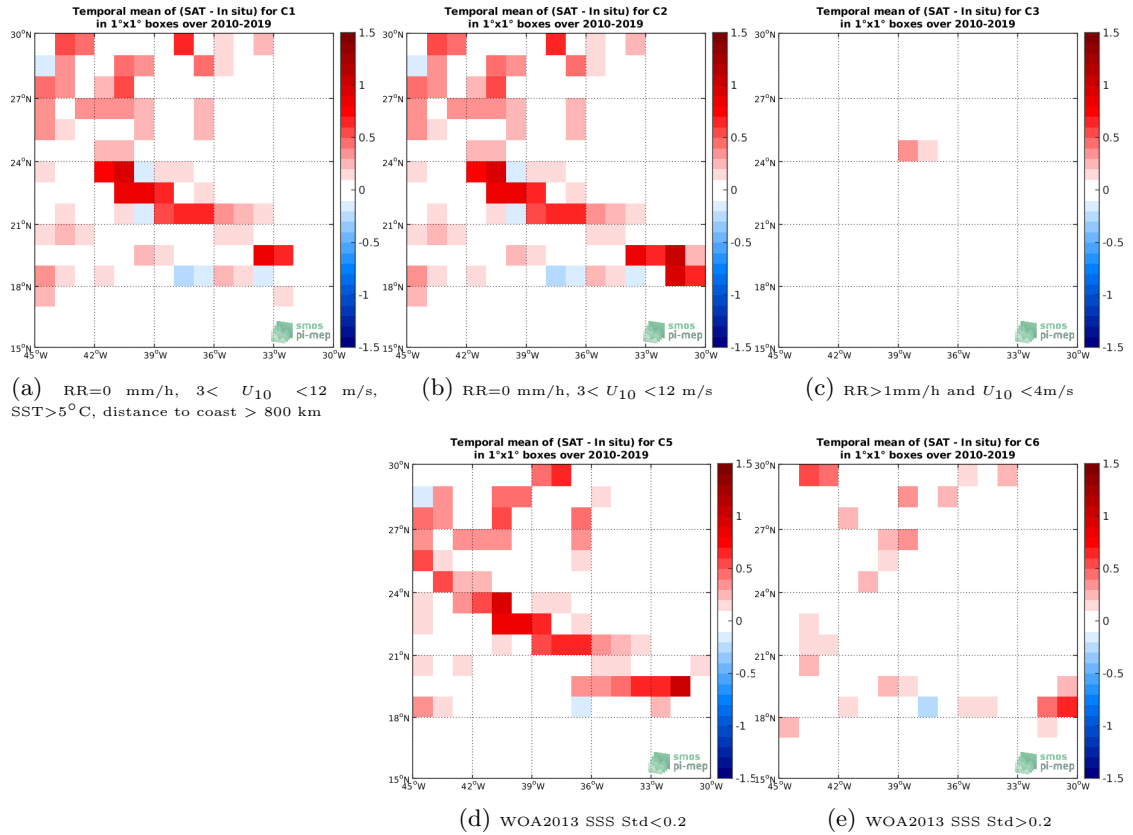
Figure 12: Temporal mean gridded over spatial boxes of size 1^\circ \times 1^\circ of \Delta SSS (SMOS-L3-CATDS-CECOS-LOCEAN-V4-9DAYS-25KM - TSG-SAMOS) for 5 different subdatasets corresponding to:RR=0 mm/h, 3 < U_{10} < 12 m/s, SST >5^\circ C, distance to coast > 800 km (a), RR=0 mm/h, 3 < U_{10} < 12 m/s (b), RR >1 mm/h and U_{10} < 4 m/s (c), WOA2013 SSS Std <0.2 (d), WOA2013 SSS Std >0.2 (e).
