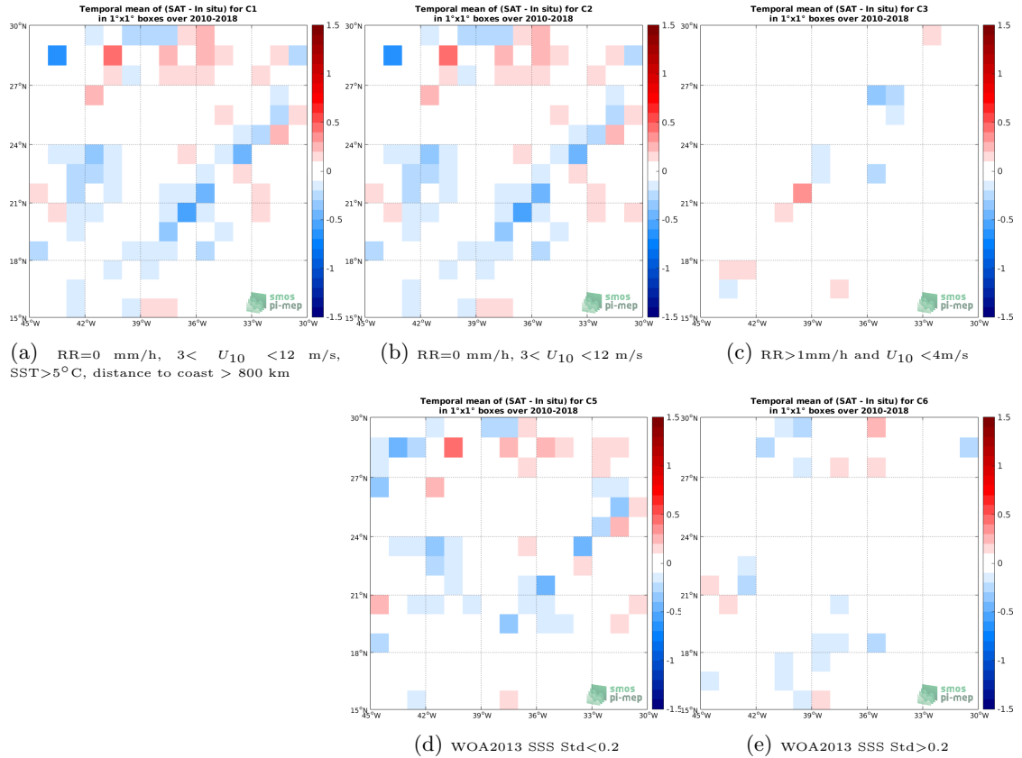
Figure 12: Temporal mean gridded over spatial boxes of size 1^{\circ}\times 1^{\circ} of \Delta\text{SSS} (SMOS-L3-CATDS-CECOS-LOCEAN-V4-9DAYS-25KM - TSG-LEGOS-DM) for 5 different subdatasets corresponding to:RR=0 mm/h, 3 < U_{10} < 12 m/s, SST >5^{\circ}\text{C} , distance to coast > 800 km (a), RR=0 mm/h, 3 < U_{10} < 12 m/s (b), RR >1 mm/h and U_{10} < 4 m/s (c), WOA2013 SSS Std <0.2 (d), WOA2013 SSS Std >0.2 (e).
