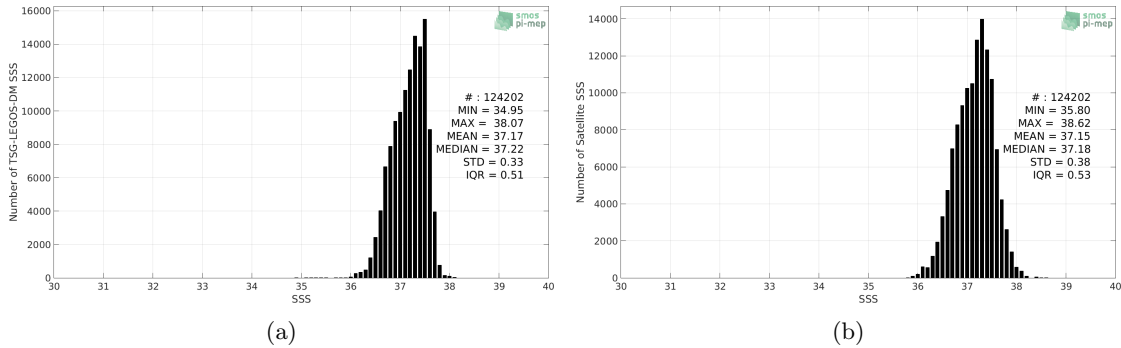
Figure 2: Histograms of SSS from TSG-LEGOS-DM (a) and SMOS-L3-CATDS-CECOS-LOCEAN-V4-9DAYS-25KM (b) considering all match-up pairs per bins of 0.1 over the SPURS 1 Pi-MEP region and for the full satellite product period.
