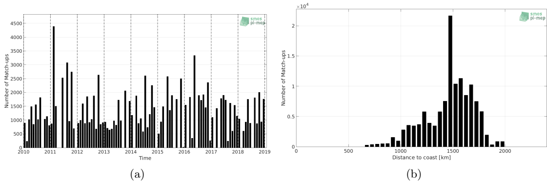
Figure 1: Number of match-ups between TSG-LEGOS-DM and SMOS-L3-CATDS-CECOS-LOCEAN-V4-9DAYS-25KM SSS as a function of time (a) and as function of the distance to coast (b) over the SPURS 1 Pi-MEP region and for the full satellite product period.
