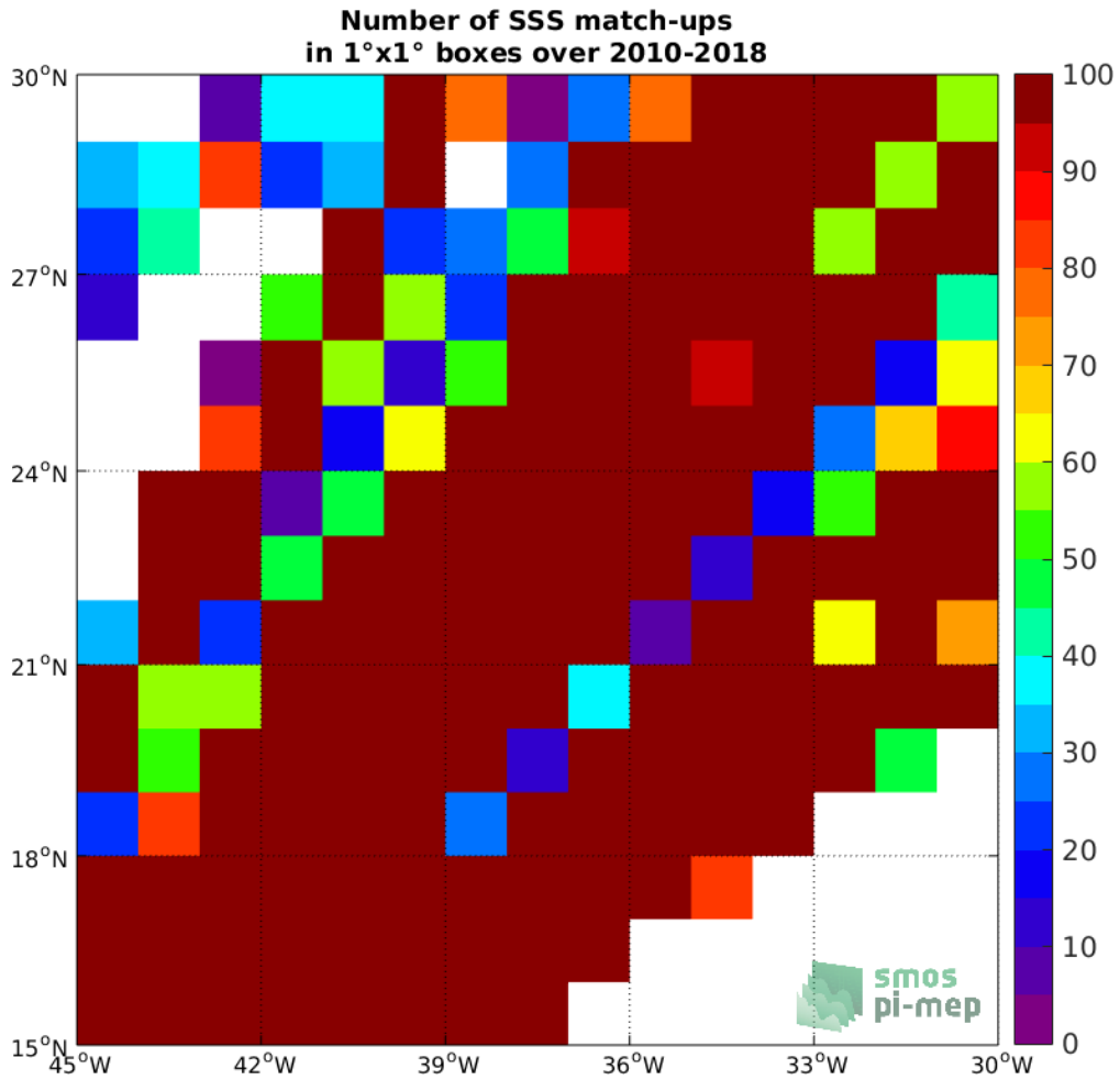
Figure 4: Number of SSS match-ups between TSG-LEGOS-DM SSS and the SMOS-L3-CATDS-CECOS-LOCEAN-V4-9DAYS-25KM SSS product for the SPURS 1 Pi-MEP region over 1°x1° boxes and for the full satellite product period.
