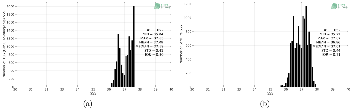
Figure 2: Histograms of SSS from TSG (GOSUD-Sailing-ship) (a) and SMOS SSS L3 v4 - 9 Days (CATDS-CECOS-LOCEAN) (b) considering all match-up pairs per bins of 0.1 over the SPURS 1 Pi-MEP region and for the full satellite product period.
