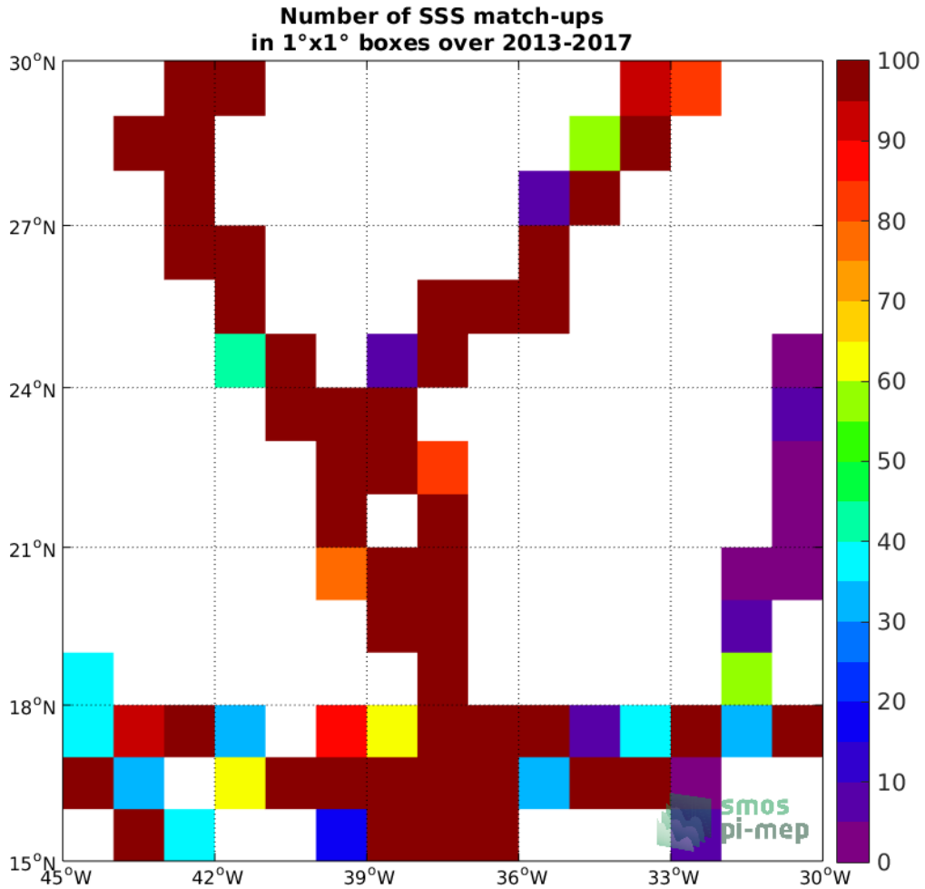
Figure 4: Number of SSS match-ups between TSG (GOSUD-Sailing-ship) SSS and the SMOS SSS L3 v4 - 9 Days (CATDS-CECOS-LOCEAN) SSS product for the SPURS 1 Pi-MEP region over 1°x1° boxes and for the full satellite product period.
