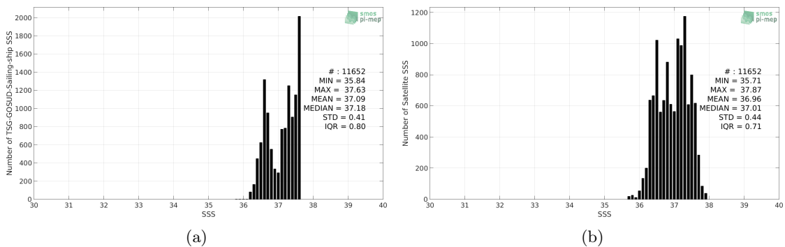
Figure 2: Histograms of SSS from TSG-GOSUD-Sailing-ship (a) and SMOS-L3-CATDS-CECOS-LOCEAN-V4-9DAYS-25KM (b) considering all match-up pairs per bins of 0.1 over the SPURS 1 Pi-MEP region and for the full satellite product period.
