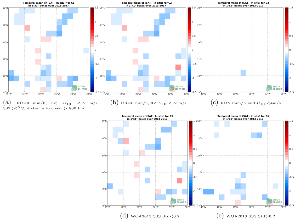
Figure 12: Temporal mean gridded over spatial boxes of size 1^\circ \times 1^\circ of \Delta SSS (SMOS-L3-CATDS-CECOS-LOCEAN-V4-9DAYS-25KM - TSG-GOSUD-Sailing-ship) for 5 different subdatasets corresponding to: RR=0 mm/h, 3 < U_{10} < 12 m/s, SST>5°C, distance to coast > 800 km (a), RR=0 mm/h, 3 < U_{10} < 12 m/s (b), RR>1mm/h and U_{10} < 4 m/s (c), WOA2013 SSS Std<0.2 (d), WOA2013 SSS Std>0.2 (e).
