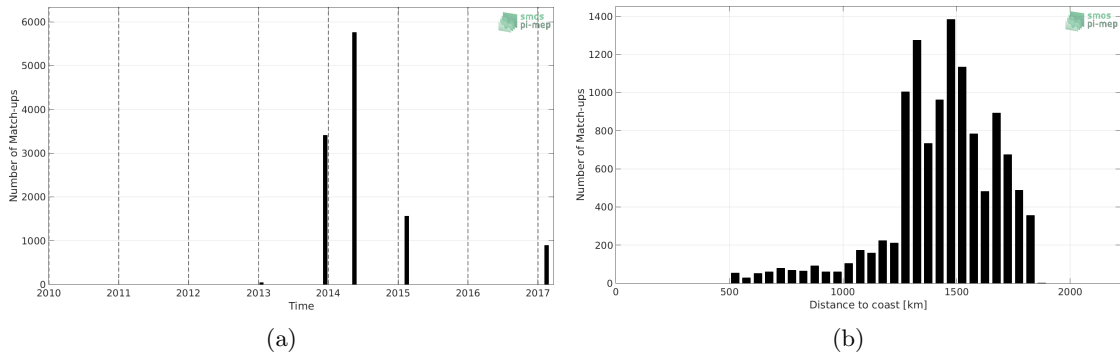
Figure 1: Number of match-ups between TSG-GOSUD-Sailing-ship and SMOS-L3-CATDS-CECOS-LOCEAN-V4-9DAYS-25KM SSS as a function of time (a) and as function of the distance to coast (b) over the SPURS 1 Pi-MEP region and for the full satellite product period.
