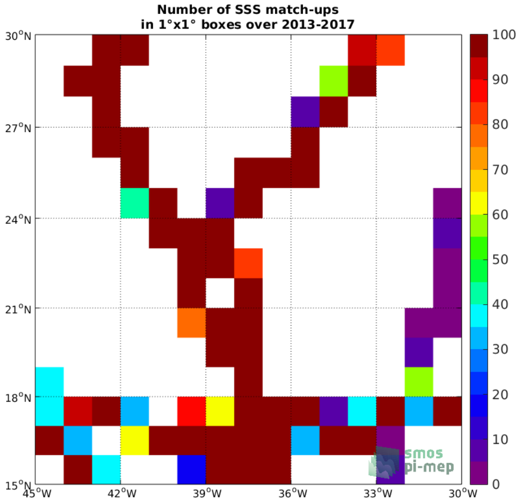
Figure 4: Number of SSS match-ups between TSG-GOSUD-Sailing-ship SSS and the SMOS-L3-CATDS-CECOS-LOCEAN-V4-9DAYS-25KM SSS product for the SPURS 1 Pi-MEP region over 1°x1° boxes and for the full satellite product period.
