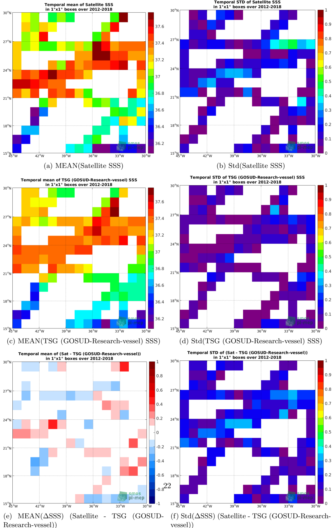
Figure 6: Temporal mean (left) and Std (right) of SSS from SMOS SSS L3 v4 - 9 Days (CATDS-CECOS-LOCEAN) (top), TSG (GOSUD-Research-vessel) (middle), and of \Delta SSS (Satellite - TSG (GOSUD-Research-vessel)). Only match-up pairs are used to generate these maps.
