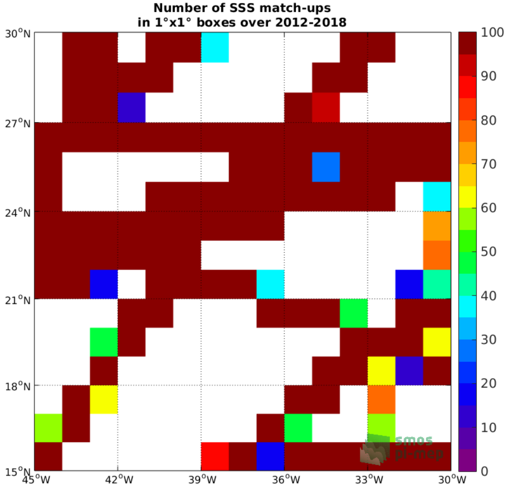
Figure 4: Number of SSS match-ups between TSG (GOSUD-Research-vessel) SSS and the SMOS SSS L3 v4 - 9 Days (CATDS-CECOS-LOCEAN) SSS product for the SPURS 1 Pi-MEP region over 1°x1° boxes and for the full satellite product period.
