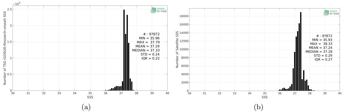
Figure 2: Histograms of SSS from TSG (GOSUD-Research-vessel) (a) and SMOS SSS L3 v4 - 9 Days (CATDS-CECOS-LOCEAN) (b) considering all match-up pairs per bins of 0.1 over the SPURS 1 Pi-MEP region and for the full satellite product period.
