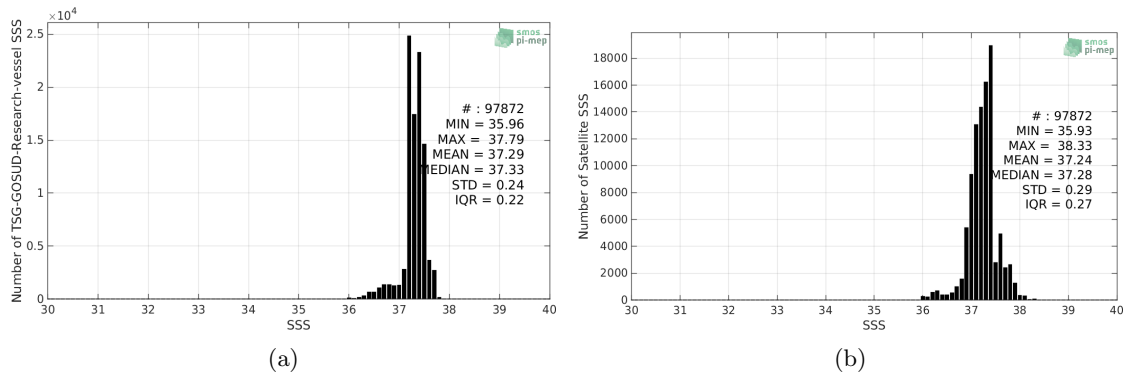
Figure 2: Histograms of SSS from TSG-GOSUD-Research-vessel (a) and SMOS-L3-CATDS-CECOS-LOCEAN-V4-9DAYS-25KM (b) considering all match-up pairs per bins of 0.1 over the SPURS 1 Pi-MEP region and for the full satellite product period.
