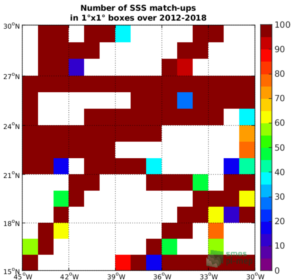
Figure 4: Number of SSS match-ups between TSG-GOSUD-Research-vessel SSS and the SMOS-L3-CATDS-CECOS-LOCEAN-V4-9DAYS-25KM SSS product for the SPURS 1 Pi-MEP region over 1°x1° boxes and for the full satellite product period.
