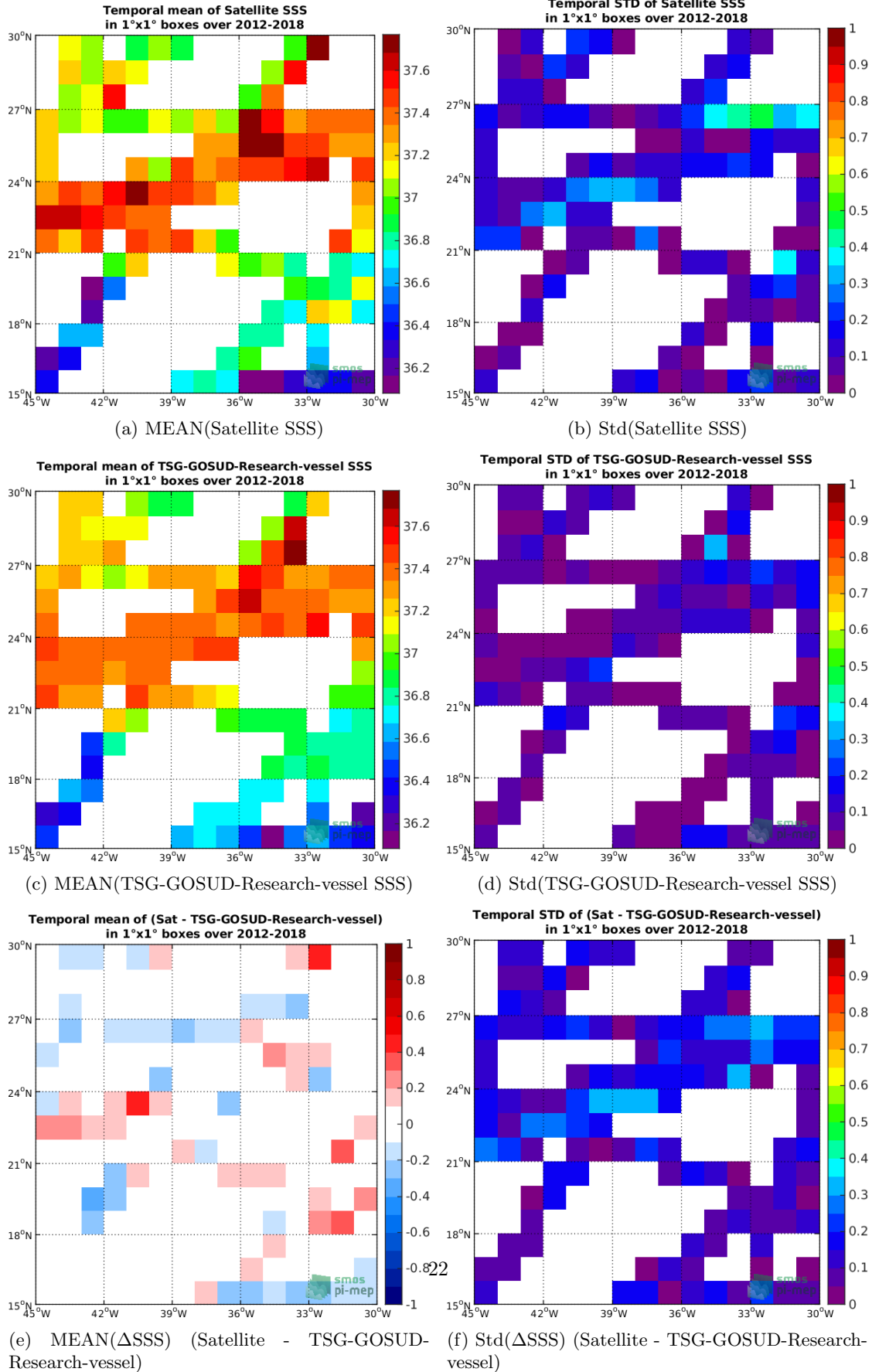
Figure 6: Temporal mean (left) and Std (right) of SSS from SMOS-L3-CATDS-CECOS-LOCEAN-V4-9DAYS-25KM (top), TSG-GOSUD-Research-vessel (middle), and of \Delta SSS (Satellite - TSG-GOSUD-Research-vessel). Only match-up pairs are used to generate these maps.
