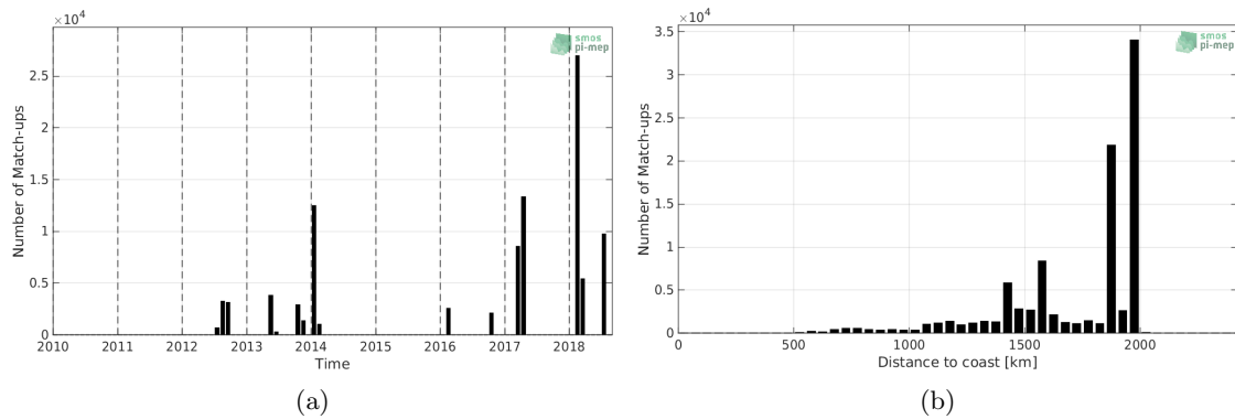
Figure 1: Number of match-ups between TSG-GOSUD-Research-vessel and SMOS-L3-CATDS-CECOS-LOCEAN-V4-9DAYS-25KM SSS as a function of time (a) and as function of the distance to coast (b) over the SPURS 1 Pi-MEP region and for the full satellite product period.
