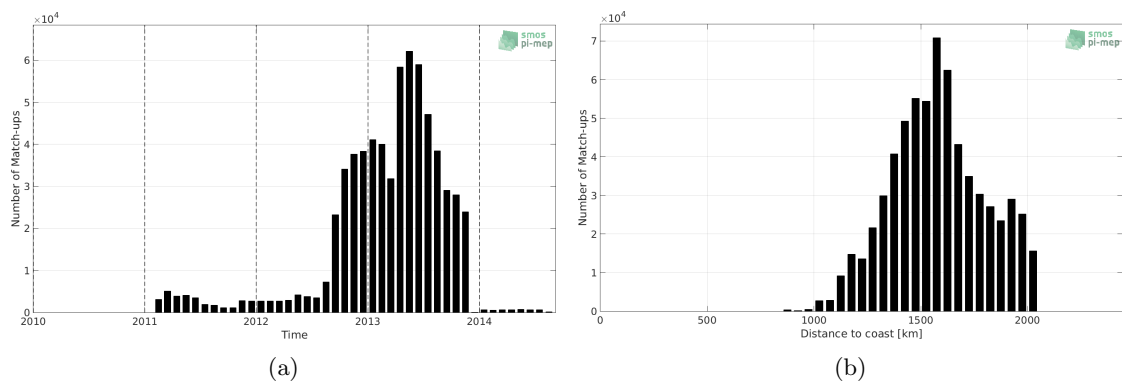
Figure 1: Number of match-ups between Surface drifters and SMOS-L3-CATDS-CECOS-LOCEAN-V4-9DAYS-25KM SSS as a function of time (a) and as function of the distance to coast (b) over the SPURS 1 Pi-MEP region and for the full satellite product period.
