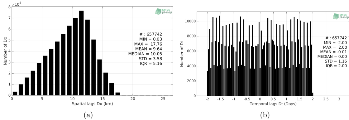
Figure 4: Histograms of the spatial (a) and temporal (b) lags between the time of the Surface drifters measurements and the date of the corresponding SMOS-L3-CATDS-CECOS-LOCEAN-V4-9DAYS-25KM SSS product.
