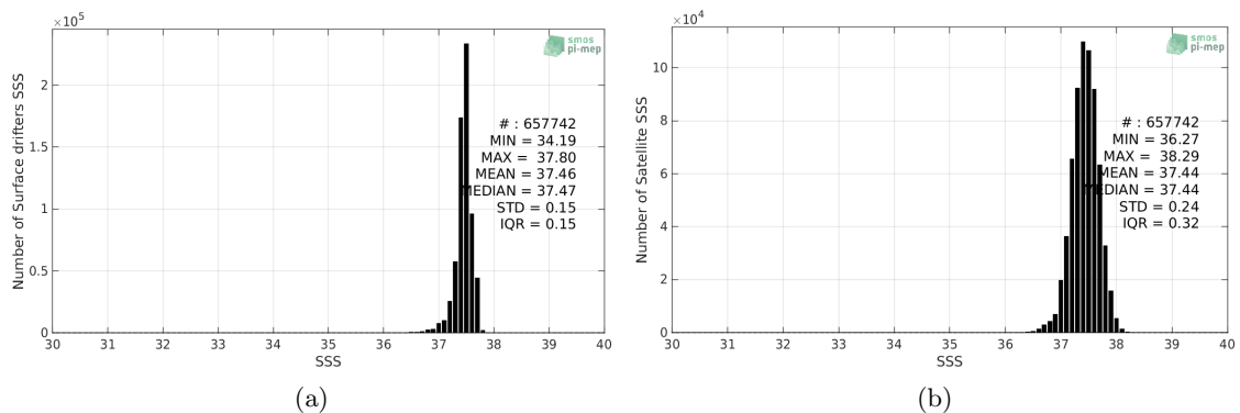
Figure 2: Histograms of SSS from Surface drifters (a) and SMOS-L3-CATDS-CECOS-LOCEAN-V4-9DAYS-25KM (b) considering all match-up pairs per bins of 0.1 over the SPURS 1 Pi-MEP region and for the full satellite product period.
