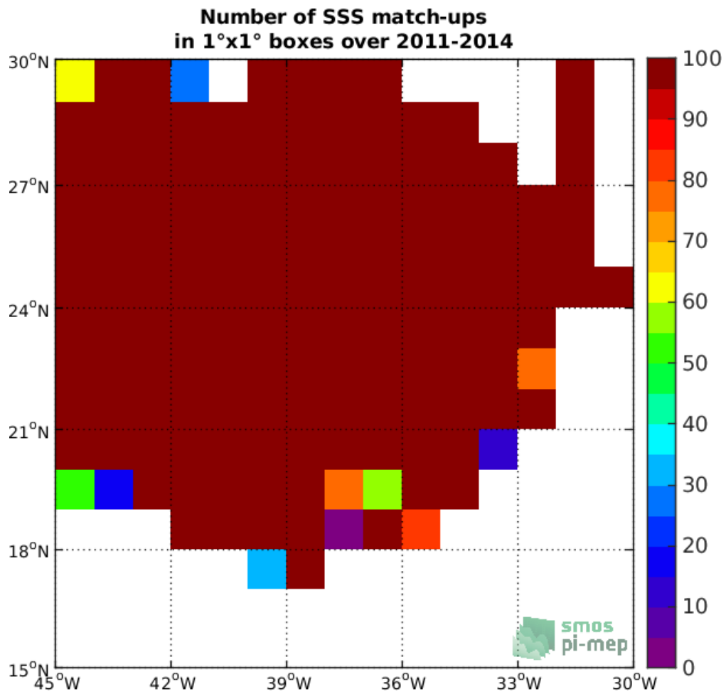
Figure 3: Number of SSS match-ups between Surface drifters SSS and the SMOS-L3-CATDS-CECOS-LOCEAN-V4-9DAYS-25KM SSS product for the SPURS 1 Pi-MEP region over 1°x1° boxes and for the full satellite product period.
