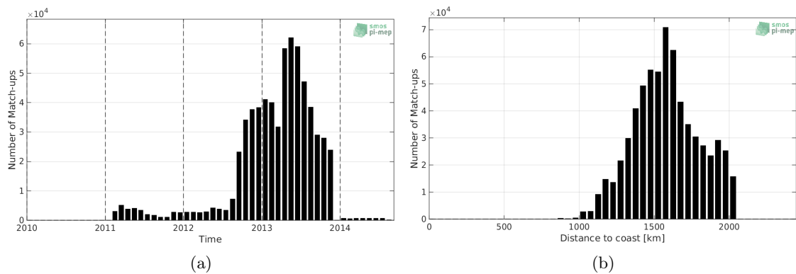
Figure 1: Number of match-ups between Surface drifters and SMOS-L3-CATDS-CECOS-LOCEAN-V4-9DAYS-25KM SSS as a function of time (a) and as function of the distance to coast (b) over the SPURS 1 Pi-MEP region and for the full satellite product period.
