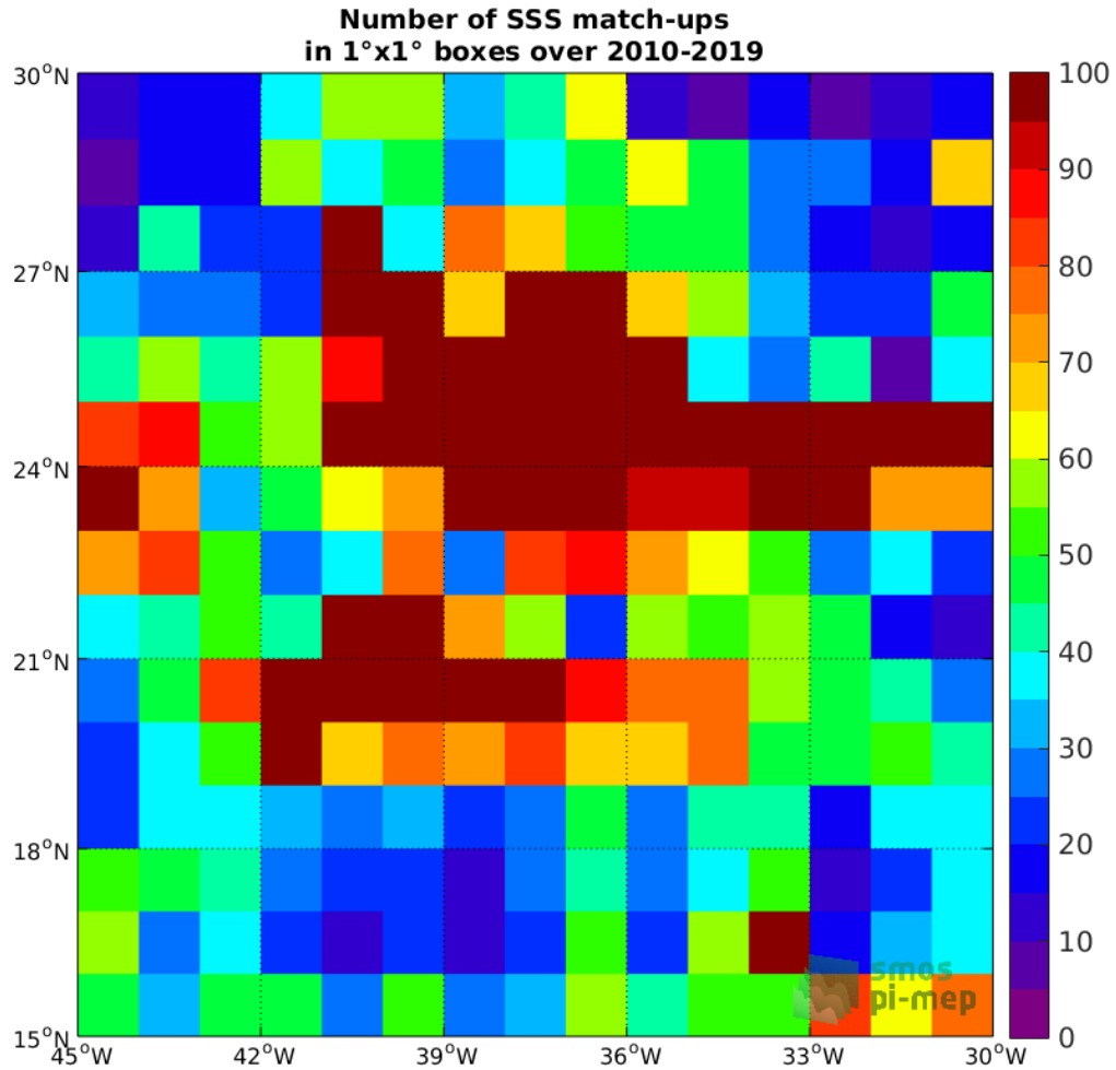
Figure 4: Number of SSS match-ups between Argo SSS and the SMOS SSS L3 v4 - 9 Days (CATDS-CECOS-LOCEAN) SSS product for the SPURS 1 Pi-MEP region over 1°x1° boxes and for the full satellite product period.
