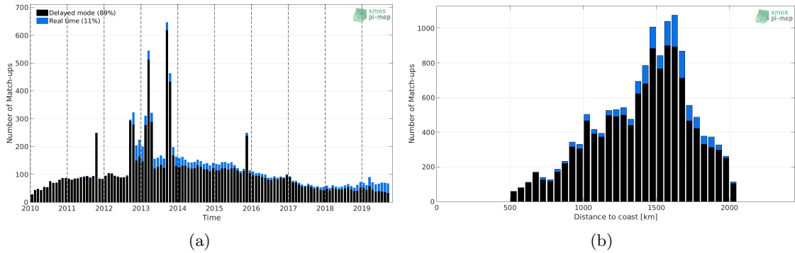
Figure 1: Number of match-ups between Argo and SMOS SSS L3 v4 - 9 Days (CATDS-CECOS-LOCEAN) SSS as a function of time (a) and as function of the distance to coast (b) over the SPURS 1 Pi-MEP region and for the full satellite product period.
