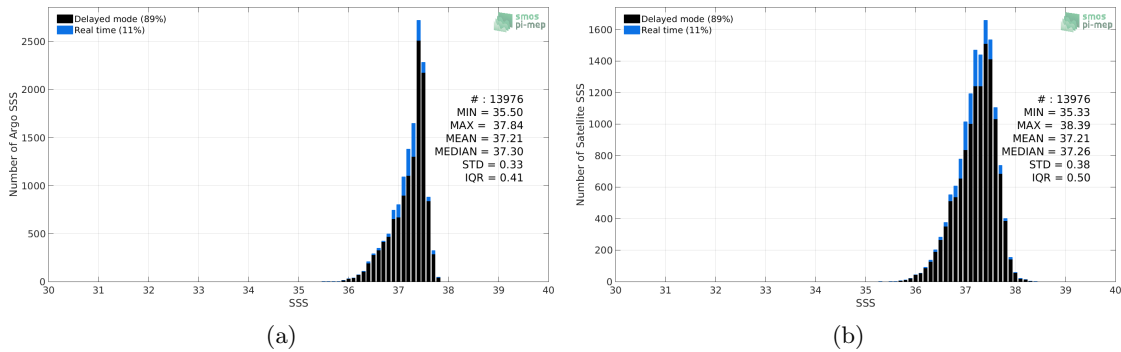
Figure 2: Histograms of SSS from Argo (a) and SMOS SSS L3 v4 - 9 Days (CATDS-CECOS-LOCEAN) (b) considering all match-up pairs per bins of 0.1 over the SPURS 1 Pi-MEP region and for the full satellite product period.
