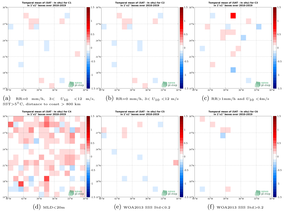
Figure 12: Temporal mean gridded over spatial boxes of size 1^\circ \times 1^\circ of \Delta SSS (SMOS SSS L3 v4 - 9 Days (CATDS-CECOS-LOCEAN) - Argo) for 6 different subdatasets corresponding to:RR=0 mm/h, 3 < U_{10} < 12 m/s, SST >5^\circ C, distance to coast > 800 km (a), RR=0 mm/h, 3 < U_{10} < 12 m/s (b), RR >1 mm/h and U_{10} < 4 m/s (c),MLD <20 m (d),WOA2013 SSS Std <0.2 (e),WOA2013 SSS Std >0.2 (f).
