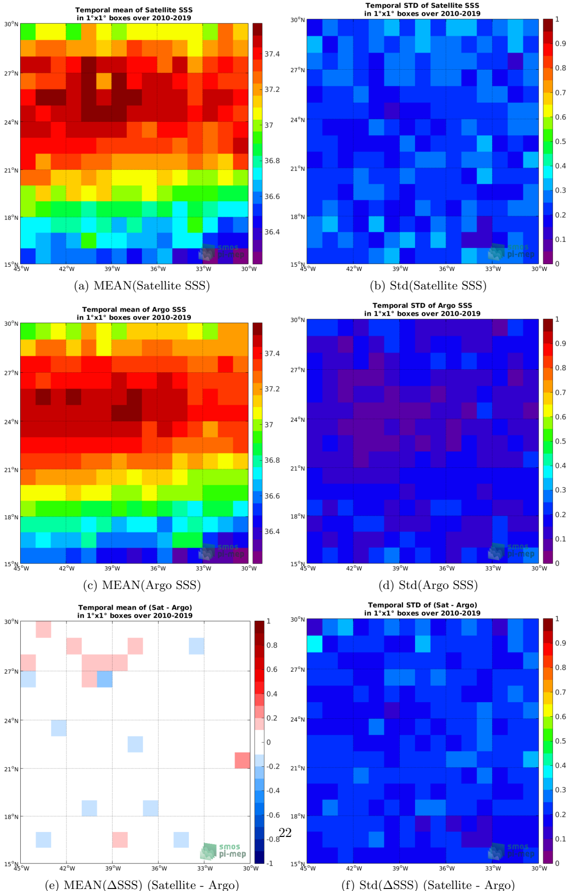
Figure 6: Temporal mean (left) and Std (right) of SSS from SMOS-L3-CATDS-CECOS-LOCEAN-V4-9DAYS-25KM (top), Argo (middle), and of \Delta SSS (Satellite - Argo). Only match-up pairs are used to generate these maps.
