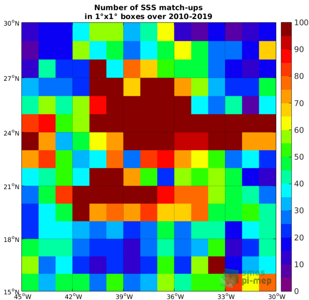
Figure 4: Number of SSS match-ups between Argo SSS and the SMOS-L3-CATDS-CECOS-LOCEAN-V4-9DAYS-25KM SSS product for the SPURS 1 Pi-MEP region over 1°x1° boxes and for the full satellite product period.
