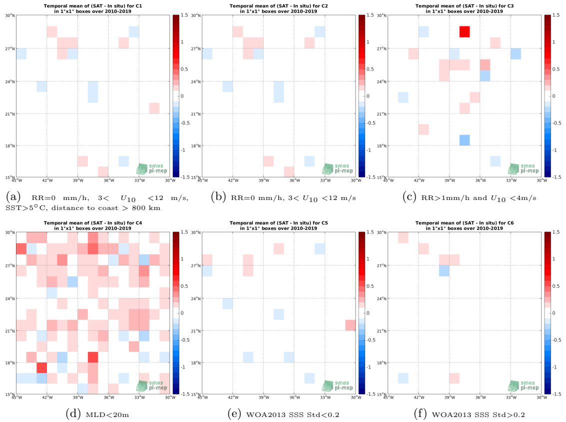
Figure 12: Temporal mean gridded over spatial boxes of size 1^\circ \times 1^\circ of \Delta SSS (SMOS-L3-CATDS-CECOS-LOCEAN-V4-9DAYS-25KM - Argo) for 6 different subdatasets corresponding to:RR=0 mm/h, 3 < U_{10} < 12 m/s, SST >5^\circ C, distance to coast > 800 km (a), RR=0 mm/h, 3 < U_{10} < 12 m/s (b), RR >1 mm/h and U_{10} < 4 m/s (c),MLD <20 m (d),WOA2013 SSS Std <0.2 (e),WOA2013 SSS Std >0.2 (f).
