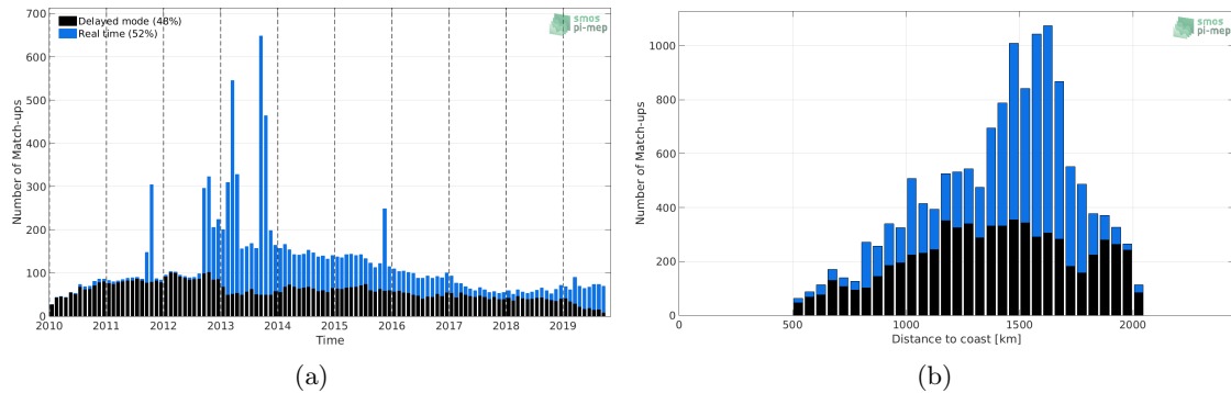
Figure 1: Number of match-ups between Argo and SMOS-L3-CATDS-CECOS-LOCEAN-V4-9DAYS-25KM SSS as a function of time (a) and as function of the distance to coast (b) over the SPURS 1 Pi-MEP region and for the full satellite product period.
