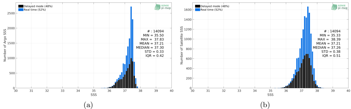
Figure 2: Histograms of SSS from Argo (a) and SMOS-L3-CATDS-CECOS-LOCEAN-V4-9DAYS-25KM (b) considering all match-up pairs per bins of 0.1 over the SPURS 1 Pi-MEP region and for the full satellite product period.
