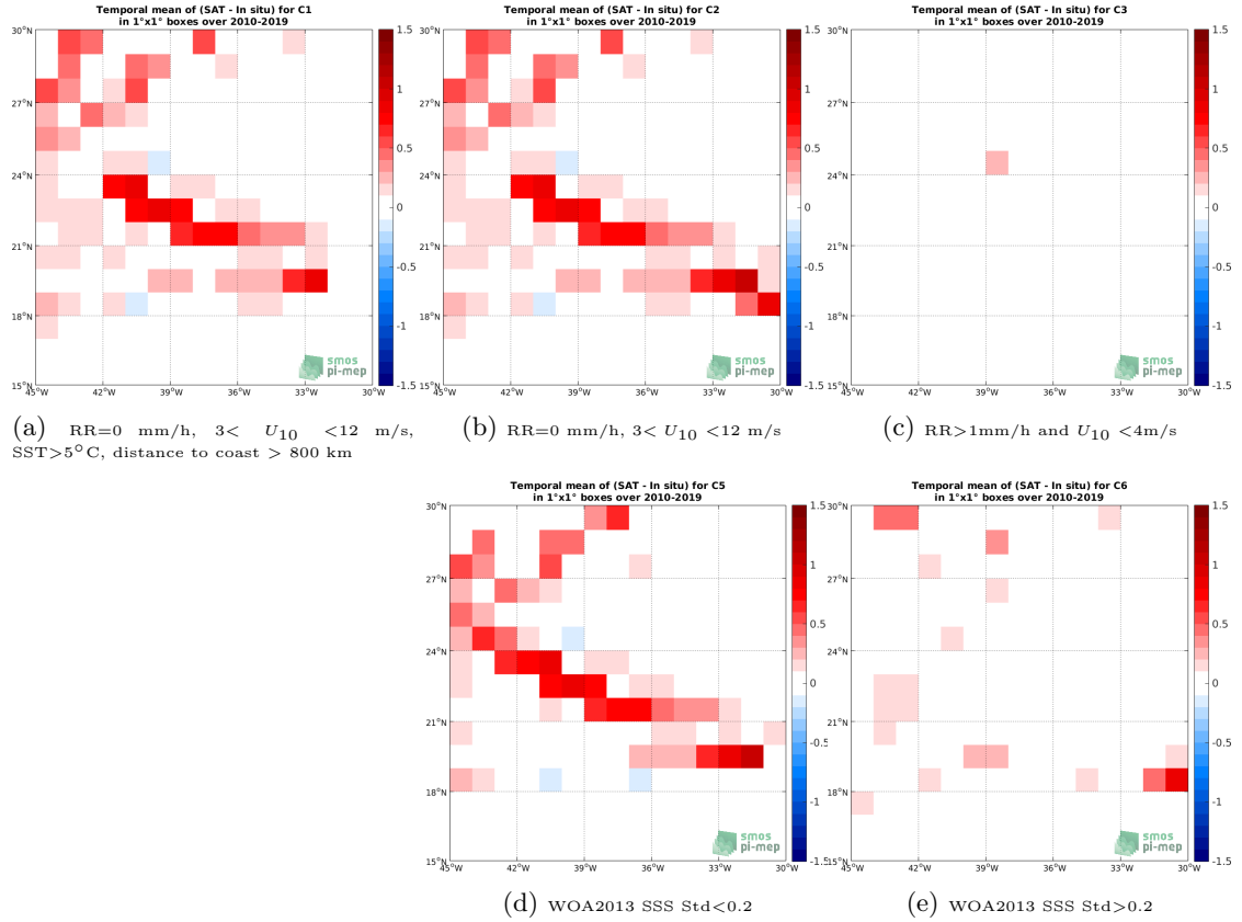
Figure 12: Temporal mean gridded over spatial boxes of size 1^{\circ}\times 1^{\circ} of \Delta\text{SSS} (SMOS SSS L3 v4 - 18 Days (CATDS-CECOS-LOCEAN) - TSG (SAMOS)) for 5 different subdatasets corresponding to: \text{RR}=0 mm/h, 3 < U_{10} < 12 m/s, \text{SST}>5^{\circ}\text{C} , distance to coast > 800 km (a), \text{RR}=0 mm/h, 3 < U_{10} < 12 m/s (b), \text{RR}>1\text{mm/h} and U_{10} < 4\text{m/s} (c), WOA2013 SSS Std <0.2 (d), WOA2013 SSS Std >0.2 (e).
