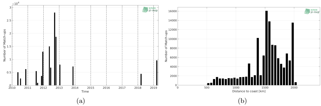
Figure 1: Number of match-ups between TSG (SAMOS) and SMOS SSS L3 v4 - 18 Days (CATDS-CECOS-LOCEAN) SSS as a function of time (a) and as function of the distance to coast (b) over the SPURS 1 Pi-MEP region and for the full satellite product period.
