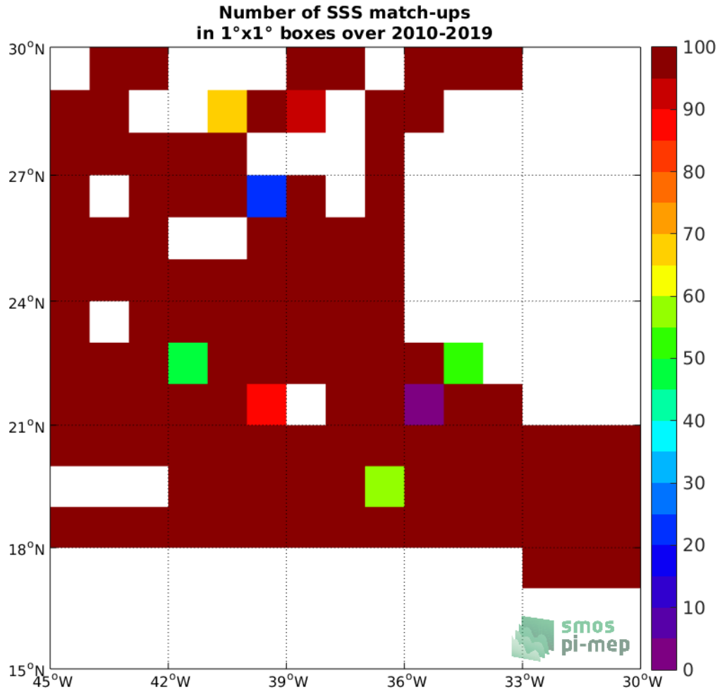
Figure 4: Number of SSS match-ups between TSG (SAMOS) SSS and the SMOS SSS L3 v4 - 18 Days (CATDS-CECOS-LOCEAN) SSS product for the SPURS 1 Pi-MEP region over 1°x1° boxes and for the full satellite product period.
