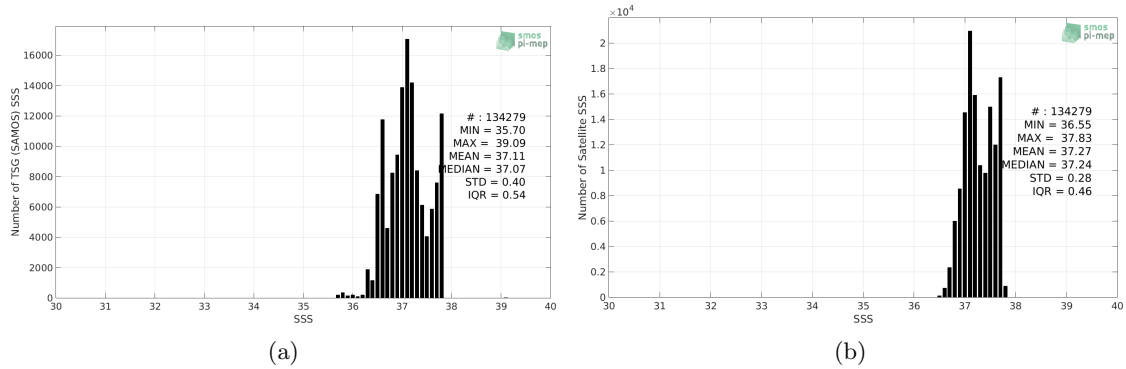
Figure 2: Histograms of SSS from TSG (SAMOS) (a) and SMOS SSS L3 v4 - 18 Days (CATDS-CECOS-LOCEAN) (b) considering all match-up pairs per bins of 0.1 over the SPURS 1 Pi-MEP region and for the full satellite product period.
