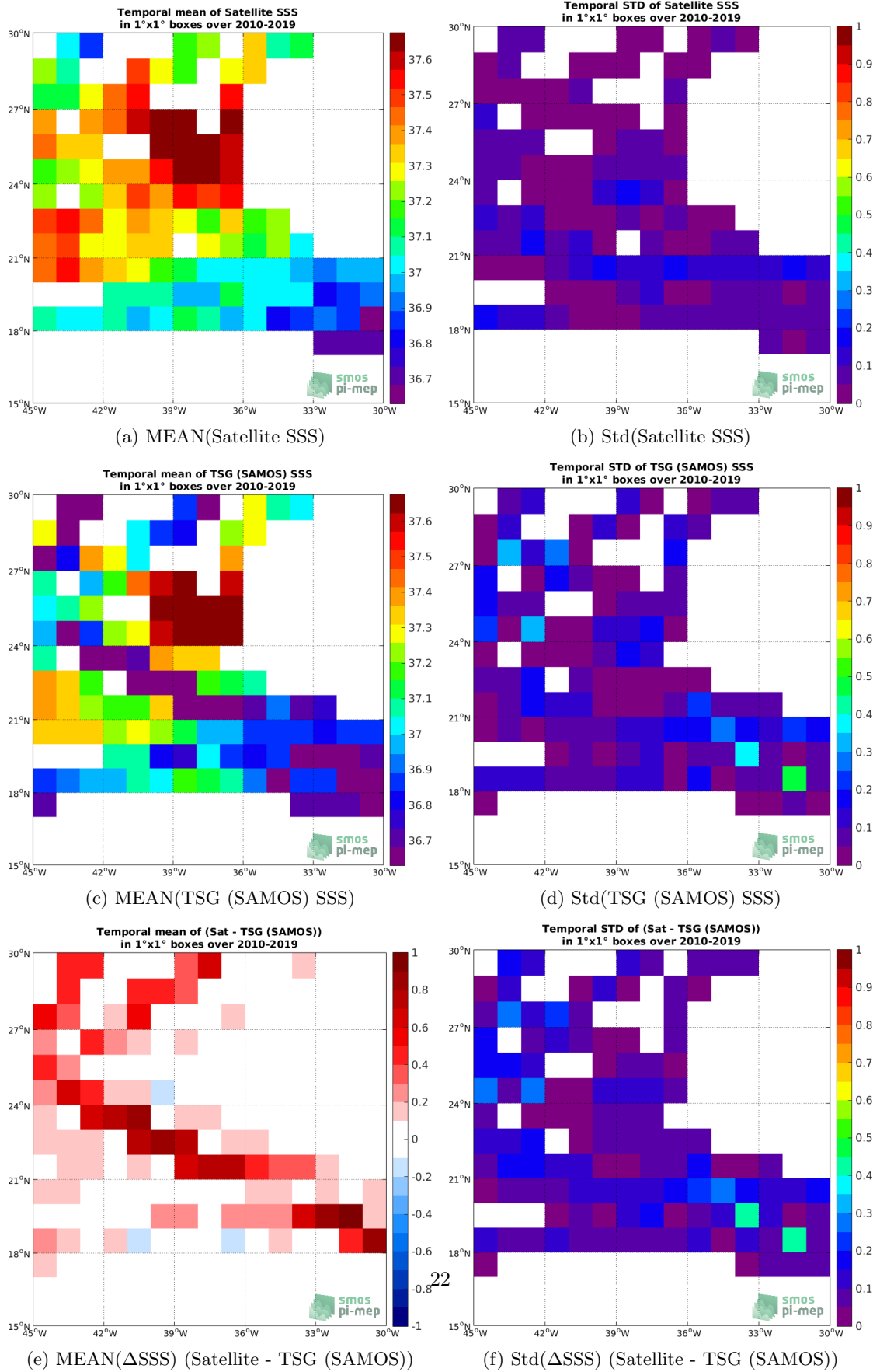
Figure 6: Temporal mean (left) and Std (right) of SSS from SMOS SSS L3 v4 - 18 Days (CATDS-CECOS-LOCEAN) (top), TSG (SAMOS) (middle), and of \Delta SSS (Satellite - TSG (SAMOS)). Only match-up pairs are used to generate these maps.
