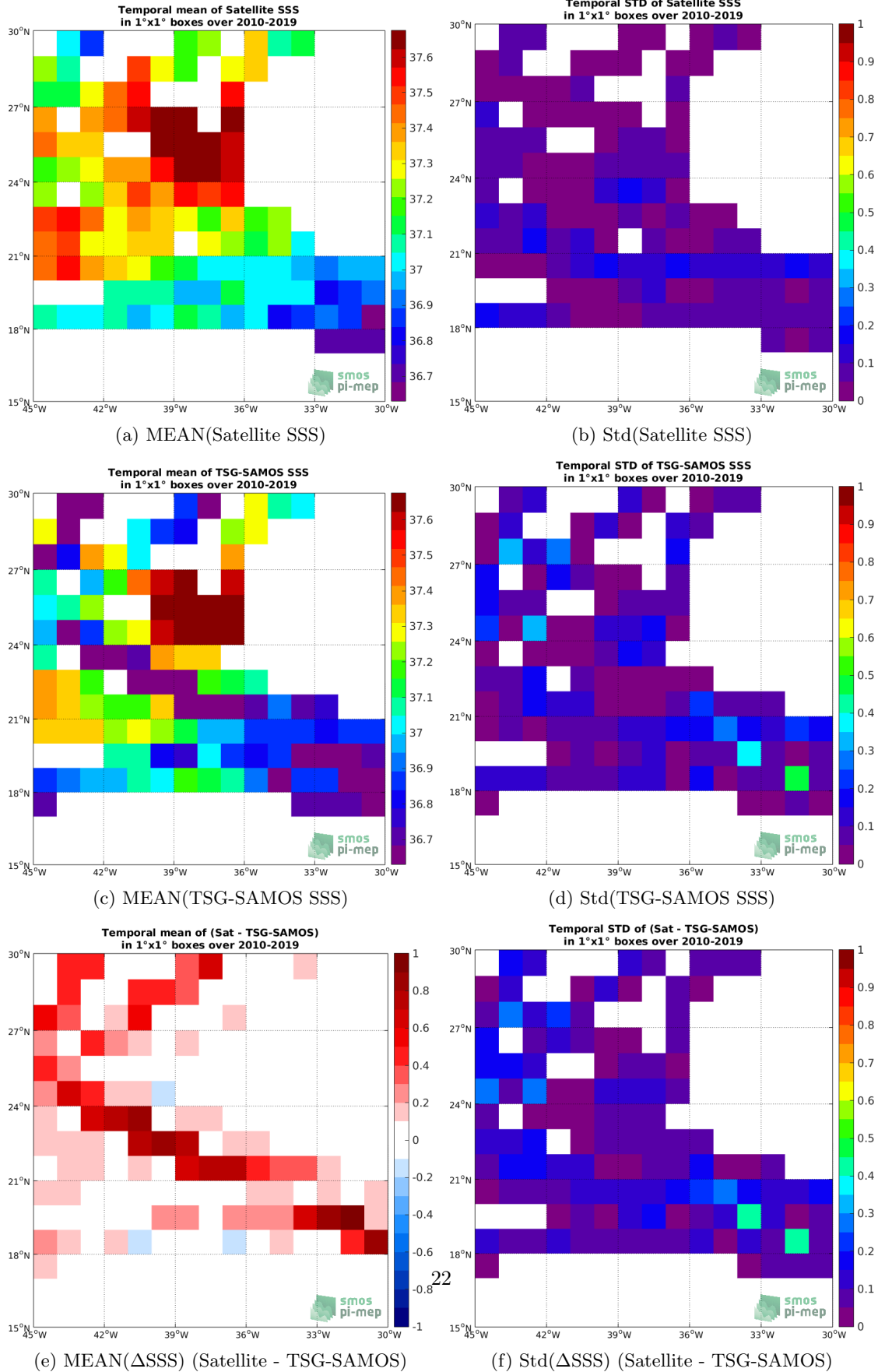
Figure 6: Temporal mean (left) and Std (right) of SSS from SMOS-L3-CATDS-CECOS-LOCEAN-V4-18DAYS-25KM (top), TSG-SAMOS (middle), and of \Delta SSS (Satellite - TSG-SAMOS). Only match-up pairs are used to generate these maps.
