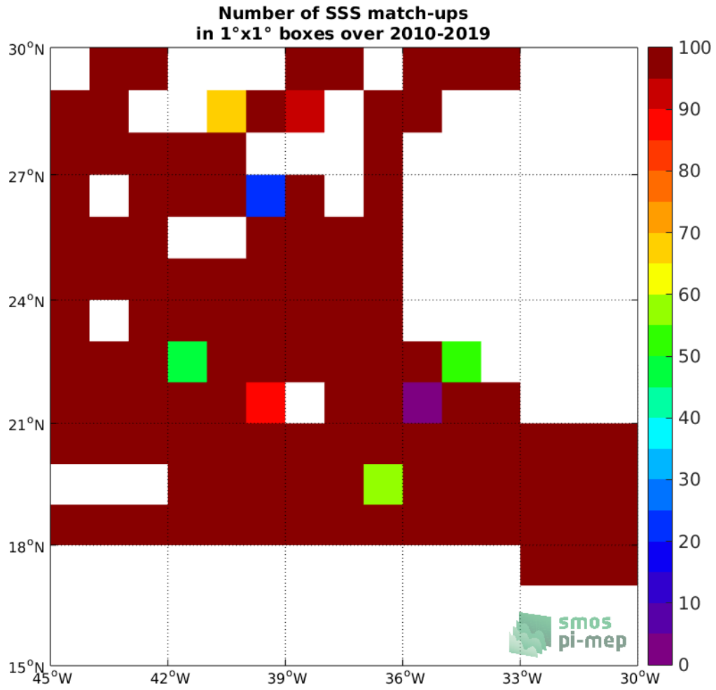
Figure 4: Number of SSS match-ups between TSG-SAMOS SSS and the SMOS-L3-CATDS-CECOS-LOCEAN-V4-18DAYS-25KM SSS product for the SPURS 1 Pi-MEP region over 1°x1° boxes and for the full satellite product period.
