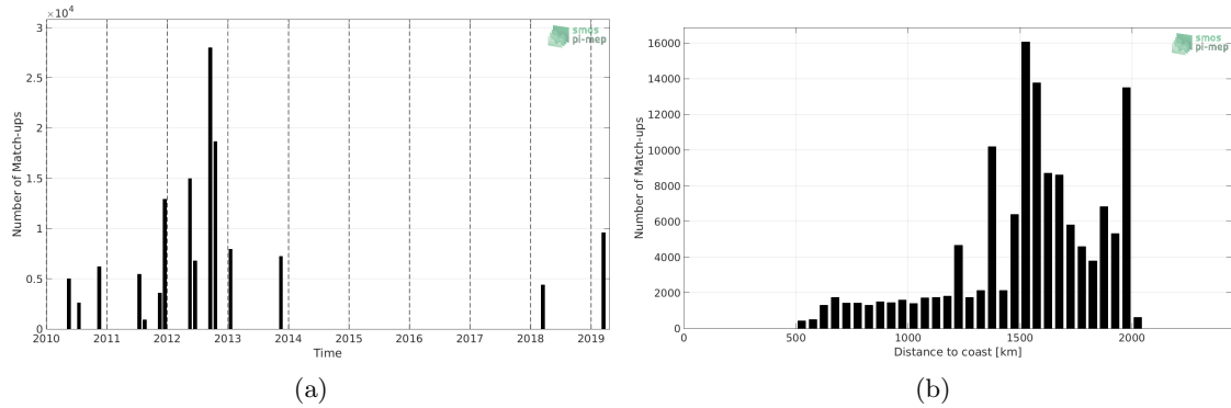
Figure 1: Number of match-ups between TSG-SAMOS and SMOS-L3-CATDS-CECOS-LOCEAN-V4-18DAYS-25KM SSS as a function of time (a) and as function of the distance to coast (b) over the SPURS 1 Pi-MEP region and for the full satellite product period.
