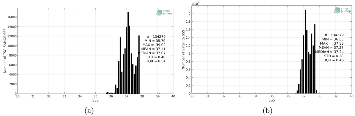
Figure 2: Histograms of SSS from TSG-SAMOS (a) and SMOS-L3-CATDS-CECOS-LOCEAN-V4-18DAYS-25KM (b) considering all match-up pairs per bins of 0.1 over the SPURS 1 Pi-MEP region and for the full satellite product period.
