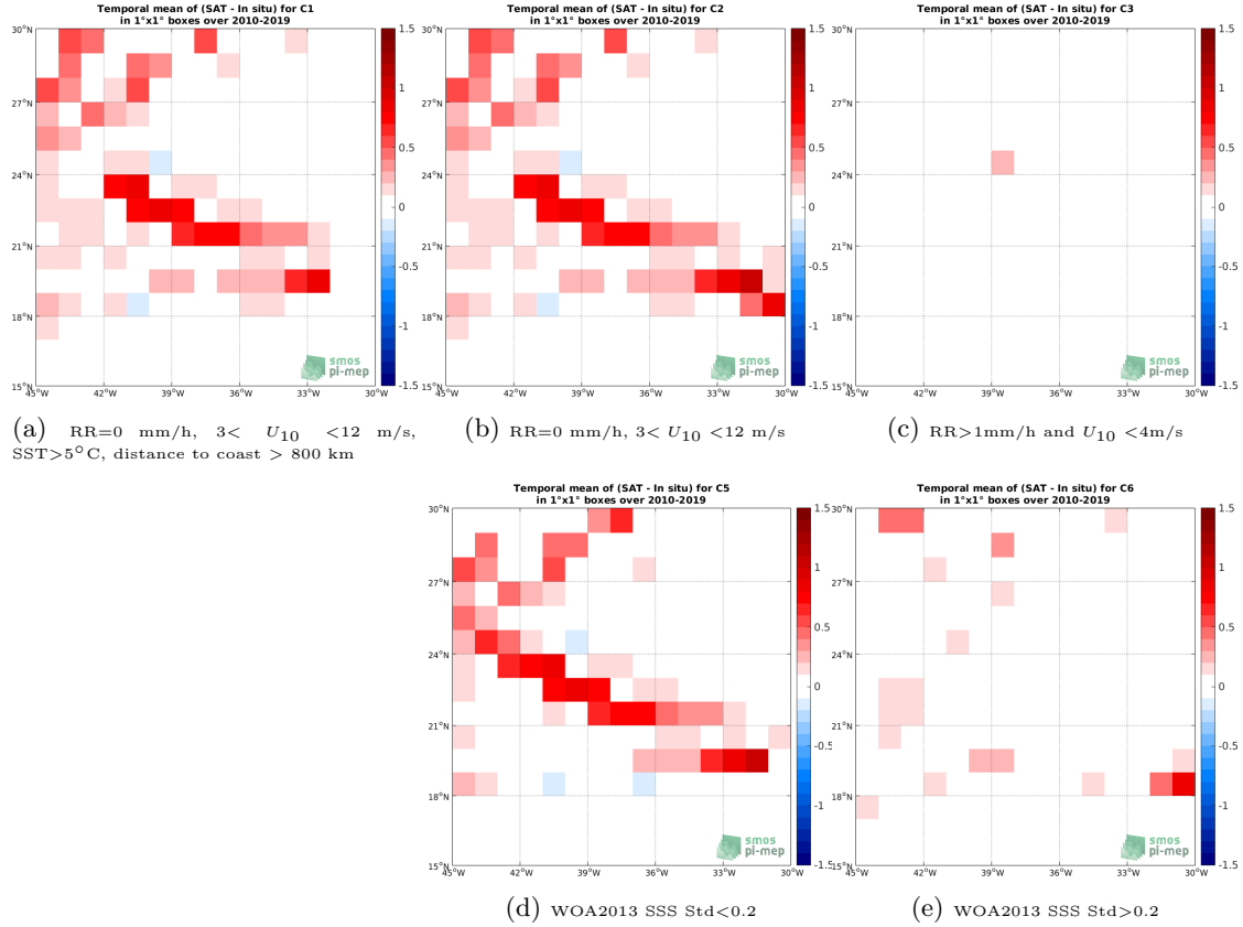
Figure 12: Temporal mean gridded over spatial boxes of size 1^{\circ}\times 1^{\circ} of \Delta\text{SSS} (SMOS-L3-CATDS-CECOS-LOCEAN-V4-18DAYS-25KM - TSG-SAMOS) for 5 different subdatasets corresponding to: RR=0 mm/h, 3 < U_{10} < 12 m/s, SST >5^{\circ}\text{C} , distance to coast > 800 km (a), RR=0 mm/h, 3 < U_{10} < 12 m/s (b), RR >1 mm/h and U_{10} < 4 m/s (c), WOA2013 SSS Std <0.2 (d), WOA2013 SSS Std >0.2 (e).
