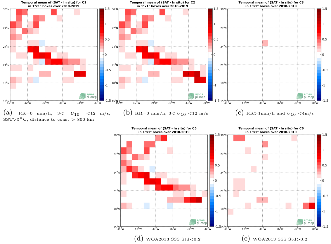
Figure 12: Temporal mean gridded over spatial boxes of size 1^\circ \times 1^\circ of \Delta SSS (SMOS-L3-CATDS-CECOS-LOCEAN-V4-18DAYS-25KM - TSG-SAMOS) for 5 different subdatasets corresponding to: RR=0 mm/h, 3 < U_{10} < 12 m/s, SST>5°C, distance to coast > 800 km (a), RR=0 mm/h, 3 < U_{10} < 12 m/s (b), RR>1mm/h and U_{10} < 4 m/s (c), WOA2013 SSS Std<0.2 (d), WOA2013 SSS Std>0.2 (e).
