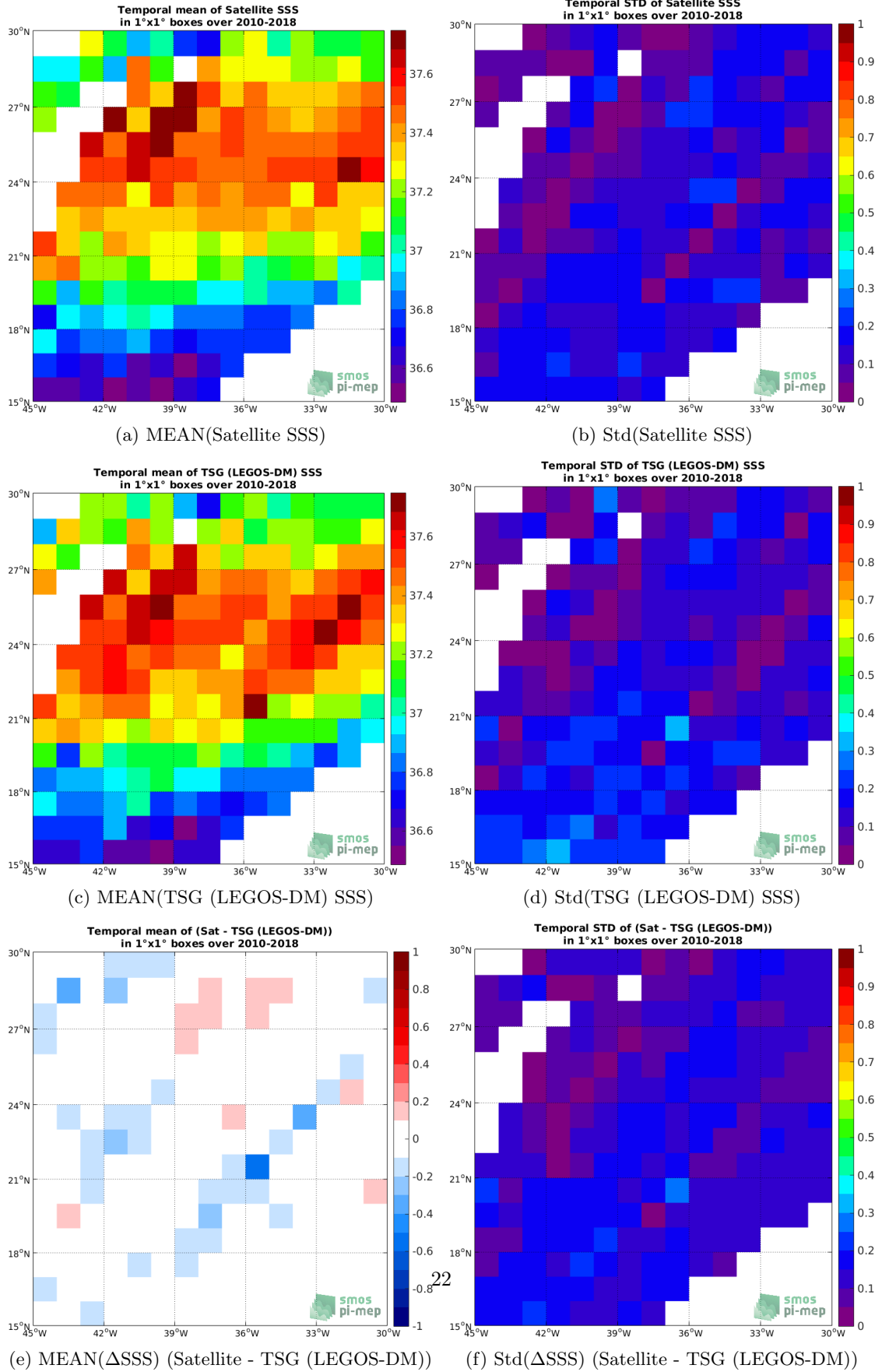
Figure 6: Temporal mean (left) and Std (right) of SSS from SMOS SSS L3 v4 - 18 Days (CATDS-CECOS-LOCEAN) (top), TSG (LEGOS-DM) (middle), and of \Delta SSS (Satellite - TSG (LEGOS-DM)). Only match-up pairs are used to generate these maps.
