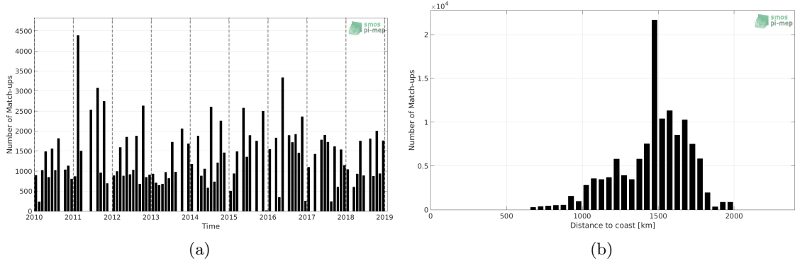
Figure 1: Number of match-ups between TSG (LEGOS-DM) and SMOS SSS L3 v4 - 18 Days (CATDS-CECOS-LOCEAN) SSS as a function of time (a) and as function of the distance to coast (b) over the SPURS 1 Pi-MEP region and for the full satellite product period.
