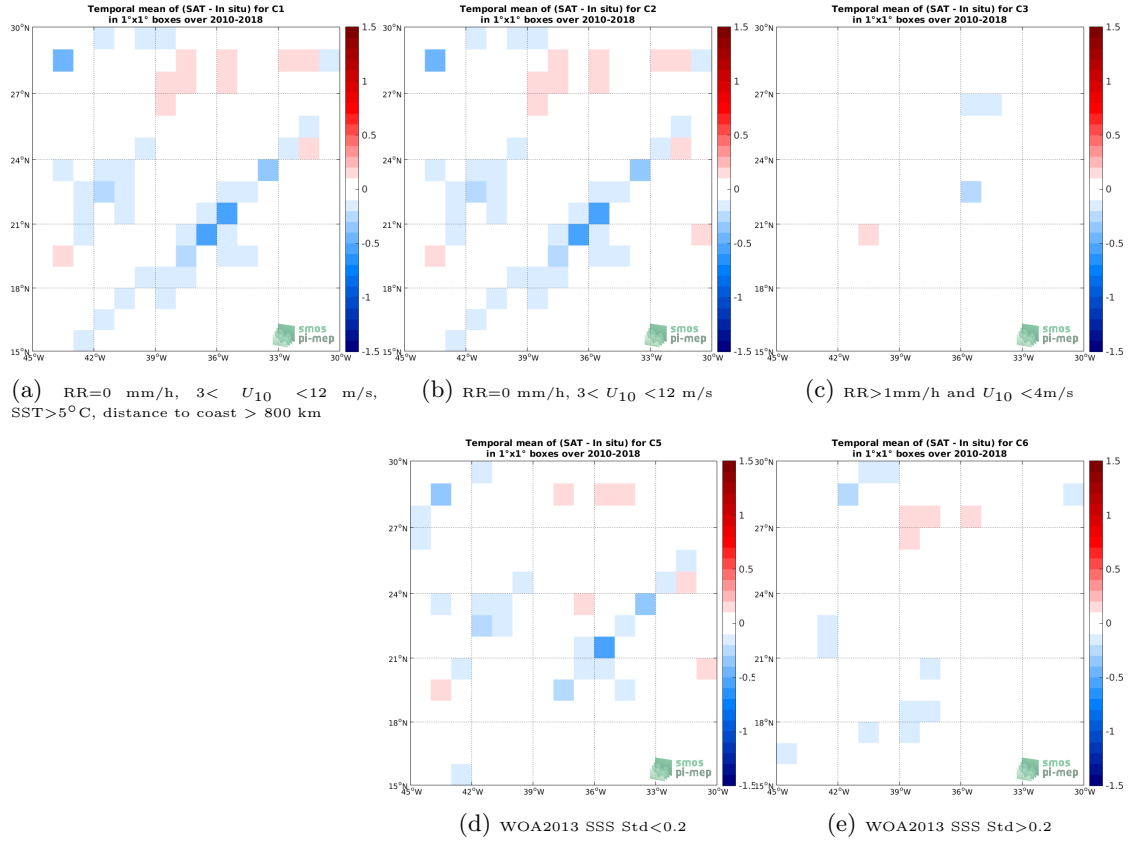
Figure 12: Temporal mean gridded over spatial boxes of size 1^{\circ}\times 1^{\circ} of \Delta\text{SSS} (SMOS SSS L3 v4 - 18 Days (CATDS-CECOS-LOCEAN) - TSG (LEGOS-DM)) for 5 different subdatasets corresponding to: RR=0 mm/h, 3 < U_{10} < 12 m/s, SST >5^{\circ}\text{C} , distance to coast > 800 km (a), RR=0 mm/h, 3 < U_{10} < 12 m/s (b), RR >1 mm/h and U_{10} < 4 m/s (c), WOA2013 SSS Std <0.2 (d), WOA2013 SSS Std >0.2 (e).
