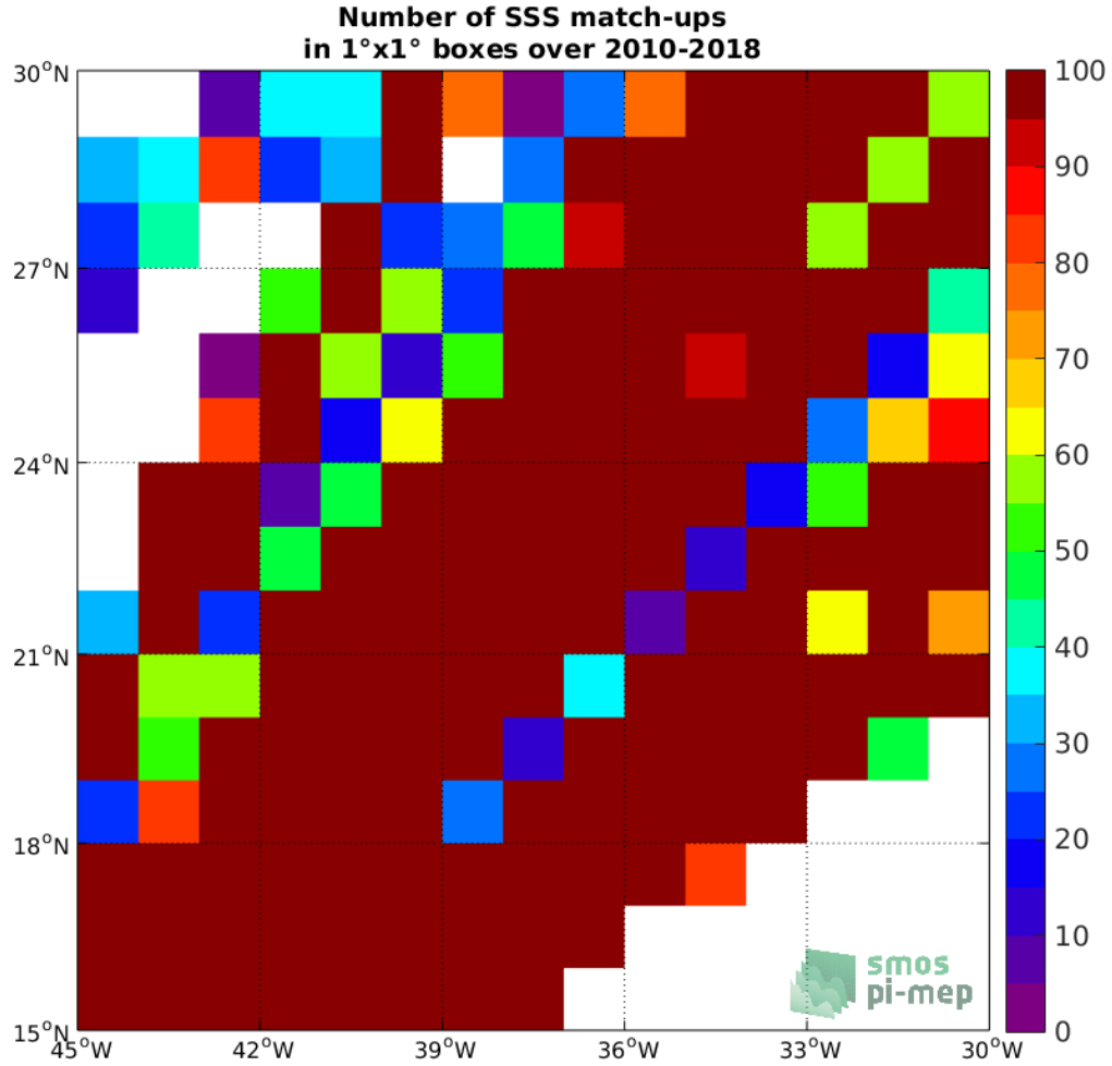
Figure 4: Number of SSS match-ups between TSG (LEGOS-DM) SSS and the SMOS SSS L3 v4 - 18 Days (CATDS-CECOS-LOCEAN) SSS product for the SPURS 1 Pi-MEP region over 1°x1° boxes and for the full satellite product period.
