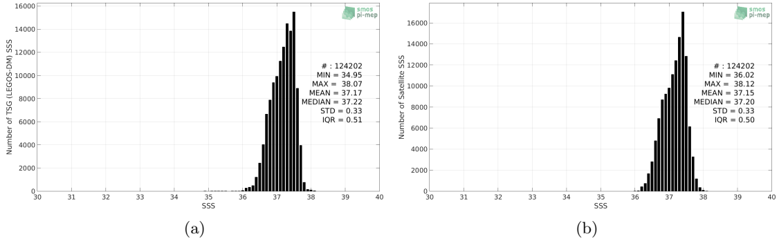
Figure 2: Histograms of SSS from TSG (LEGOS-DM) (a) and SMOS SSS L3 v4 - 18 Days (CATDS-CECOS-LOCEAN) (b) considering all match-up pairs per bins of 0.1 over the SPURS 1 Pi-MEP region and for the full satellite product period.
