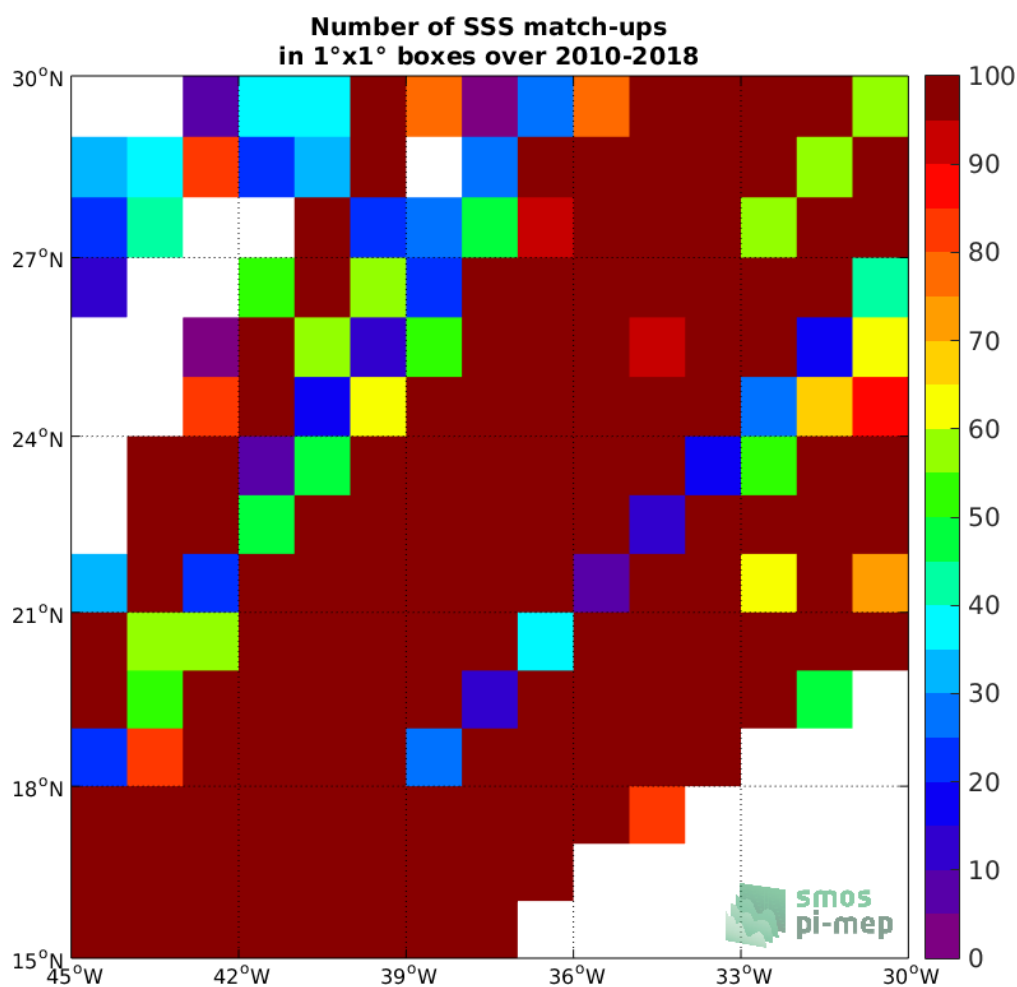
Figure 4: Number of SSS match-ups between TSG-LEGOS-DM SSS and the SMOS-L3-CATDS-CECOS-LOCEAN-V4-18DAYS-25KM SSS product for the SPURS 1 Pi-MEP region over 1°x1° boxes and for the full satellite product period.
