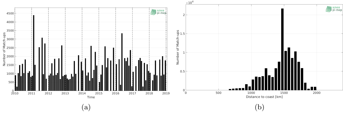
Figure 1: Number of match-ups between TSG-LEGOS-DM and SMOS-L3-CATDS-CECOS-LOCEAN-V4-18DAYS-25KM SSS as a function of time (a) and as function of the distance to coast (b) over the SPURS 1 Pi-MEP region and for the full satellite product period.
