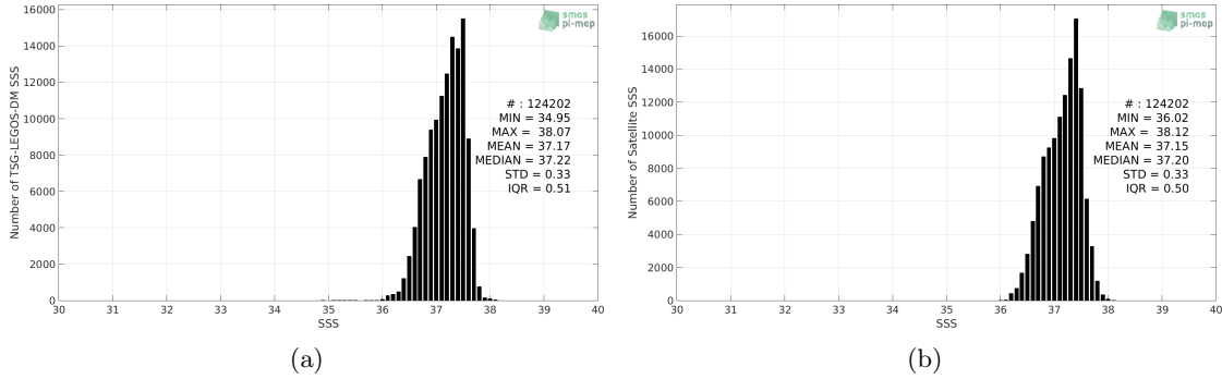
Figure 2: Histograms of SSS from TSG-LEGOS-DM (a) and SMOS-L3-CATDS-CECOS-LOCEAN-V4-18DAYS-25KM (b) considering all match-up pairs per bins of 0.1 over the SPURS 1 Pi-MEP region and for the full satellite product period.
