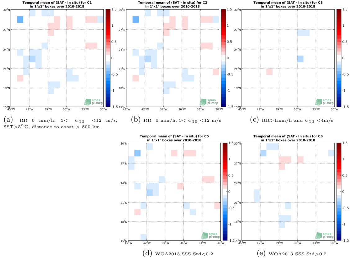
Figure 12: Temporal mean gridded over spatial boxes of size 1^\circ \times 1^\circ of \Delta SSS (SMOS-L3-CATDS-CECOS-LOCEAN-V4-18DAYS-25KM - TSG-LEGOS-DM) for 5 different subdatasets corresponding to: RR=0 mm/h, 3 < U_{10} < 12 m/s, SST >5^\circ C, distance to coast > 800 km (a), RR=0 mm/h, 3 < U_{10} < 12 m/s (b), RR >1 mm/h and U_{10} < 4 m/s (c), WOA2013 SSS Std <0.2 (d), WOA2013 SSS Std >0.2 (e).
