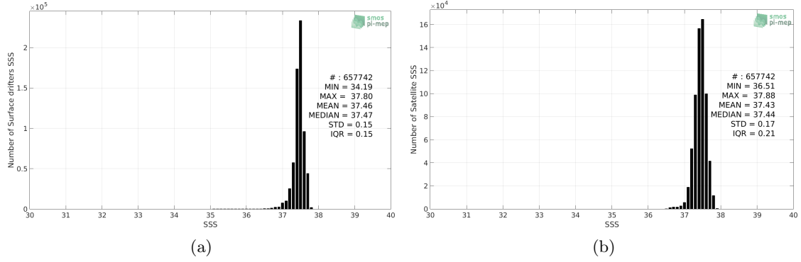
Figure 2: Histograms of SSS from Surface drifters (a) and SMOS SSS L3 v4 - 18 Days (CATDS-CECOS-LOCEAN) (b) considering all match-up pairs per bins of 0.1 over the SPURS 1 Pi-MEP region and for the full satellite product period.
