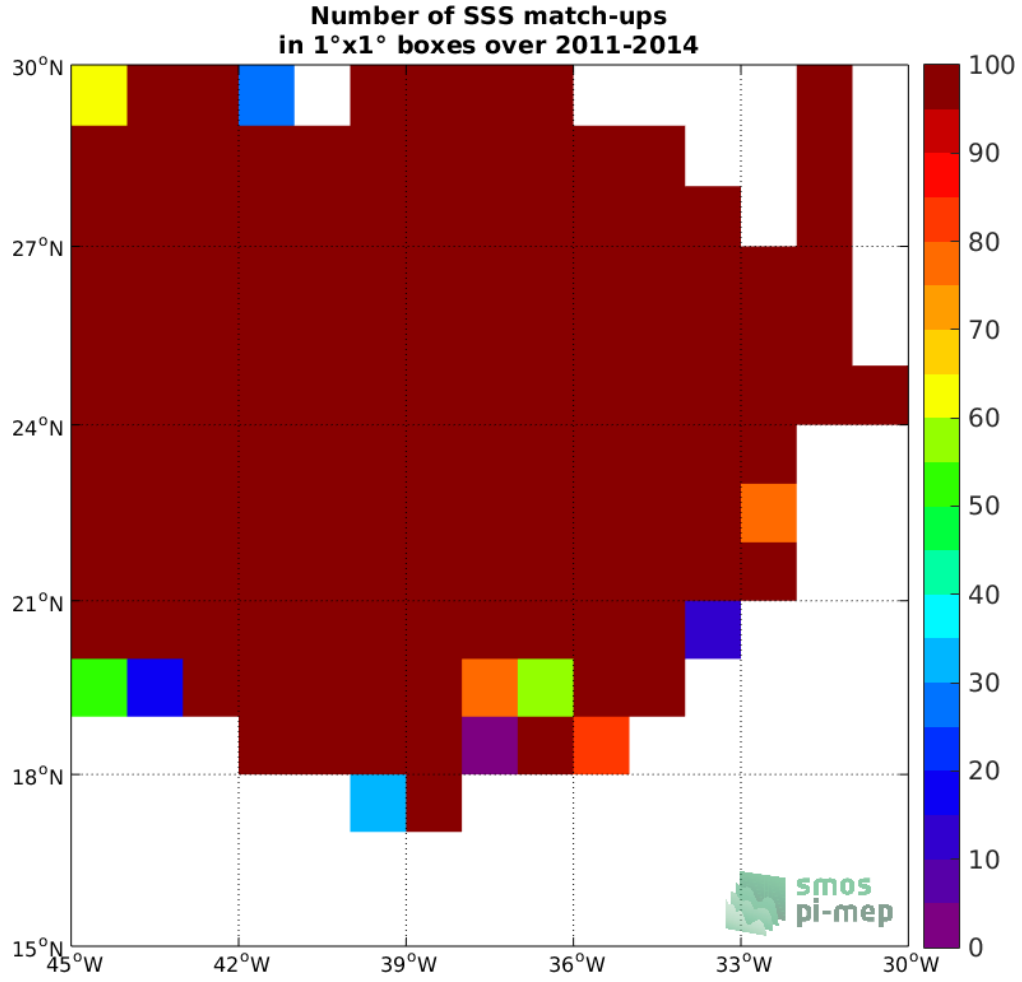
Figure 3: Number of SSS match-ups between Surface drifters SSS and the SMOS SSS L3 v4 - 18 Days (CATDS-CECOS-LOCEAN) SSS product for the SPURS 1 Pi-MEP region over 1°x1° boxes and for the full satellite product period.
