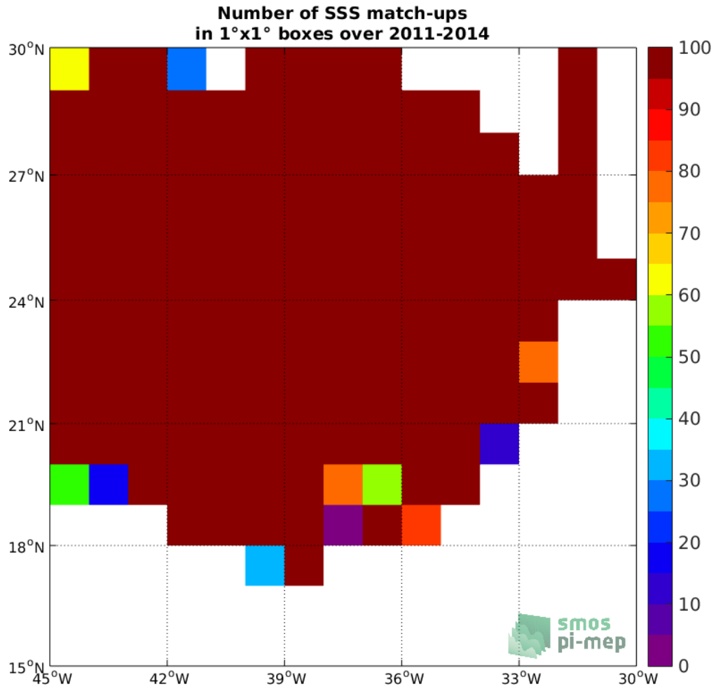
Figure 3: Number of SSS match-ups between Surface drifters SSS and the SMOS-L3-CATDS-CECOS-LOCEAN-V4-18DAYS-25KM SSS product for the SPURS 1 Pi-MEP region over 1°x1° boxes and for the full satellite product period.
