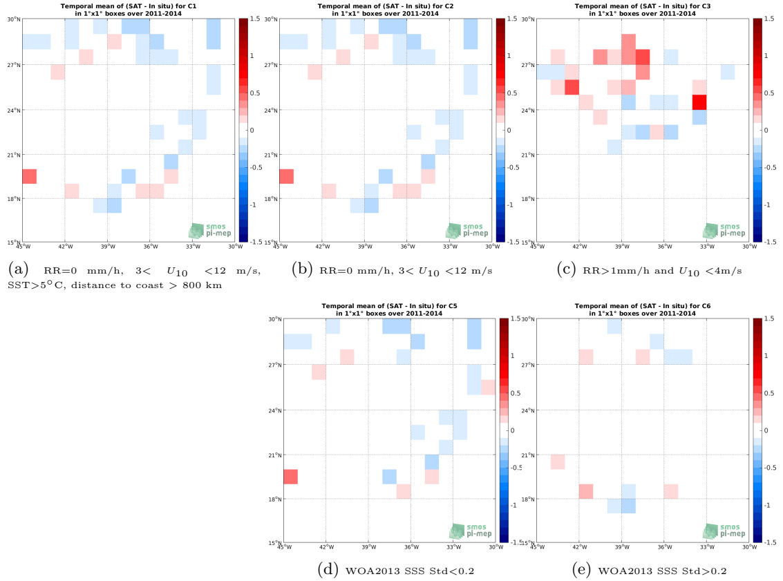
Figure 11: Temporal mean gridded over spatial boxes of size 1^{\circ}\times 1^{\circ} of \Delta\text{SSS} (SMOS-L3-CATDS-CECOS-LOCEAN-V4-18DAYS-25KM - Surface drifters) for 5 different subdatasets corresponding to: RR=0 mm/h, 3 < U_{10} < 12 m/s, SST >5^{\circ}\text{C} , distance to coast > 800 km (a), RR=0 mm/h, 3 < U_{10} < 12 m/s (b), RR >1 mm/h and U_{10} < 4 m/s (c), WOA2013 SSS Std <0.2 (d), WOA2013 SSS Std >0.2 (e).
