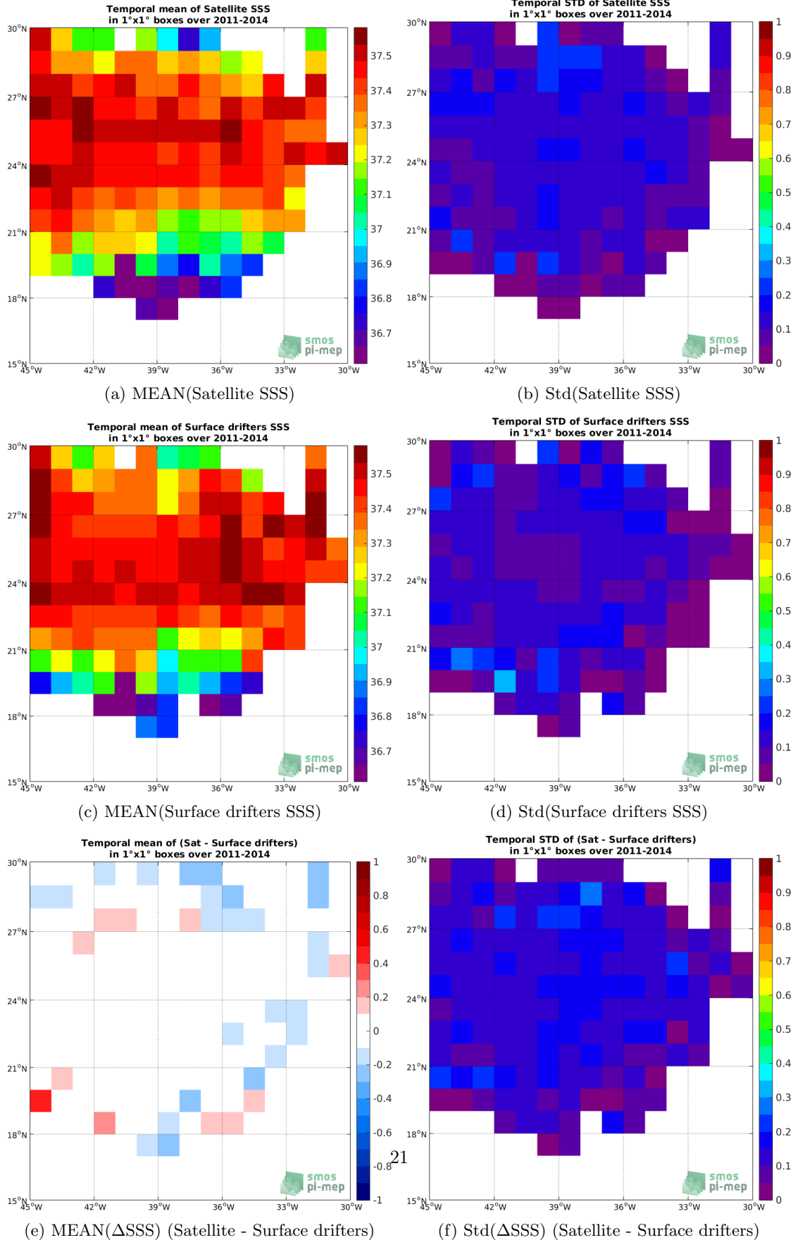
Figure 5: Temporal mean (left) and Std (right) of SSS from SMOS-L3-CATDS-CECOS-LOCEAN-V4-18DAYS-25KM (top), Surface drifters (middle), and of \Delta SSS (Satellite - Surface drifters). Only match-up pairs are used to generate these maps.
