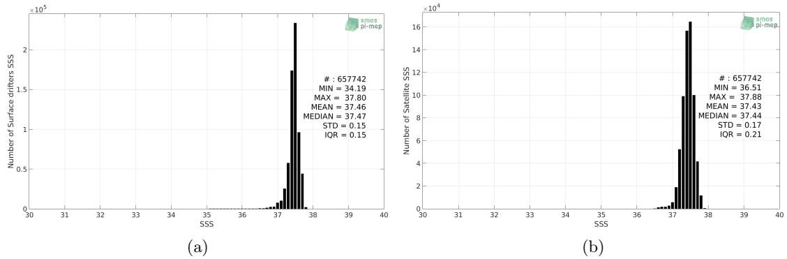
Figure 2: Histograms of SSS from Surface drifters (a) and SMOS-L3-CATDS-CECOS-LOCEAN-V4-18DAYS-25KM (b) considering all match-up pairs per bins of 0.1 over the SPURS 1 Pi-MEP region and for the full satellite product period.
