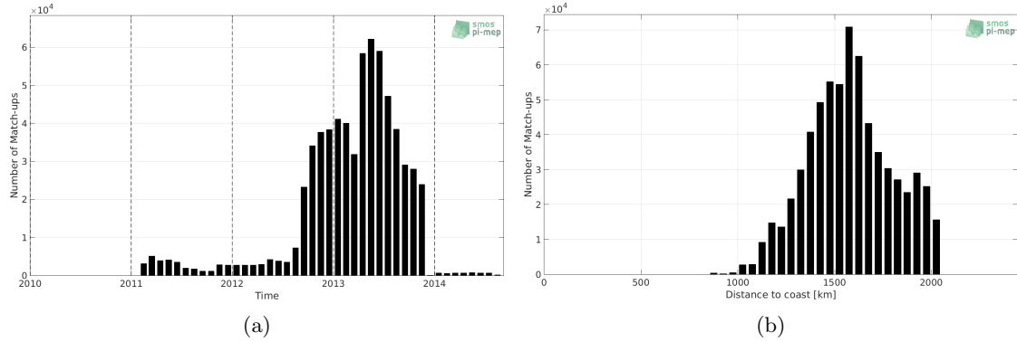
Figure 1: Number of match-ups between Surface drifters and SMOS-L3-CATDS-CECOS-LOCEAN-V4-18DAYS-25KM SSS as a function of time (a) and as function of the distance to coast (b) over the SPURS 1 Pi-MEP region and for the full satellite product period.
