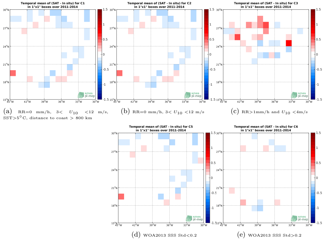
Figure 11: Temporal mean gridded over spatial boxes of size 1^\circ \times 1^\circ of \Delta SSS (SMOS-L3-CATDS-CECOS-LOCEAN-V4-18DAYS-25KM - Surface drifters) for 5 different subdatasets corresponding to:RR=0 mm/h, 3 < U_{10} < 12 m/s, SST>5°C, distance to coast > 800 km (a), RR=0 mm/h, 3 < U_{10} < 12 m/s (b), RR>1mm/h and U_{10} < 4 m/s (c), WOA2013 SSS Std<0.2 (d), WOA2013 SSS Std>0.2 (e).
