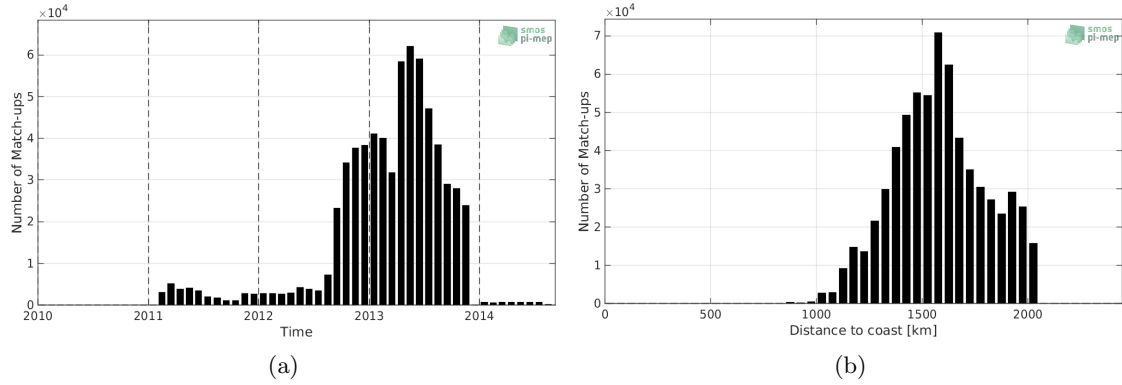
Figure 1: Number of match-ups between Surface drifters and SMOS-L3-CATDS-CECOS-LOCEAN-V4-18DAYS-25KM SSS as a function of time (a) and as function of the distance to coast (b) over the SPURS 1 Pi-MEP region and for the full satellite product period.
