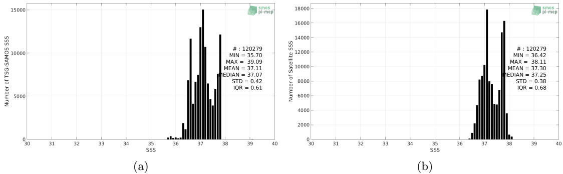
Figure 2: Histograms of SSS from TSG-SAMOS (a) and SMOS-L3-CATDS-CECOS-LOCEAN-V3-9DAYS-25KM (b) considering all match-up pairs per bins of 0.1 over the SPURS 1 Pi-MEP region and for the full satellite product period.
