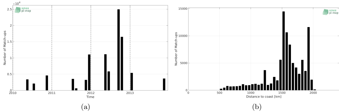
Figure 1: Number of match-ups between TSG-SAMOS and SMOS-L3-CATDS-CECOS-LOCEAN-V3-9DAYS-25KM SSS as a function of time (a) and as function of the distance to coast (b) over the SPURS 1 Pi-MEP region and for the full satellite product period.
