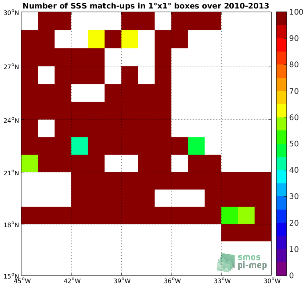
Figure 4: Number of SSS match-ups between TSG-SAMOS SSS and the SMOS-L3-CATDS-CECOS-LOCEAN-V3-9DAYS-25KM SSS product for the SPURS 1 Pi-MEP region over 1°x1° boxes and for the full satellite product period.
