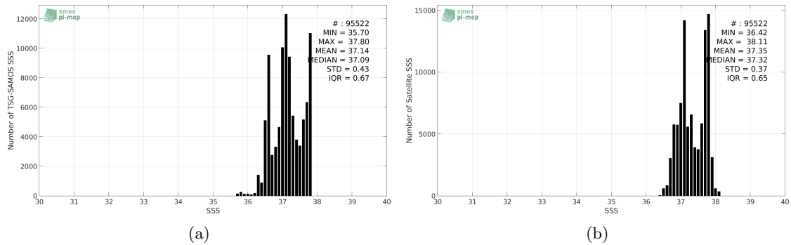
Figure 2: Histograms of SSS from TSG-SAMOS (a) and SMOS-L3-CATDS-CECOS-LOCEAN-V3-9DAYS-25KM (b) considering all match-up pairs per bins of 0.1 over the SPURS 1 Pi-MEP region and for the full satellite product period.
