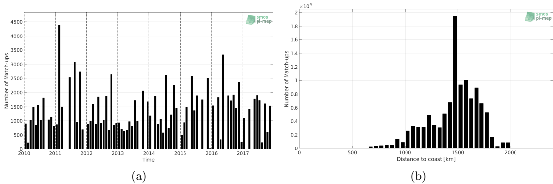
Figure 1: Number of match-ups between TSG-LEGOS-DM and SMOS-L3-CATDS-CECOS-LOCEAN-V3-9DAYS-25KM SSS as a function of time (a) and as function of the distance to coast (b) over the SPURS 1 Pi-MEP region and for the full satellite product period.
