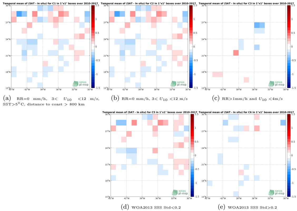
Figure 12: Temporal mean gridded over spatial boxes of size 1^\circ \times 1^\circ of \Delta SSS (SMOS-L3-CATDS-CECOS-LOCEAN-V3-9DAYS-25KM - TSG-LEGOS-DM) for 5 different subdatasets corresponding to:RR=0 mm/h, 3 < U_{10} < 12 m/s, SST >5^\circ C, distance to coast > 800 km (a), RR=0 mm/h, 3 < U_{10} < 12 m/s (b), RR >1 mm/h and U_{10} < 4 m/s (c), WOA2013 SSS Std <0.2 (d), WOA2013 SSS Std >0.2 (e).
