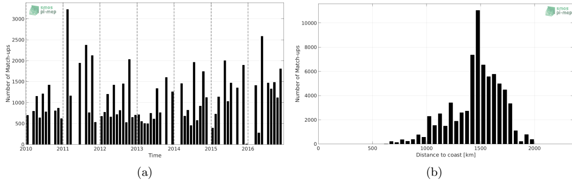
Figure 1: Number of match-ups between TSG-LEGOS-DM and SMOS-L3-CATDS-CECOS-LOCEAN-V3-9DAYS-25KM SSS as a function of time (a) and as function of the distance to coast (b) over the SPURS 1 Pi-MEP region and for the full satellite product period.
