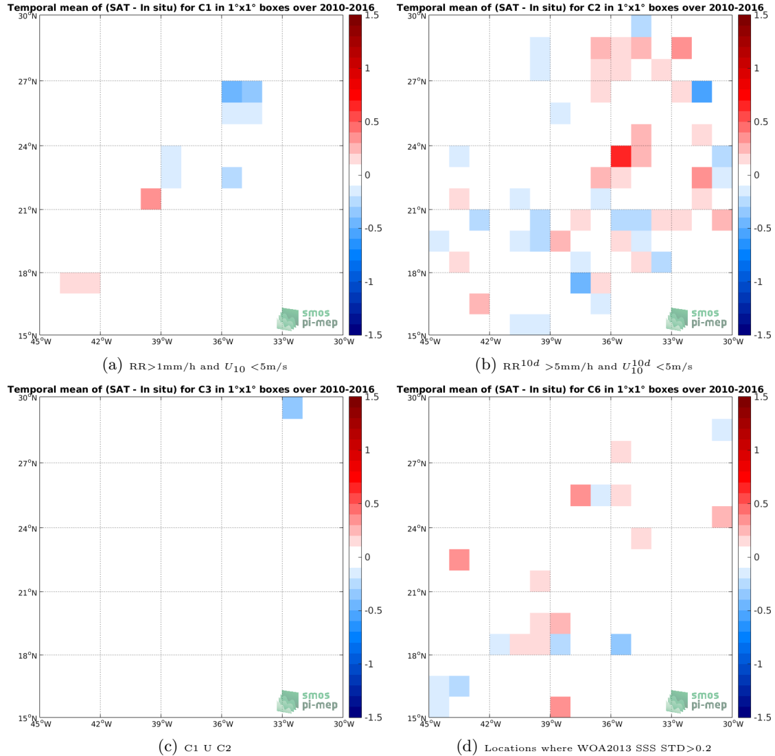
Figure 12: Temporal mean gridded over spatial boxes of size 1^\circ \times 1^\circ of \Delta SSS (SMOS-L3-CATDS-CECOS-LOCEAN-V3-9DAYS-25KM - TSG-LEGOS-DM) for 4 different subdatasets corresponding to: RR > 1\text{mm/h} and U_{10} < 5\text{m/s} (a), RR^{10d} > 5\text{mm/h} and U_{10}^{10d} < 5\text{m/s} (b), C1 U C2 (c), Locations where WOA2013 SSS STD > 0.2 (d).
