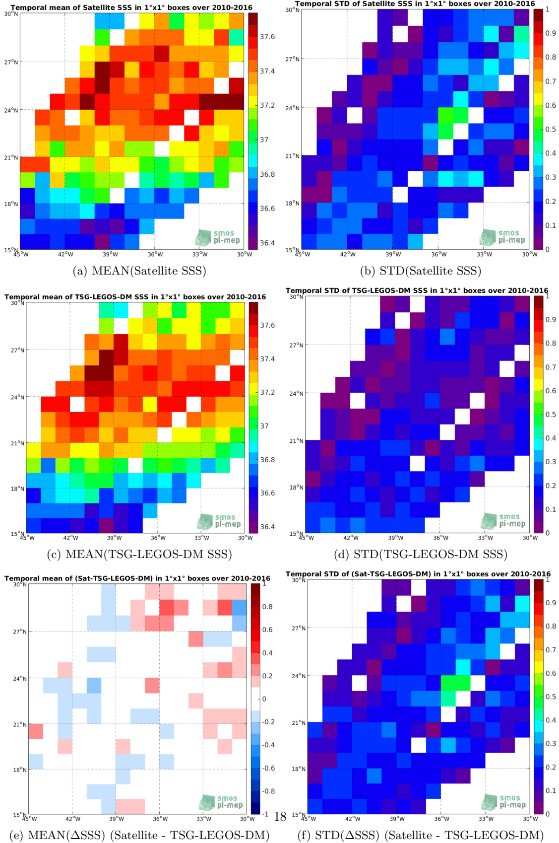
Figure 6: Temporal mean (left) and STD (right) of SSS from SMOS-L3-CATDS-CECOS-LOCEAN-V3-9DAYS-25KM (top), TSG-LEGOS-DM (middle), and of \Delta SSS (Satellite - TSG-LEGOS-DM). Only match-up pairs are used to generate these maps.
