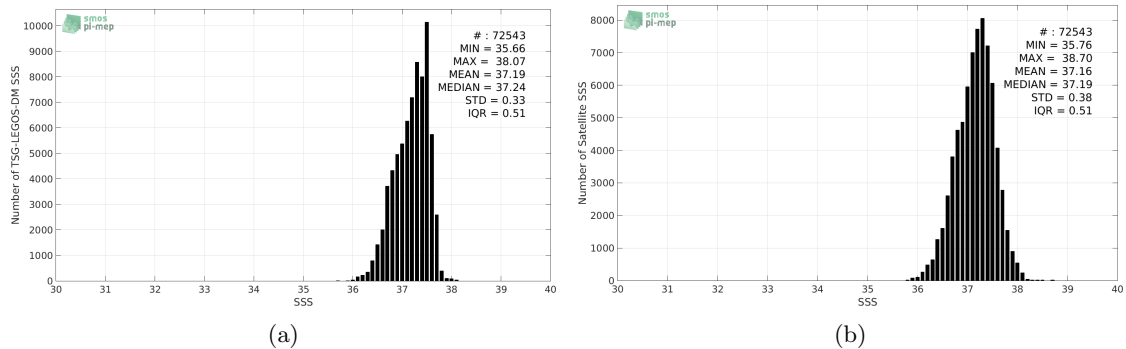
Figure 2: Histograms of SSS from TSG-LEGOS-DM (a) and SMOS-L3-CATDS-CECOS-LOCEAN-V3-9DAYS-25KM (b) considering all match-up pairs per bins of 0.1 over the SPURS 1 Pi-MEP region and for the full satellite product period.
