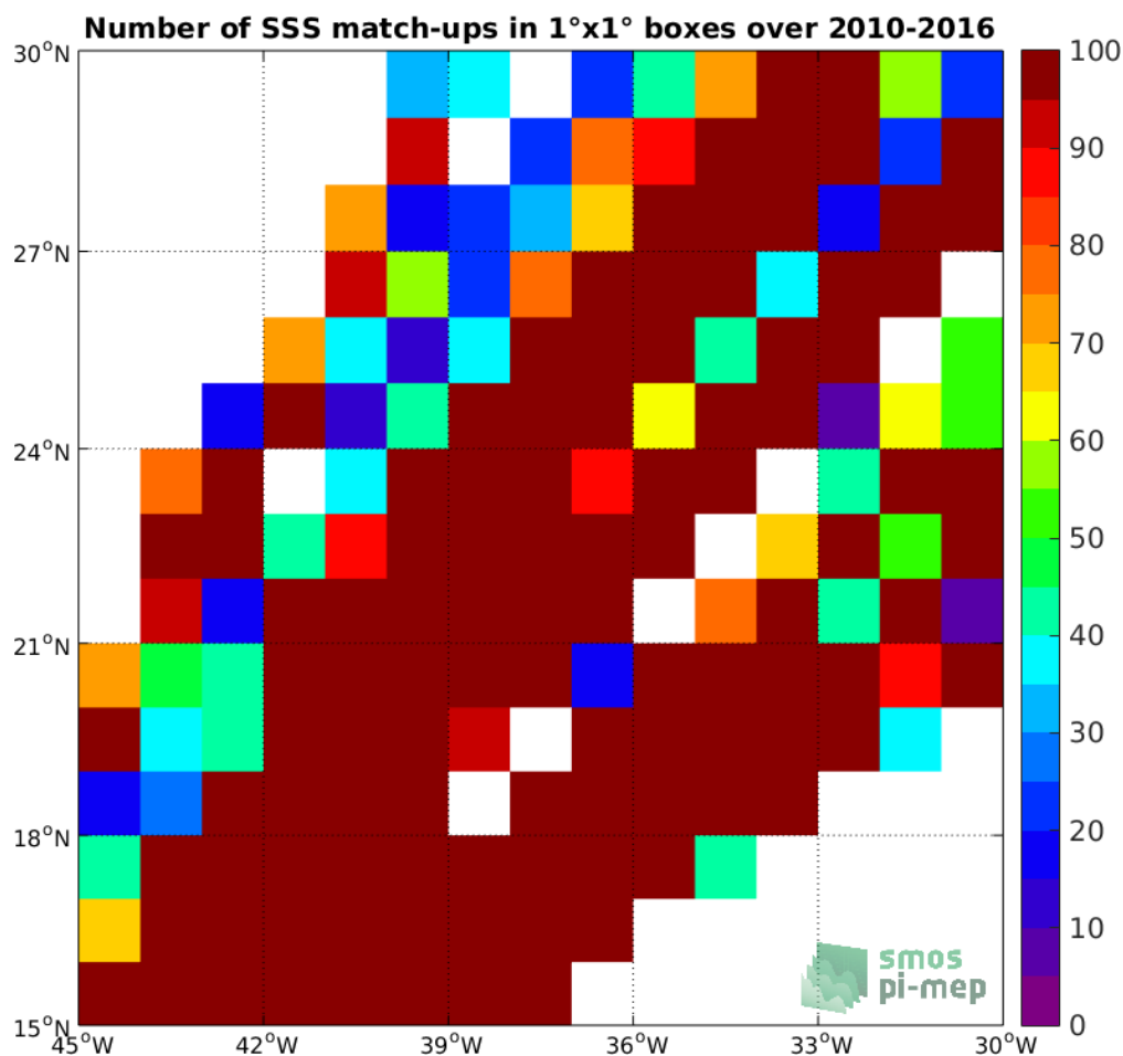
Figure 4: Number of SSS match-ups between TSG-LEGOS-DM SSS and the SMOS-L3-CATDS-CECOS-LOCEAN-V3-9DAYS-25KM SSS product for the SPURS 1 Pi-MEP region over 1°x1° boxes and for the full satellite product period.
