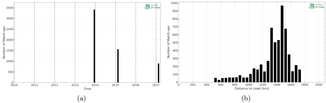
Figure 1: Number of match-ups between TSG-GOSUD-Sailing-ship and SMOS-L3-CATDS-CECOS-LOCEAN-V3-9DAYS-25KM SSS as a function of time (a) and as function of the distance to coast (b) over the SPURS 1 Pi-MEP region and for the full satellite product period.
