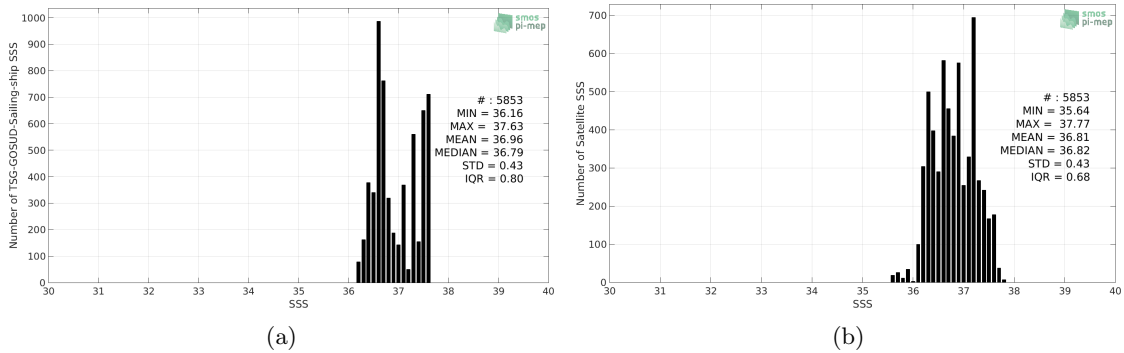
Figure 2: Histograms of SSS from TSG-GOSUD-Sailing-ship (a) and SMOS-L3-CATDS-CECOS-LOCEAN-V3-9DAYS-25KM (b) considering all match-up pairs per bins of 0.1 over the SPURS 1 Pi-MEP region and for the full satellite product period.
