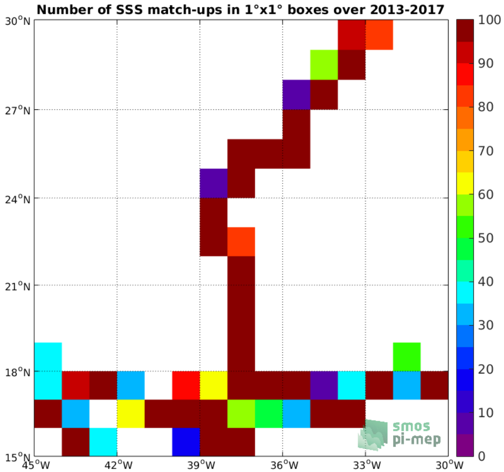
Figure 4: Number of SSS match-ups between TSG-GOSUD-Sailing-ship SSS and the SMOS-L3-CATDS-CECOS-LOCEAN-V3-9DAYS-25KM SSS product for the SPURS 1 Pi-MEP region over 1°x1° boxes and for the full satellite product period.
