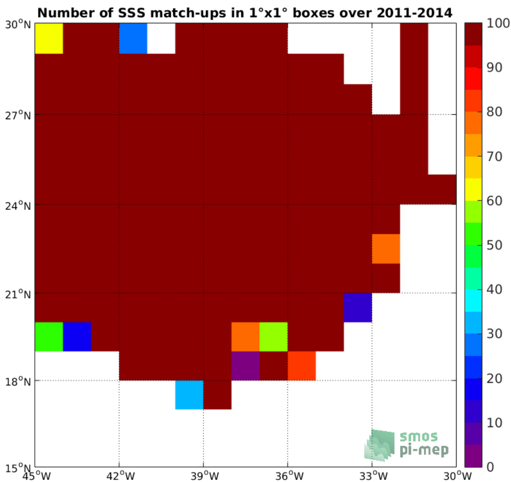
Figure 3: Number of SSS match-ups between Surface drifters SSS and the SMOS-L3-CATDS-CECOS-LOCEAN-V3-9DAYS-25KM SSS product for the SPURS 1 Pi-MEP region over 1°x1° boxes and for the full satellite product period.
