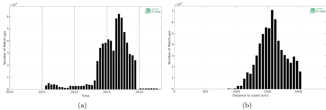
Figure 1: Number of match-ups between Surface drifters and SMOS-L3-CATDS-CECOS-LOCEAN-V3-9DAYS-25KM SSS as a function of time (a) and as function of the distance to coast (b) over the SPURS 1 Pi-MEP region and for the full satellite product period.
