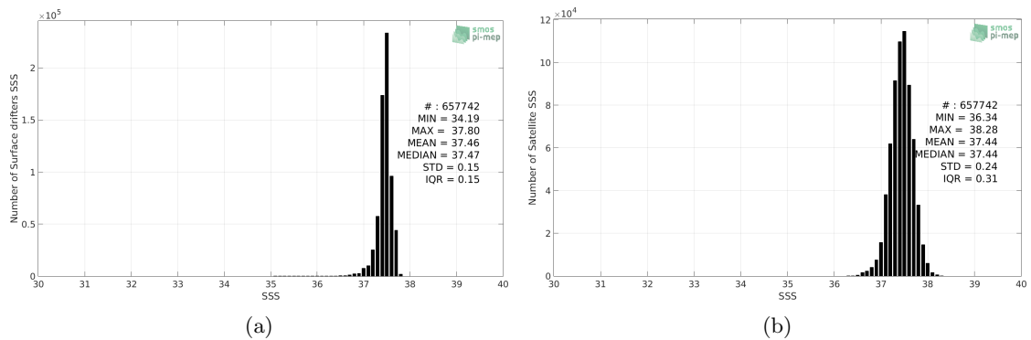
Figure 2: Histograms of SSS from Surface drifters (a) and SMOS-L3-CATDS-CECOS-LOCEAN-V3-9DAYS-25KM (b) considering all match-up pairs per bins of 0.1 over the SPURS 1 Pi-MEP region and for the full satellite product period.
