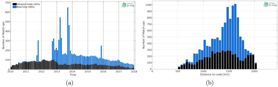
Figure 1: Number of match-ups between Argo and SMOS-L3-CATDS-CECOS-LOCEAN-V3-9DAYS-25KM SSS as a function of time (a) and as function of the distance to coast (b) over the SPURS 1 Pi-MEP region and for the full satellite product period.
