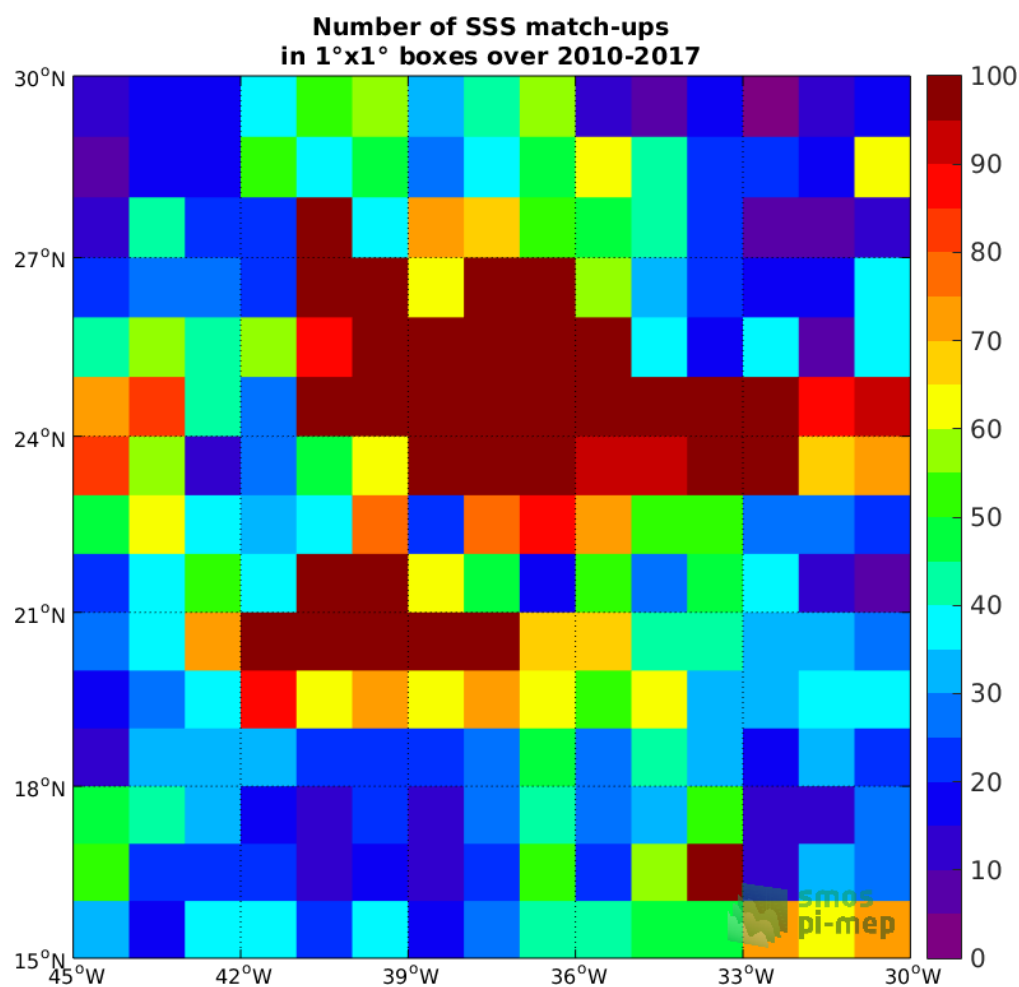
Figure 4: Number of SSS match-ups between Argo SSS and the SMOS-L3-CATDS-CECOS-LOCEAN-V3-9DAYS-25KM SSS product for the SPURS 1 Pi-MEP region over 1°x1° boxes and for the full satellite product period.
