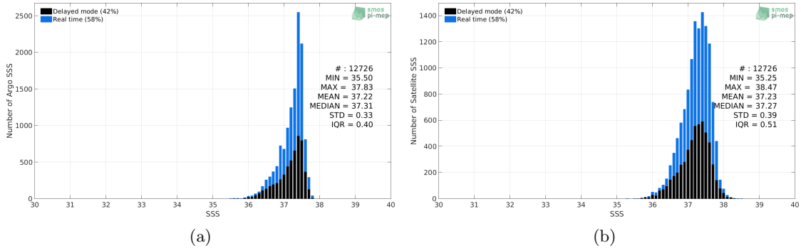
Figure 2: Histograms of SSS from Argo (a) and SMOS-L3-CATDS-CECOS-LOCEAN-V3-9DAYS-25KM (b) considering all match-up pairs per bins of 0.1 over the SPURS 1 Pi-MEP region and for the full satellite product period.
