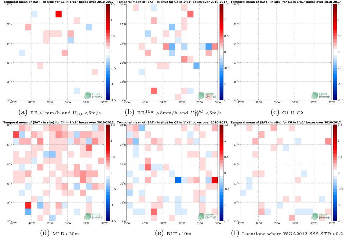
Figure 12: Temporal mean gridded over spatial boxes of size 1^\circ \times 1^\circ of \Delta\text{SSS} (SMOS-L3-CATDS-CECOS-LOCEAN-V3-9DAYS-25KM - Argo) for 6 different subdatasets corresponding to: \text{RR} > 1\text{mm/h} and U_{10} < 5\text{m/s} (a), \text{RR}^{10d} > 5\text{mm/h} and U_{10}^{10d} < 5\text{m/s} (b), C1 U C2 (c), \text{MLD} < 20\text{m} (d), \text{BLT} > 10\text{m} (e), Locations where WOA2013 SSS STD > 0.2 (f).
