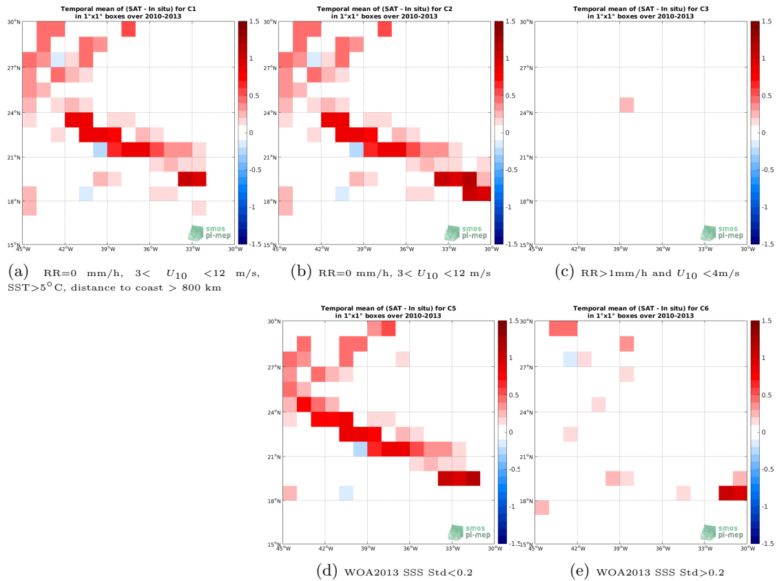
Figure 12: Temporal mean gridded over spatial boxes of size 1^\circ \times 1^\circ of \Delta SSS (SMOS-L3-CATDS-CECOS-LOCEAN-V3-18DAYS-25KM - TSG-SAMOS) for 5 different subdatasets corresponding to:RR=0 mm/h, 3 < U_{10} < 12 m/s, SST >5^\circ C, distance to coast > 800 km (a), RR=0 mm/h, 3 < U_{10} < 12 m/s (b), RR >1 mm/h and U_{10} < 4 m/s (c), WOA2013 SSS Std <0.2 (d), WOA2013 SSS Std >0.2 (e).
