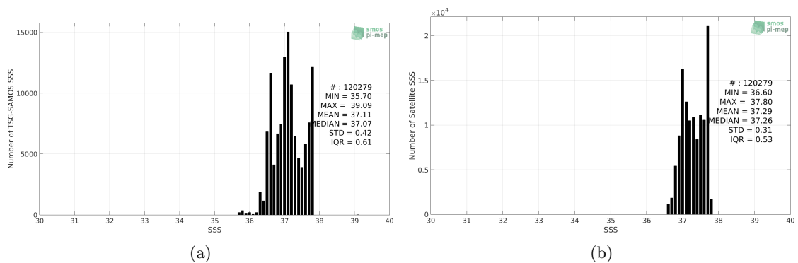
Figure 2: Histograms of SSS from TSG-SAMOS (a) and SMOS-L3-CATDS-CECOS-LOCEAN-V3-18DAYS-25KM (b) considering all match-up pairs per bins of 0.1 over the SPURS 1 Pi-MEP region and for the full satellite product period.
