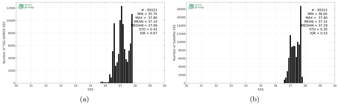
Figure 2: Histograms of SSS from TSG-SAMOS (a) and SMOS-L3-CATDS-CECOS-LOCEAN-V3-18DAYS-25KM (b) considering all match-up pairs per bins of 0.1 over the SPURS 1 Pi-MEP region and for the full satellite product period.
