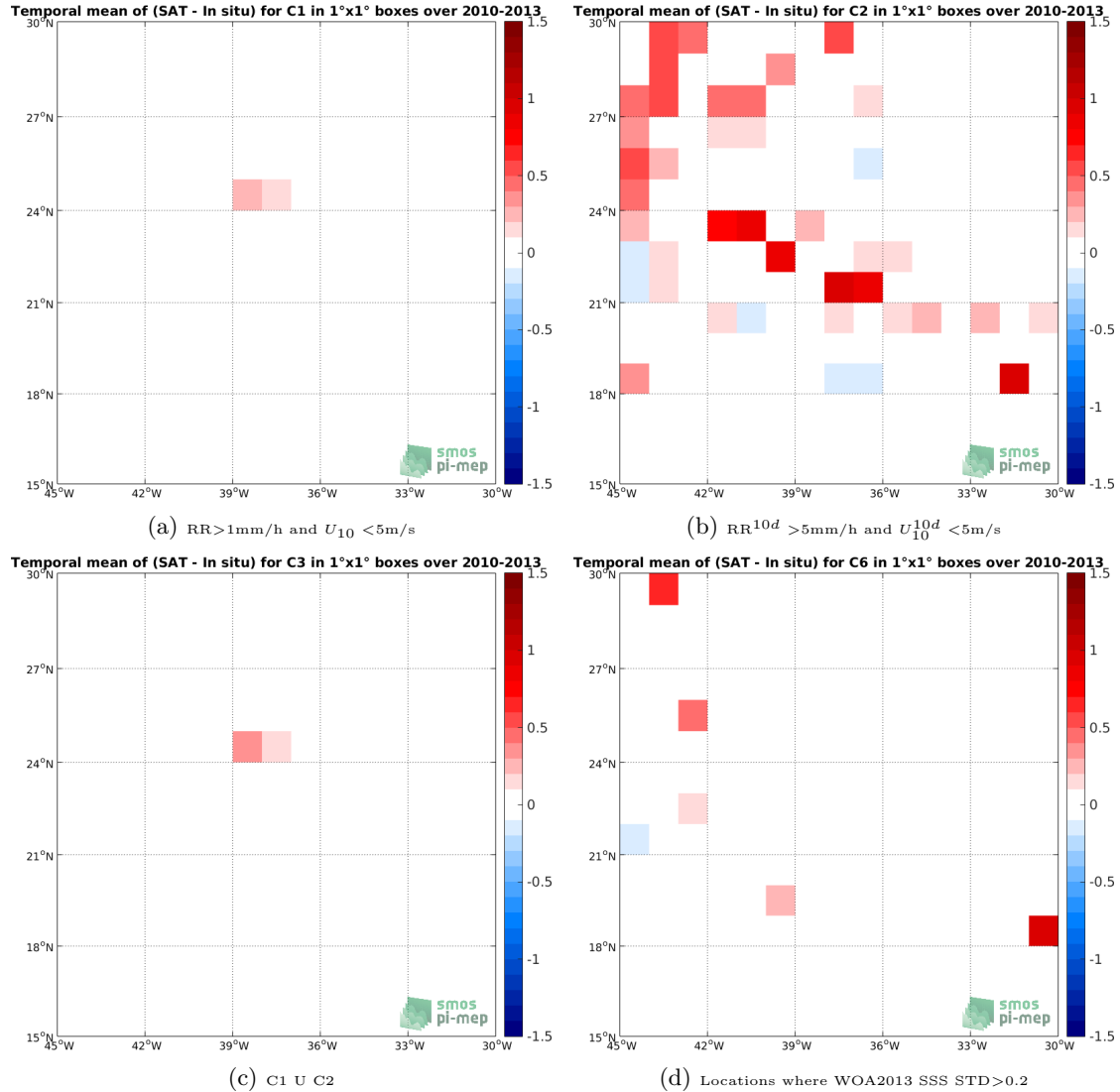
Figure 12: Temporal mean gridded over spatial boxes of size 1^\circ \times 1^\circ of \Delta SSS (SMOS-L3-CATDS-CECOS-LOCEAN-V3-18DAYS-25KM - TSG-SAMOS) for 4 different subdatasets corresponding to: RR > 1\text{mm/h} and U_{10} < 5\text{m/s} (a), RR^{10d} > 5\text{mm/h} and U_{10}^{10d} < 5\text{m/s} (b), C1 U C2 (c), Locations where WOA2013 SSS STD > 0.2 (d).
