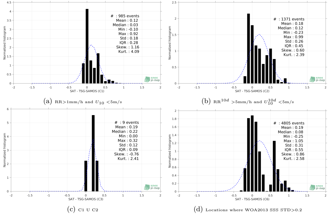
Figure 13: Normalized histogram of \Delta\text{SSS} (SMOS-L3-CATDS-CECOS-LOCEAN-V3-18DAYS-25KM - TSG-SAMOS) for 6 different subdatasets corresponding to: RR > 1\text{mm/h} and U_{10} < 5\text{m/s} (a), RR^{10d} > 5\text{mm/h} and U_{10}^{10d} < 5\text{m/s} (b), C1 U C2 (c), Locations where WOA2013 SSS STD > 0.2 (d).
