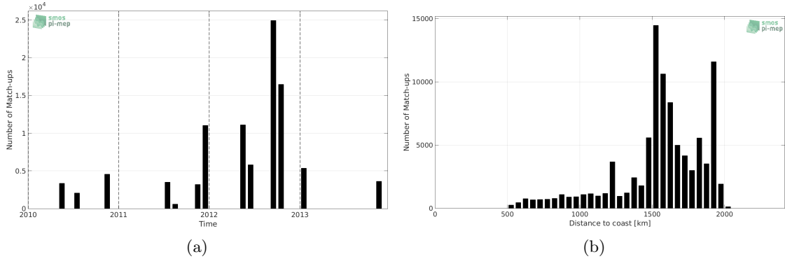
Figure 1: Number of match-ups between TSG-SAMOS and SMOS-L3-CATDS-CECOS-LOCEAN-V3-18DAYS-25KM SSS as a function of time (a) and as function of the distance to coast (b) over the SPURS 1 Pi-MEP region and for the full satellite product period.
