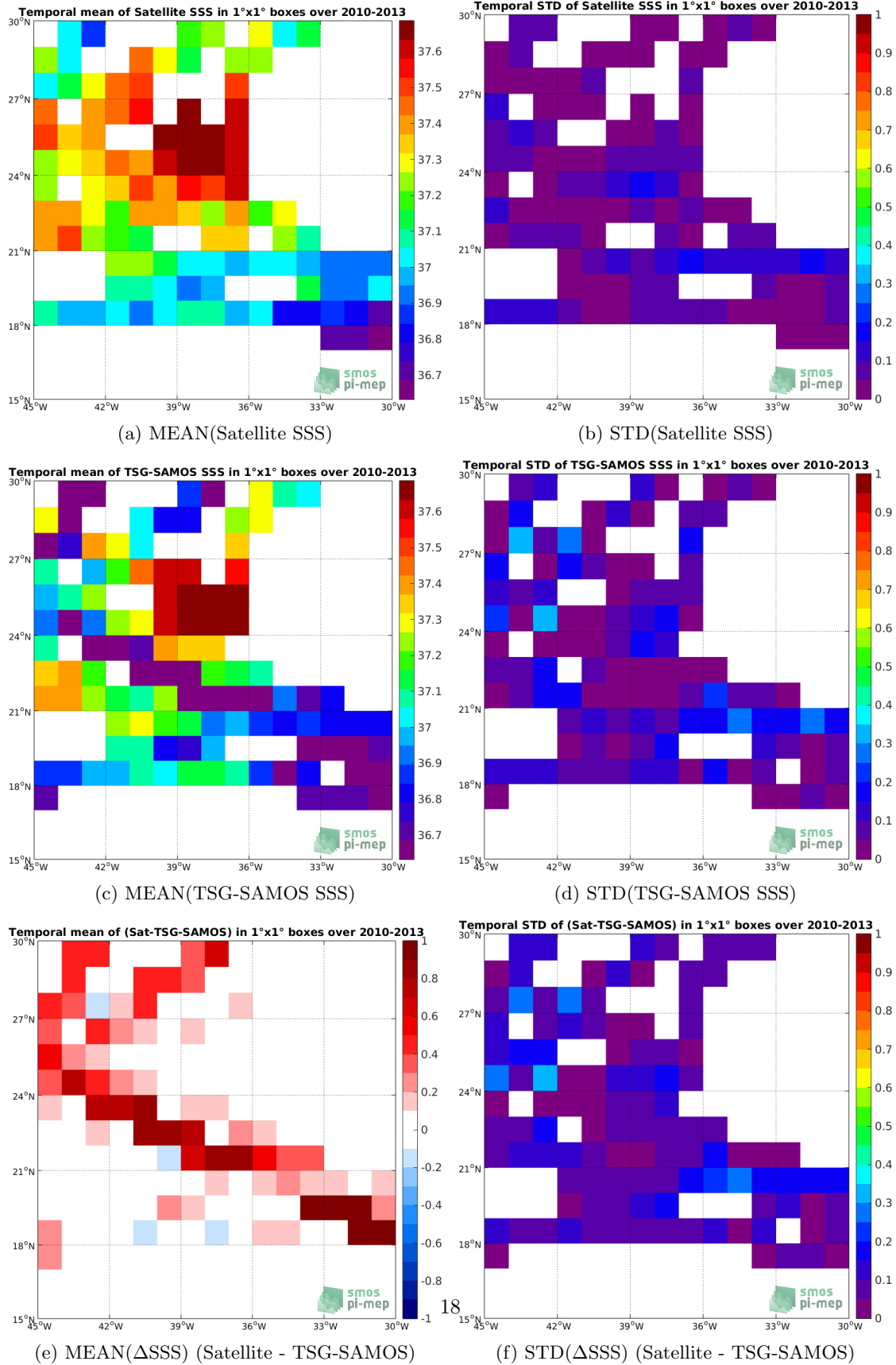
Figure 6: Temporal mean (left) and STD (right) of SSS from SMOS-L3-CATDS-CECOS-LOCEAN-V3-18DAYS-25KM (top), TSG-SAMOS (middle), and of \Delta SSS (Satellite - TSG-SAMOS). Only match-up pairs are used to generate these maps.
