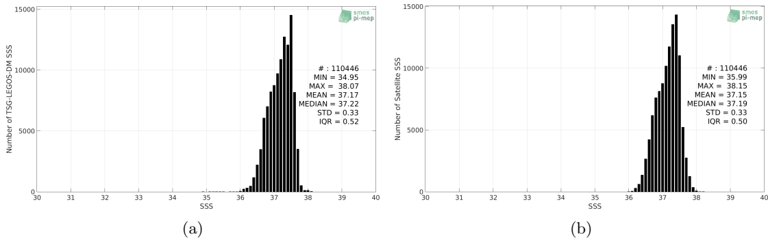
Figure 2: Histograms of SSS from TSG-LEGOS-DM (a) and SMOS-L3-CATDS-CECOS-LOCEAN-V3-18DAYS-25KM (b) considering all match-up pairs per bins of 0.1 over the SPURS 1 Pi-MEP region and for the full satellite product period.
