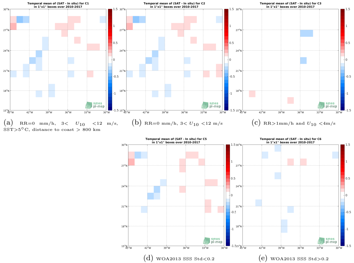
Figure 12: Temporal mean gridded over spatial boxes of size 1^\circ \times 1^\circ of \Delta SSS (SMOS-L3-CATDS-CECOS-LOCEAN-V3-18DAYS-25KM - TSG-LEGOS-DM) for 5 different subdatasets corresponding to:RR=0 mm/h, 3 < U_{10} < 12 m/s, SST >5^\circ C, distance to coast > 800 km (a), RR=0 mm/h, 3 < U_{10} < 12 m/s (b), RR >1 mm/h and U_{10} < 4 m/s (c), WOA2013 SSS Std <0.2 (d), WOA2013 SSS Std >0.2 (e).
