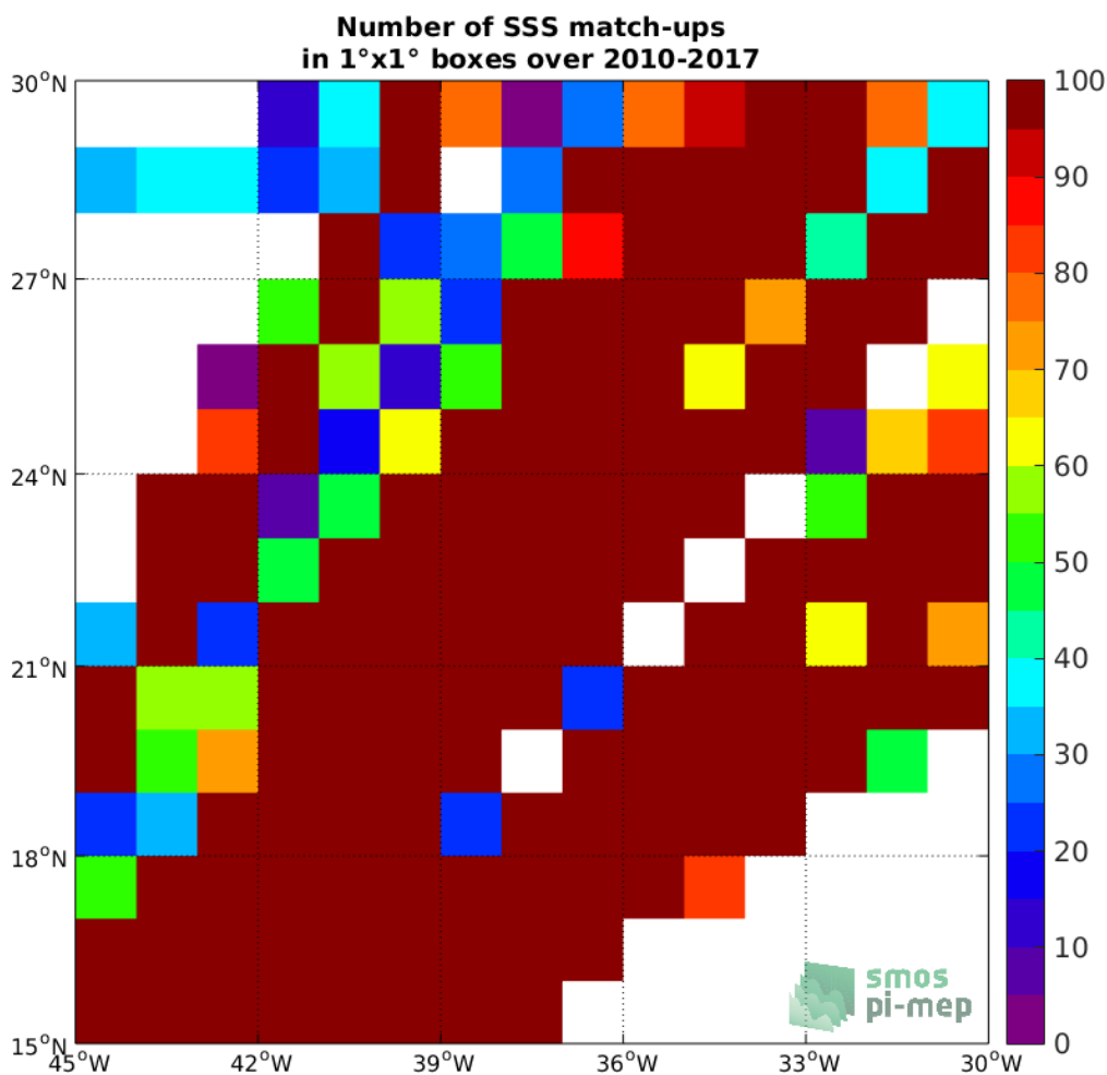
Figure 4: Number of SSS match-ups between TSG-LEGOS-DM SSS and the SMOS-L3-CATDS-CECOS-LOCEAN-V3-18DAYS-25KM SSS product for the SPURS 1 Pi-MEP region over 1°x1° boxes and for the full satellite product period.
