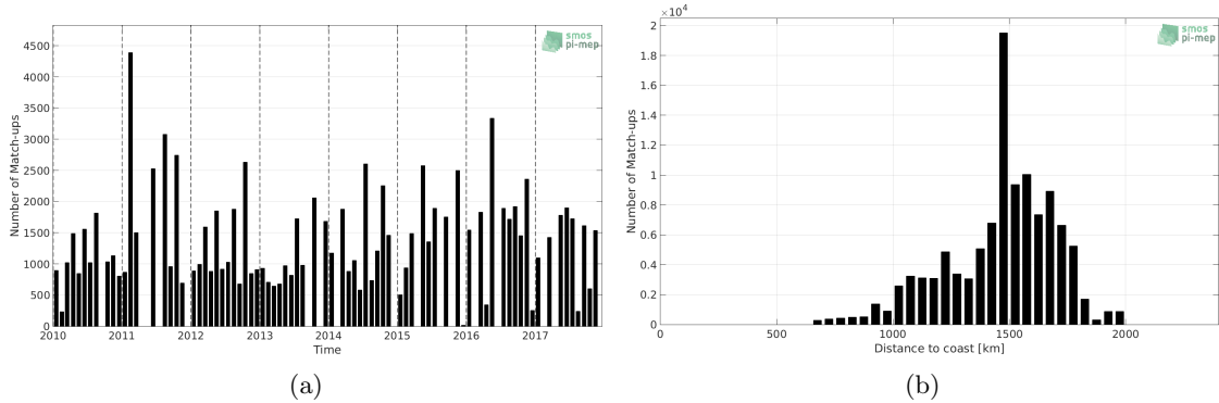
Figure 1: Number of match-ups between TSG-LEGOS-DM and SMOS-L3-CATDS-CECOS-LOCEAN-V3-18DAYS-25KM SSS as a function of time (a) and as function of the distance to coast (b) over the SPURS 1 Pi-MEP region and for the full satellite product period.
