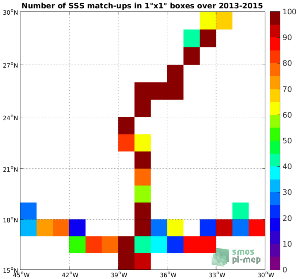
Figure 4: Number of SSS match-ups between TSG-GOSUD-Sailing-ship SSS and the SMOS-L3-CATDS-CECOS-LOCEAN-V3-18DAYS-25KM SSS product for the SPURS 1 Pi-MEP region over 1°x1° boxes and for the full satellite product period.
