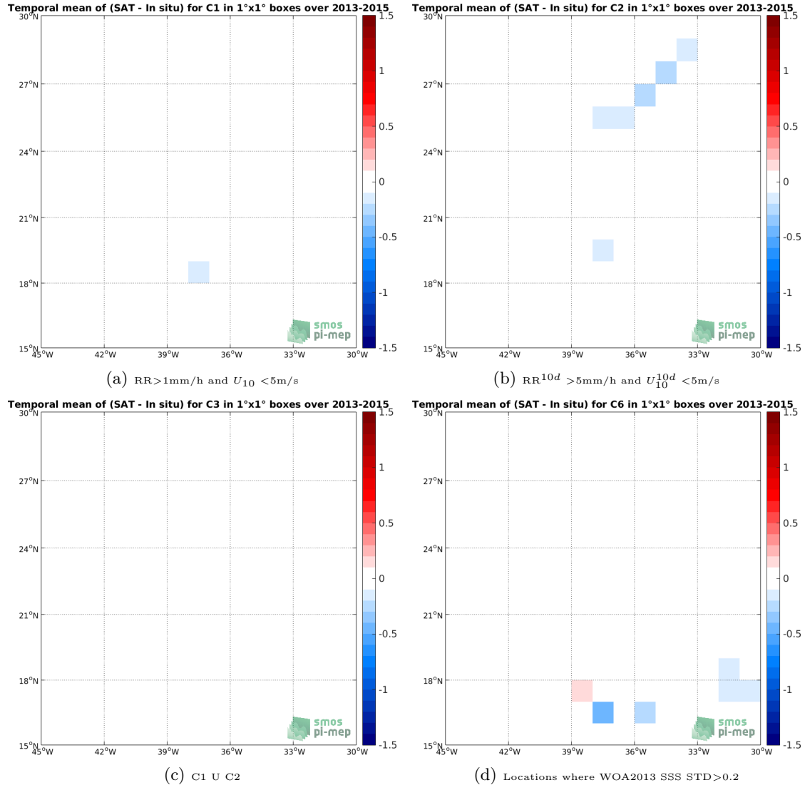
Figure 12: Temporal mean gridded over spatial boxes of size 1^\circ \times 1^\circ of \Delta SSS (SMOS-L3-CATDS-CECOS-LOCEAN-V3-18DAYS-25KM - TSG-GOSUD-Sailing-ship) for 4 different subdatasets corresponding to:RR >1 mm/h and U_{10} < 5 m/s (a), RR^{10d} > 5 mm/h and U_{10}^{10d} < 5 m/s (b), C1 U C2 (c),Locations where WOA2013 SSS STD >0.2 (d).
