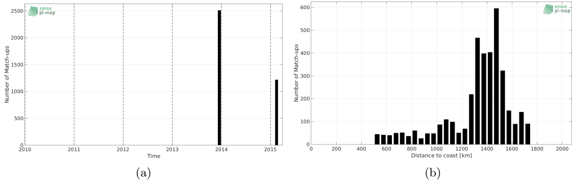
Figure 1: Number of match-ups between TSG-GOSUD-Sailing-ship and SMOS-L3-CATDS-CECOS-LOCEAN-V3-18DAYS-25KM SSS as a function of time (a) and as function of the distance to coast (b) over the SPURS 1 Pi-MEP region and for the full satellite product period.
