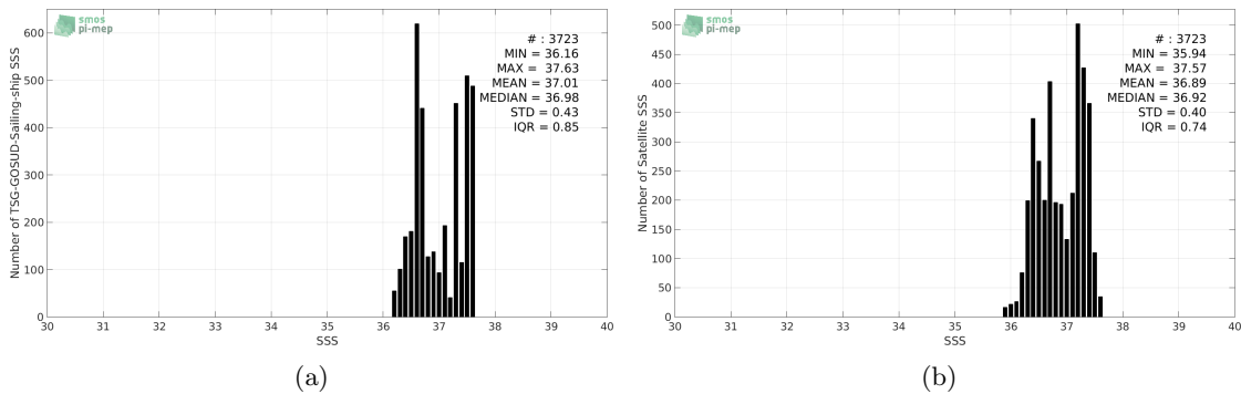
Figure 2: Histograms of SSS from TSG-GOSUD-Sailing-ship (a) and SMOS-L3-CATDS-CECOS-LOCEAN-V3-18DAYS-25KM (b) considering all match-up pairs per bins of 0.1 over the SPURS 1 Pi-MEP region and for the full satellite product period.
