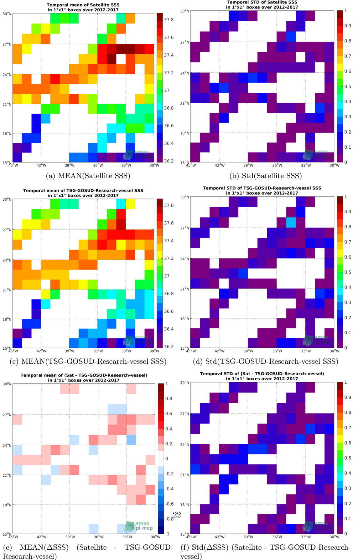
Figure 6: Temporal mean (left) and Std (right) of SSS from SMOS-L3-CATDS-CECOS-LOCEAN-V3-18DAYS-25KM (top), TSG-GOSUD-Research-vessel (middle), and of \Delta SSS (Satellite - TSG-GOSUD-Research-vessel). Only match-up pairs are used to generate these maps.
