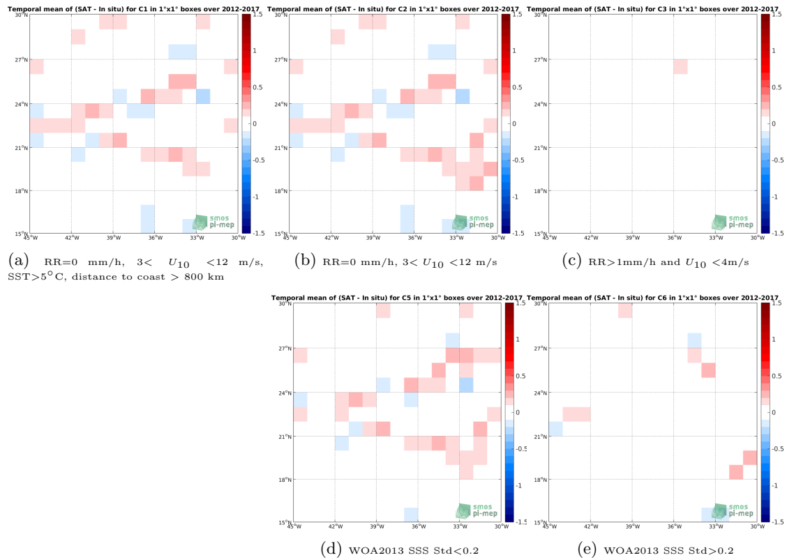
Figure 12: Temporal mean gridded over spatial boxes of size 1^\circ \times 1^\circ of \Delta SSS (SMOS-L3-CATDS-CECOS-LOCEAN-V3-18DAYS-25KM - TSG-GOSUD-Research-vessel) for 5 different subdatasets corresponding to:RR=0 mm/h, 3 < U_{10} < 12 m/s, SST >5^\circ\text{C} , distance to coast > 800 km (a), RR=0 mm/h, 3 < U_{10} < 12 m/s (b), RR >1 mm/h and U_{10} < 4 m/s (c), WOA2013 SSS Std <0.2 (d), WOA2013 SSS Std >0.2 (e).
