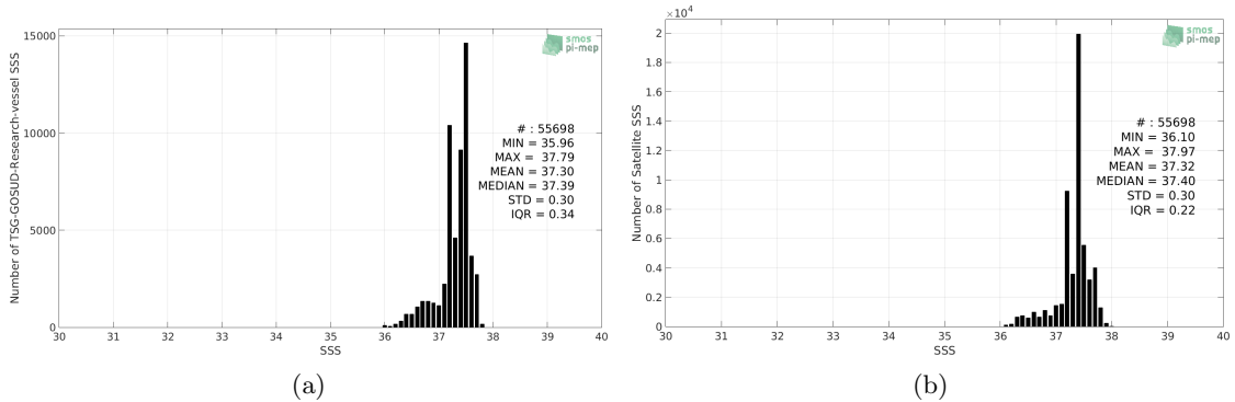
Figure 2: Histograms of SSS from TSG-GOSUD-Research-vessel (a) and SMOS-L3-CATDS-CECOS-LOCEAN-V3-18DAYS-25KM (b) considering all match-up pairs per bins of 0.1 over the SPURS 1 Pi-MEP region and for the full satellite product period.
