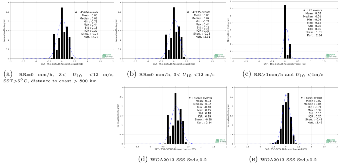
Figure 13: Normalized histogram of \Delta SSS (SMOS-L3-CATDS-CECOS-LOCEAN-V3-18DAYS-25KM - TSG-GOSUD-Research-vessel) for 5 different subdatasets corresponding to: RR=0 mm/h, 3 < U_{10} < 12 m/s, SST>5°C, distance to coast > 800 km (a), RR=0 mm/h, 3 < U_{10} < 12 m/s (b), RR>1mm/h and U_{10} < 4 m/s (c), WOA2013 SSS Std<0.2 (d), WOA2013 SSS Std>0.2 (e).
